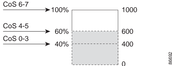
Figure 33-6 WTD and Queue Operation
