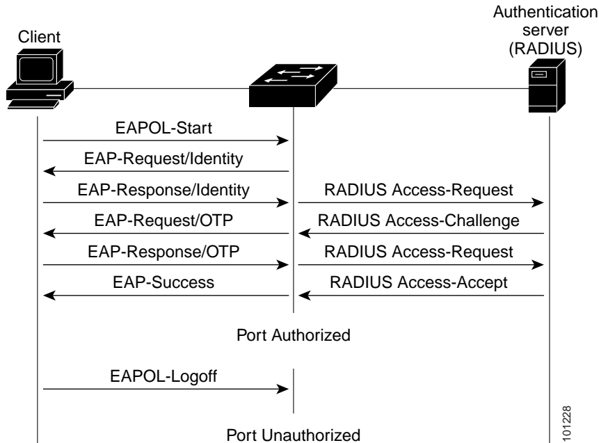
Figure 11-3 Message Exchange
