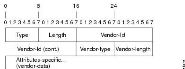
Figure 109: VSA Encapsulated Behind Attribute 26
