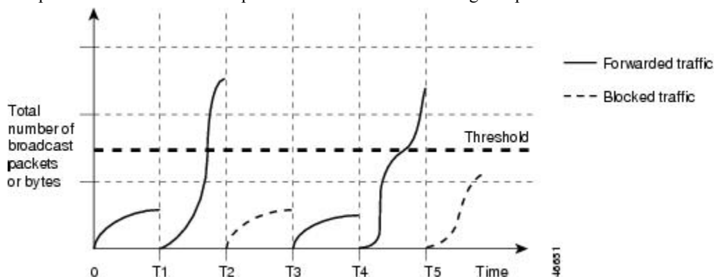
Figure 138: Broadcast Storm Control Example
