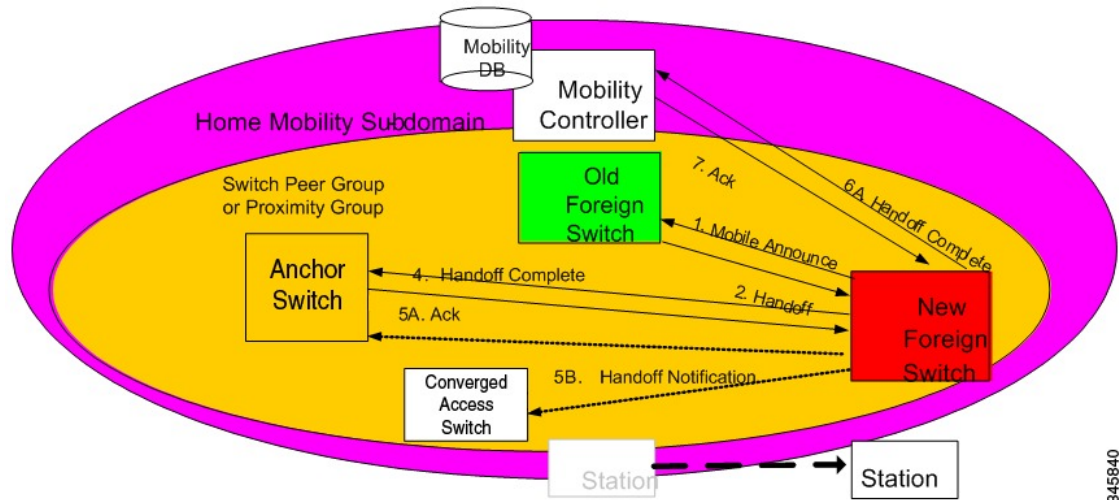
Figure 72: Intra Switch Peer Group Handoff
