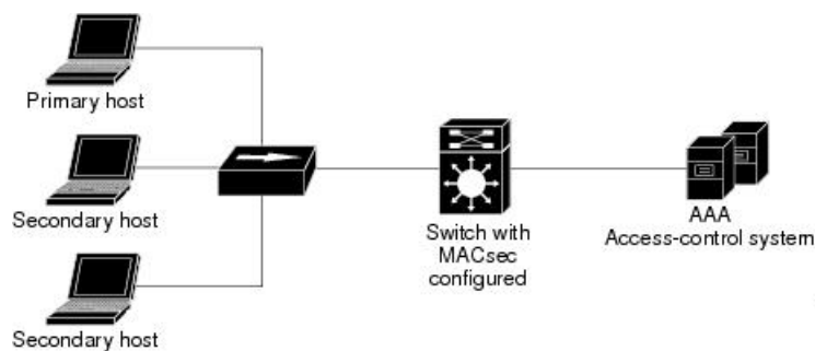
Figure 107: MACsec in Multiple-Host Mode - Unsecured
