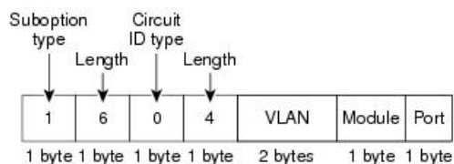
Figure 121: Suboption Packet Formats
