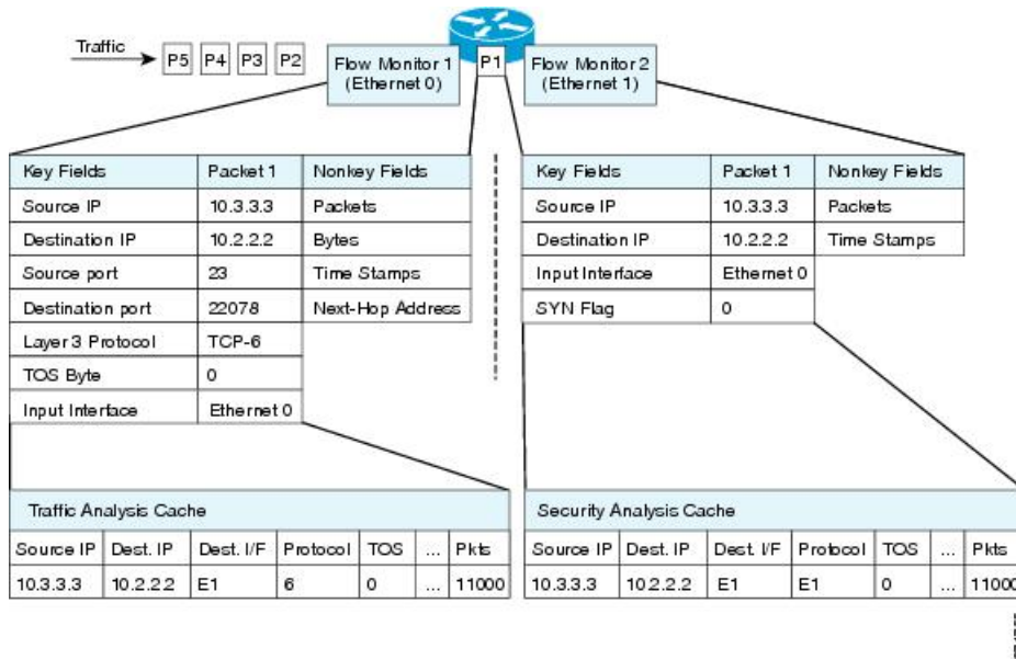
Figure 91: Example of Using Two Flow Monitors to Analyze the Same Traffic
