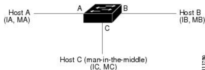
Figure 123: ARP Cache Poisoning
