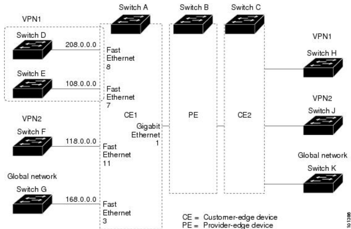
Figure 104: Multi-VRF CE Configuration Example
