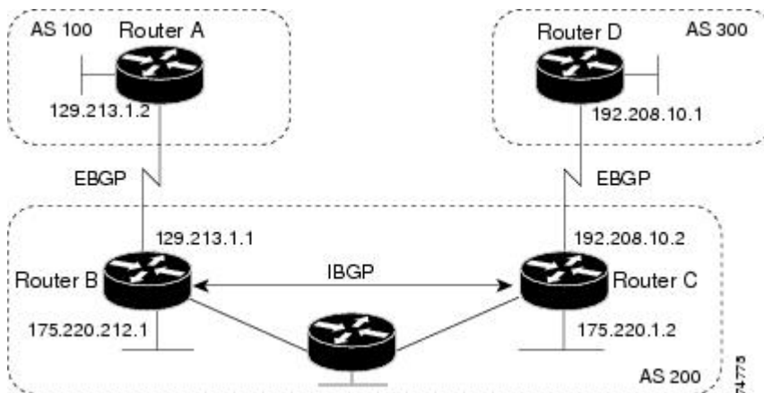
Figure 102: EBGP, IBGP, and Multiple Autonomous Systems
