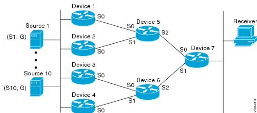
Figure 40: Polarization Topology
