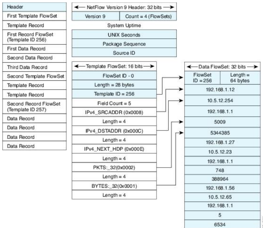
Figure 90: Detailed Example of the NetFlow Version 9 Export Format
