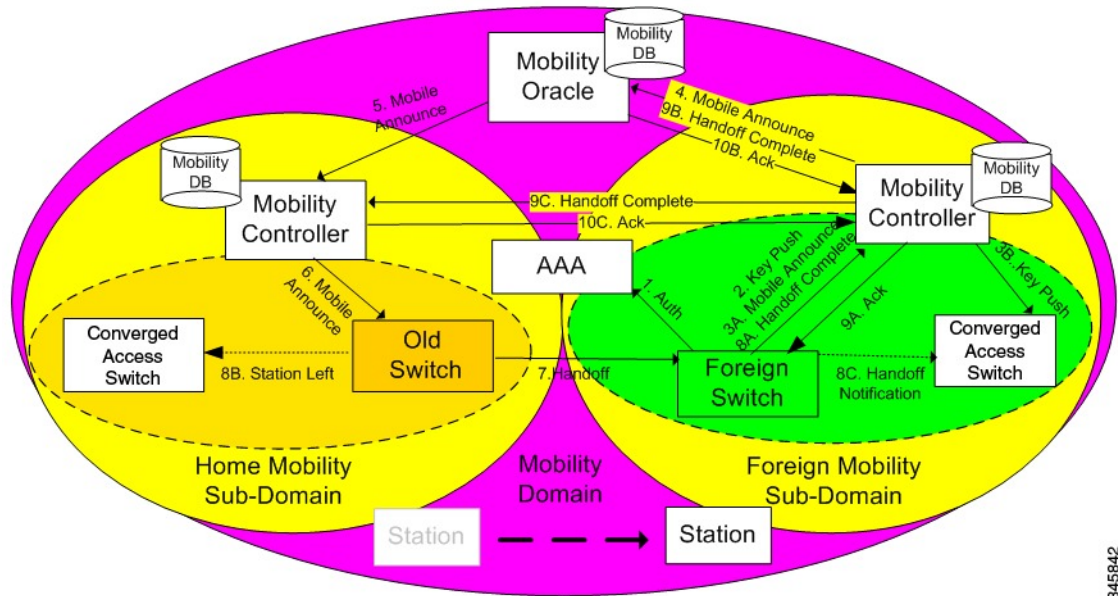
Figure 74: Inter Sub Domain Handoff
