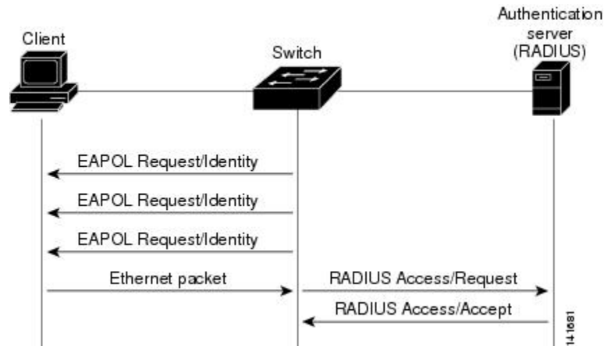
Figure 129: Message Exchange During MAC Authentication Bypass
