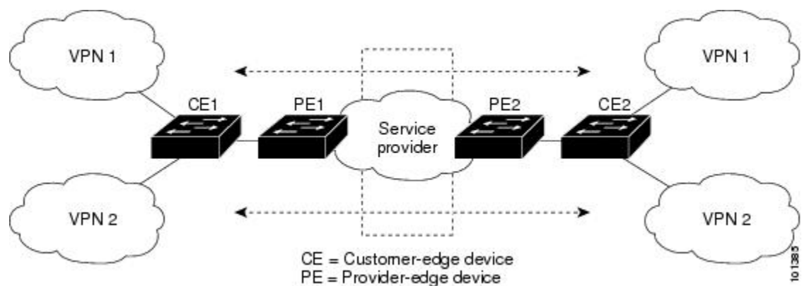
Figure 103: Switches Acting as Multiple Virtual CEs
