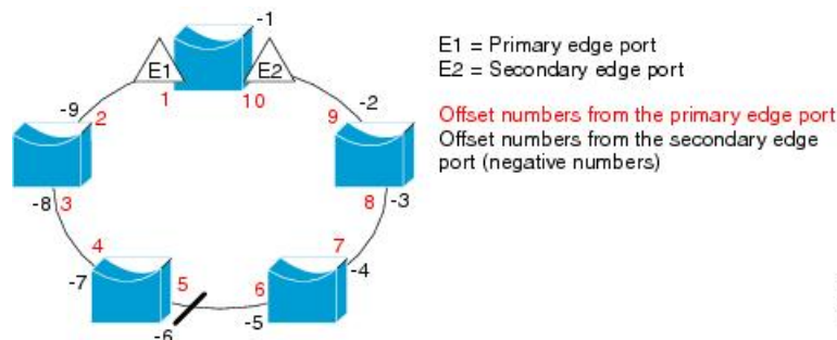
Figure 70: Neighbor Offset Numbers in a Segment
