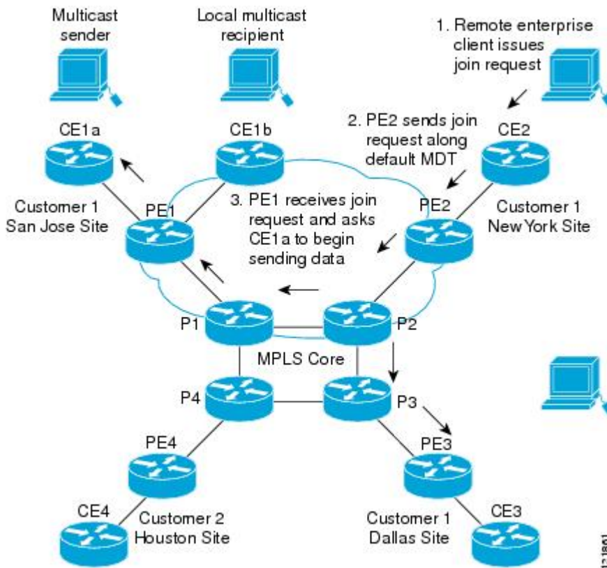
Figure 77: Initializing the Data MDT
