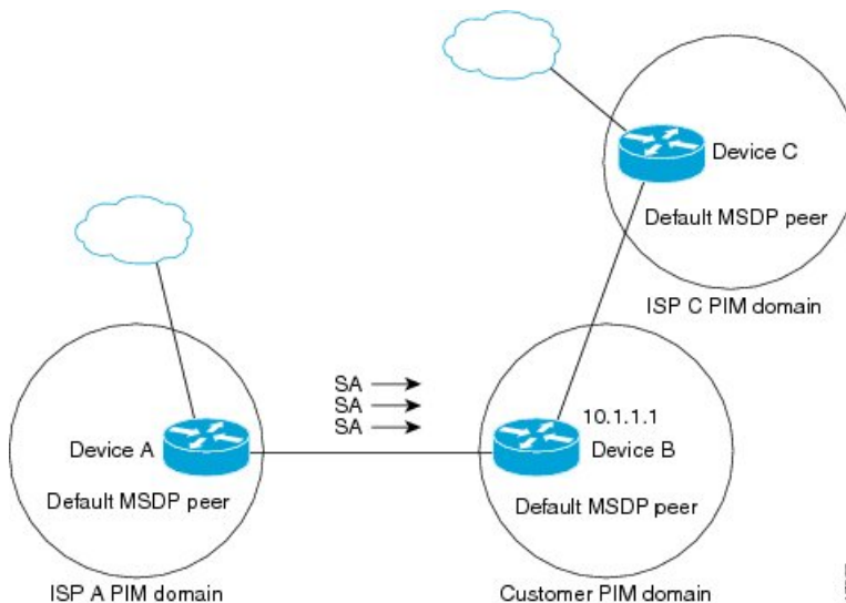
Figure 33: Default MSDP Peer Scenario
