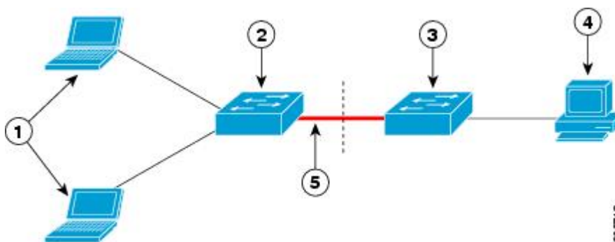
Figure 131: Authenticator and Supplicant Switch using CISP
