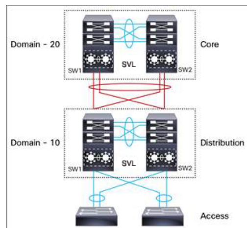
Figure 140: Typical Network Design using Cisco StackWise Virtual
