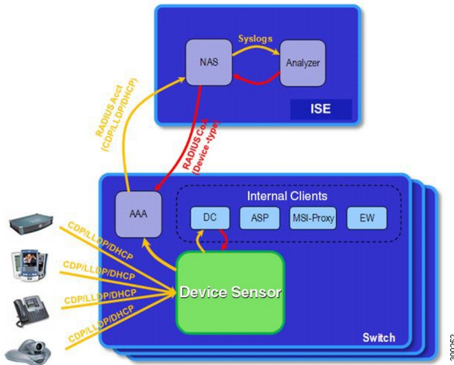
Figure 132: Device Sensor Clients
