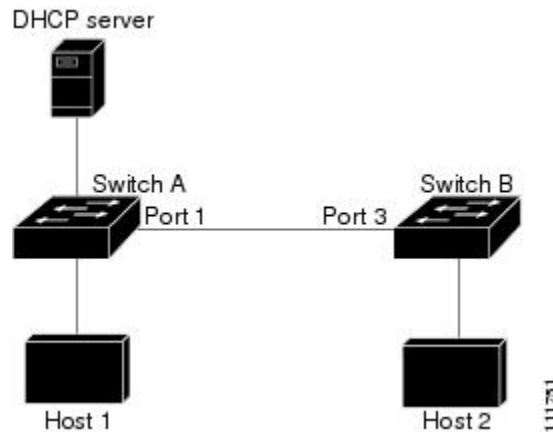
Figure 124: ARP Packet Validation on a VLAN Enabled for Dynamic ARP Inspection
