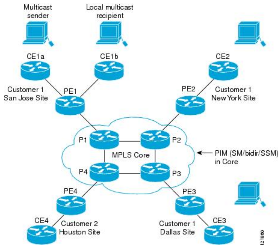
Figure 76: Default Multicast Distribution Tree Overview
