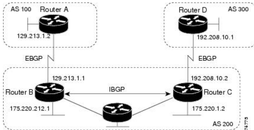
Figure 101: EBGP, IBGP, and Multiple Autonomous Systems
