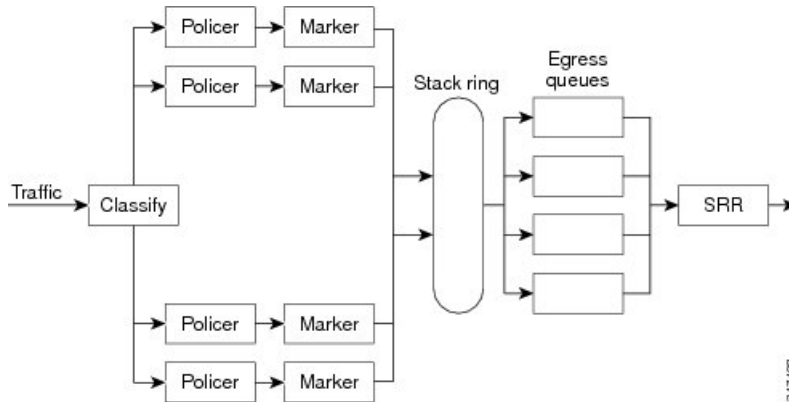
Figure 67: Egress Queue Location on Switch
