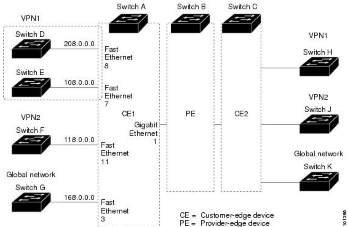
Figure 76: Multi-VRF CE Configuration Example
