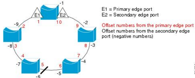
Figure 42: Neighbor Offset Numbers in a Segment
