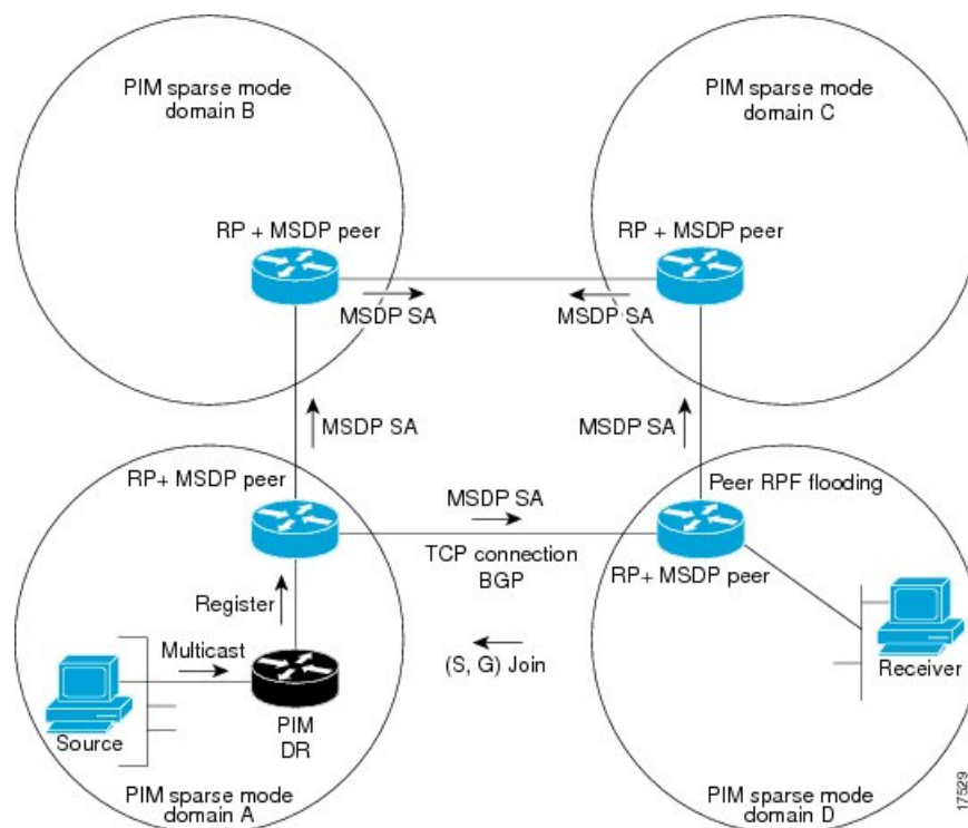
Figure 87: MSDP Running Between RP Peers
