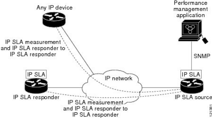
Figure 47: Cisco IOS IP SLAs Operation
