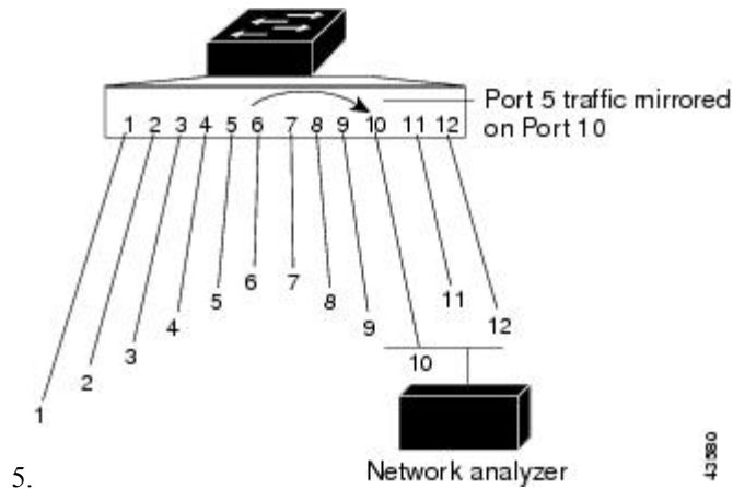
Figure 55: Example of Local SPAN Configuration on a Device Stack
