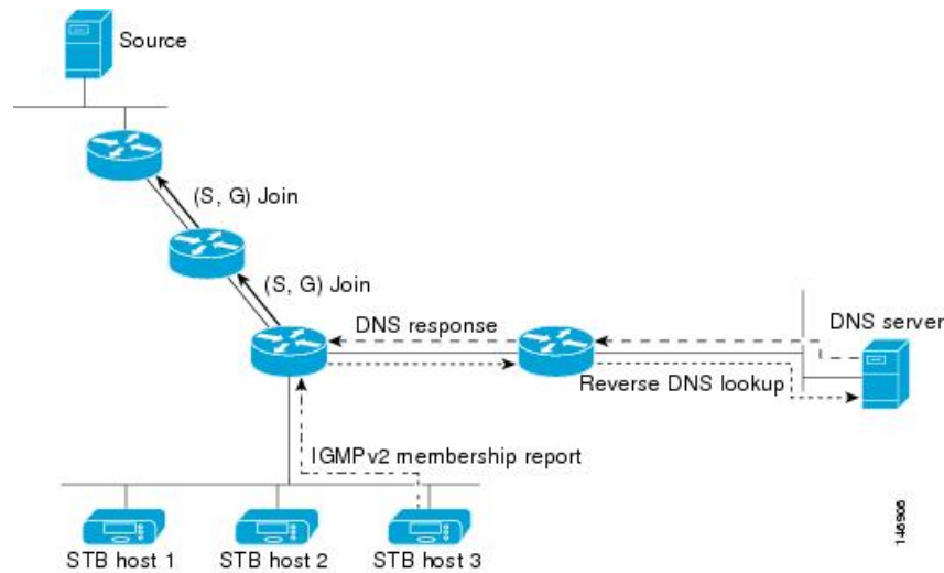
Figure 83: DNS-Based SSM-Mapping
