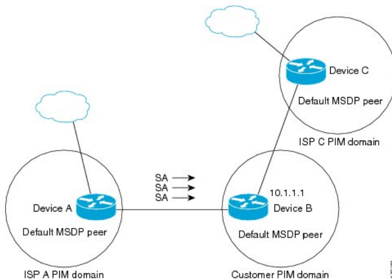
Figure 88: Default MSDP Peer Scenario
