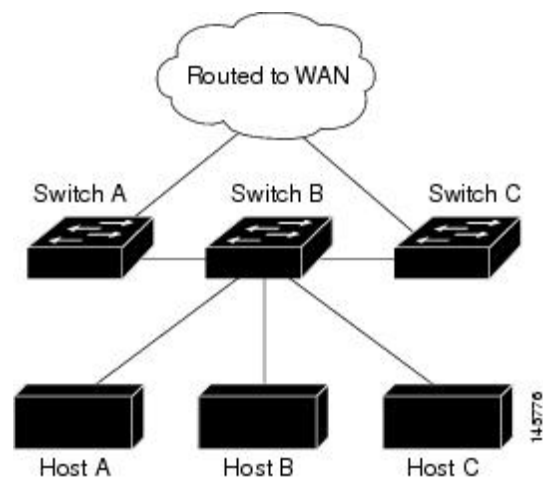
Figure 74: EIGRP Stub Router Configuration
