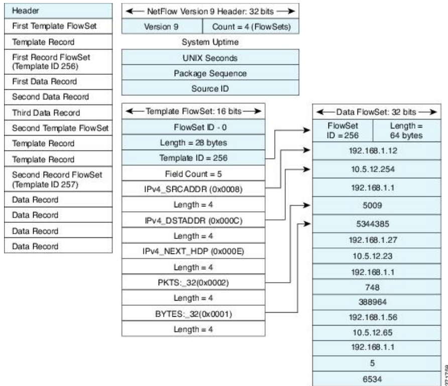
Figure 60: Detailed Example of the NetFlow Version 9 Export Format
