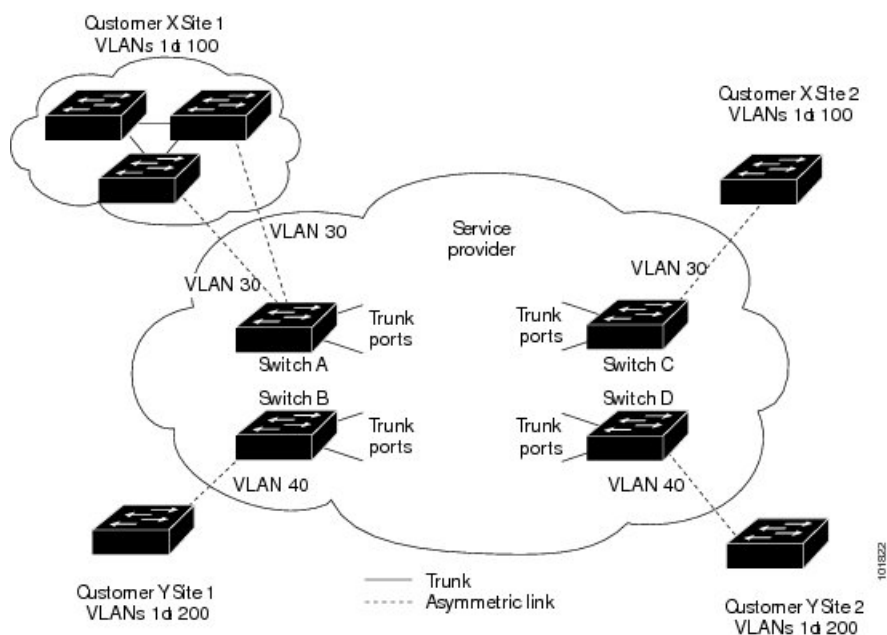
Figure 6: Layer 2 Protocol Tunneling
