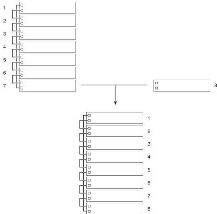
Figure 50: Adding a Standalone Switch to a Switch Stack
