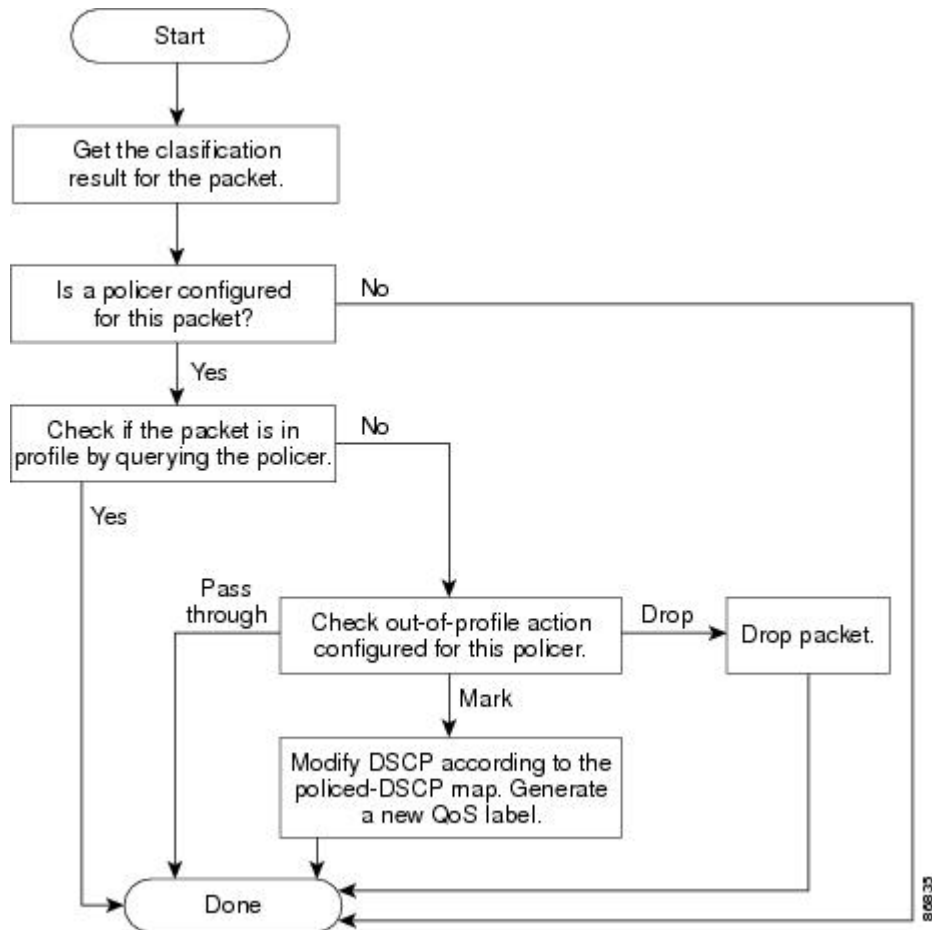
Figure 66: Policing and Marking Flowchart on Physical Ports
