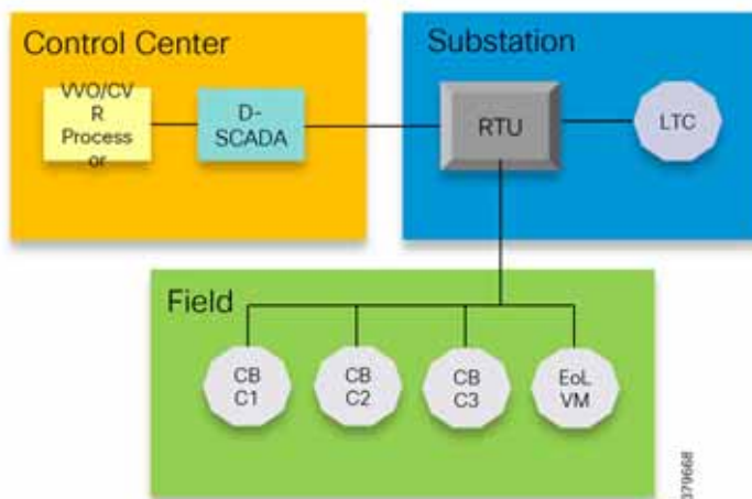
Figure 6 Volt/VAR Use Case Block Diagram
