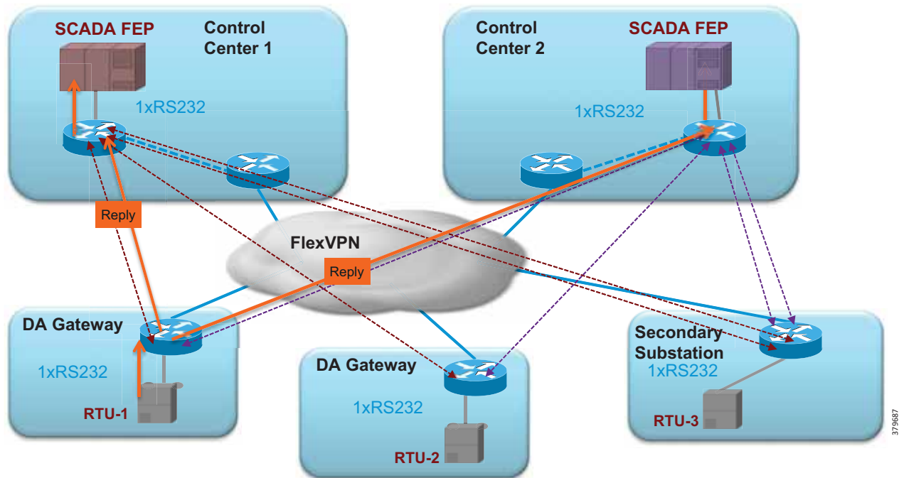
Figure 38 SCADA Multi-Drop Response
