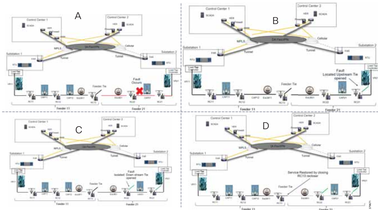
Figure 9 How FLISR Works
