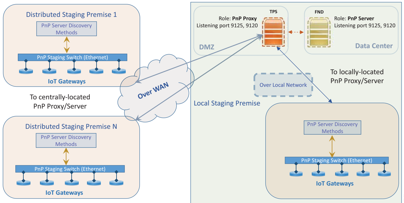
Figure 55 Bootstrapping of IoT Gateway at the Staging Premises (Local vs Distributed)
