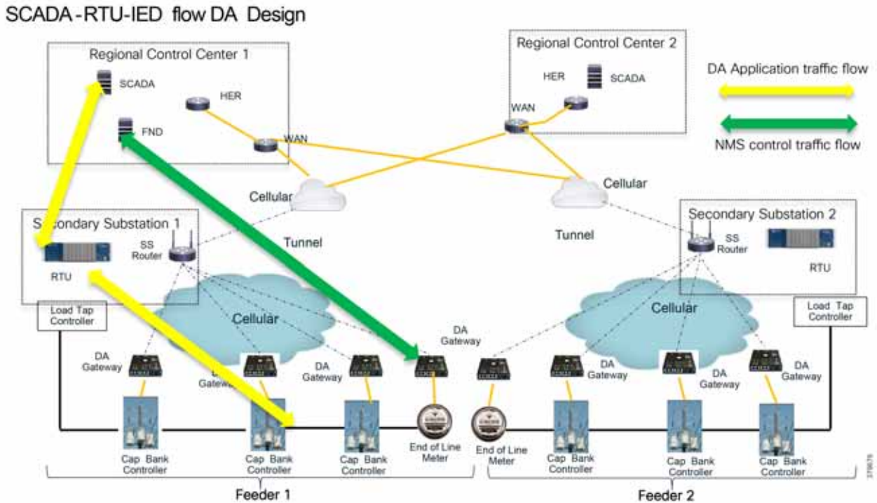
Figure 14 SCADA RTU IED Flow DA Design
