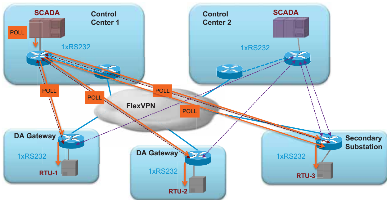
Figure 37 SCADA Multi-Drop Poll
