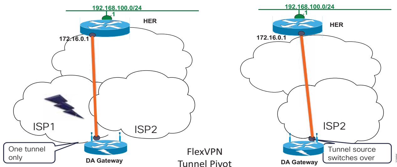
Figure 61 FlexVPN Tunnel Pivot
