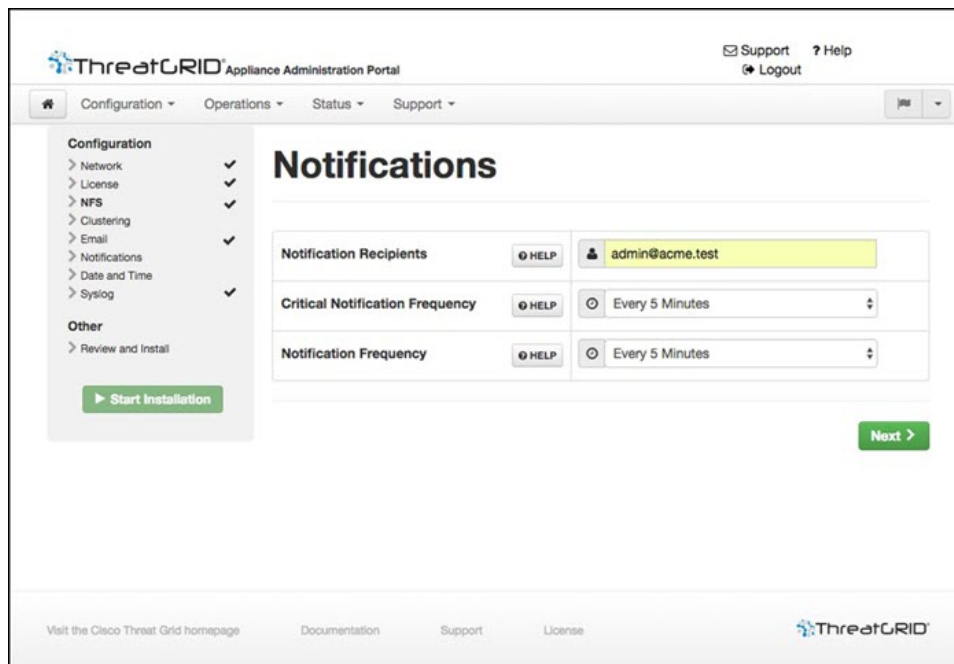
Figure 20: Notifications Configuration
