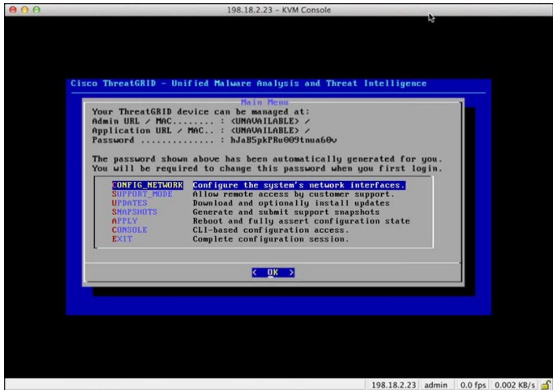
Figure 8: TGSN Dialog
