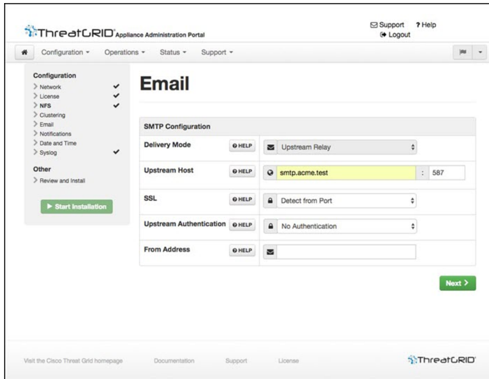
Figure 19: Email Configuration
