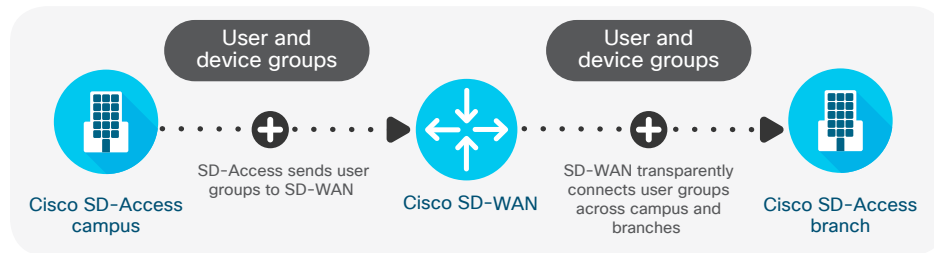
Figure 4. Cisco SD-Access and SD-WAN policy integration
