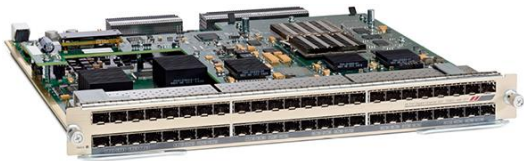
Figure 1. 48-Port Fiber Gigabit Ethernet Module
