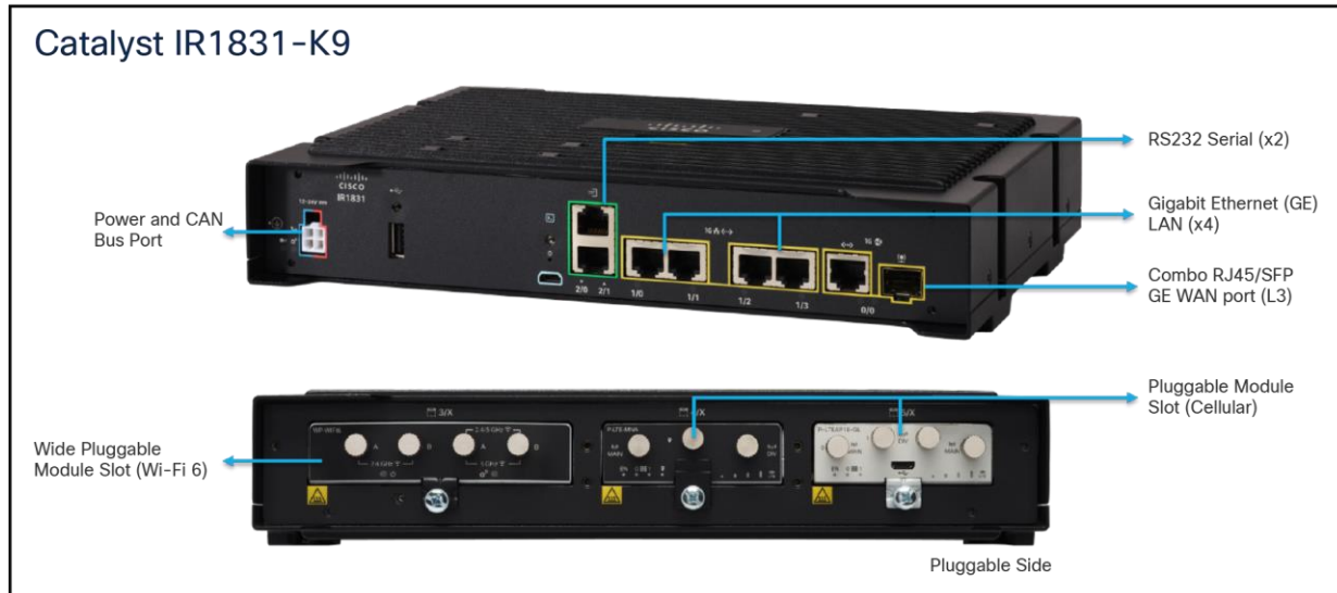
Figure 4. IR1831-K9 interface ports
