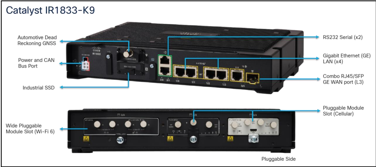
Figure 5. IR1833-K9 interface ports
