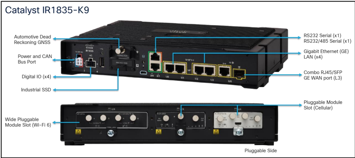
Figure 6. IR1835-K9 interface ports
