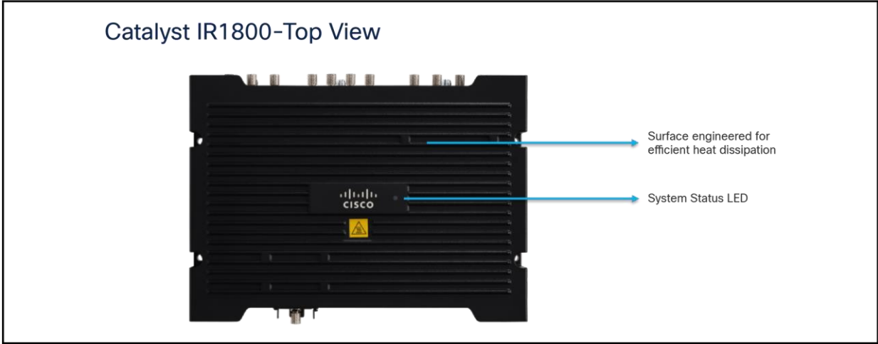
Figure 7. Top view
