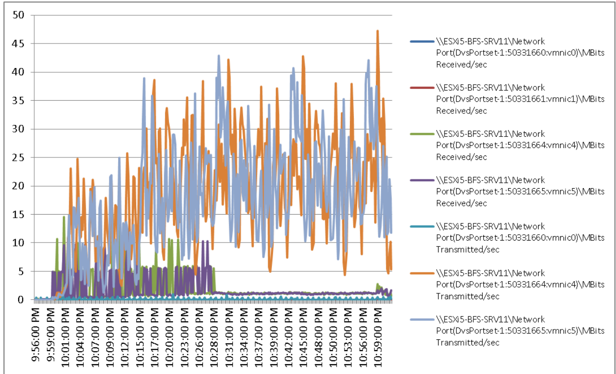
Figure 176 2000 User ESXi Host11 B200 M3 Cisco VIC1240 MLOM Network Adapter Mbps Receive/Transmit Test Phase
