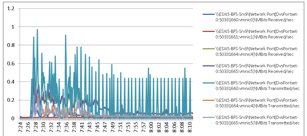
Figure 106 2000 User ESXi Host9 B200 M3 Cisco VIC1240 MLOM Network Adapter Mbps Receive/Transmit Boot Phase
