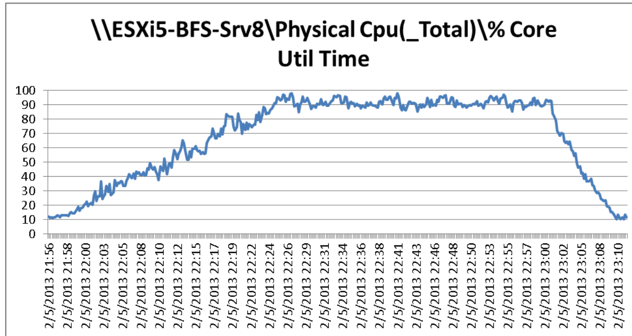
Figure 158 2000 User ESXi Host8 B200 M3 Processor Core Utilization Test Phase
