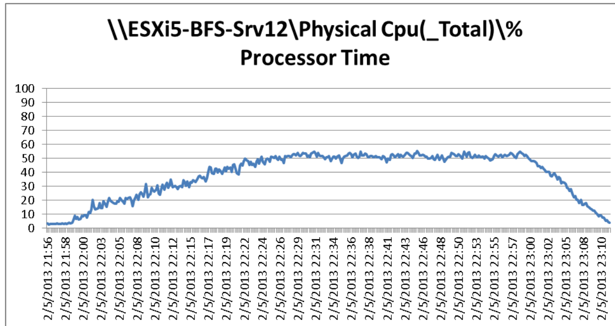
Figure 179 2000 User ESXi Host12 B200 M3 Processor Time Test Phase
