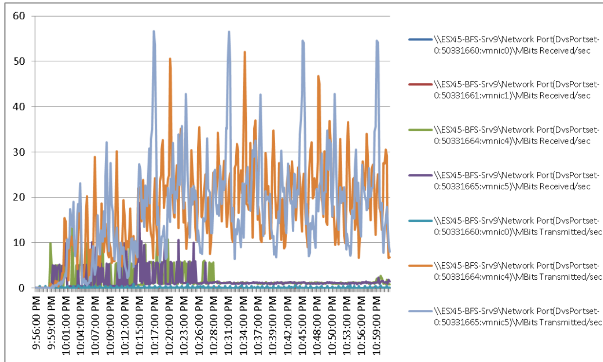
Figure 166 2000 User ESXi Host9 B200 M3 Cisco VIC1240 MLOM Network Adapter Mbps Receive/Transmit Test Phase
