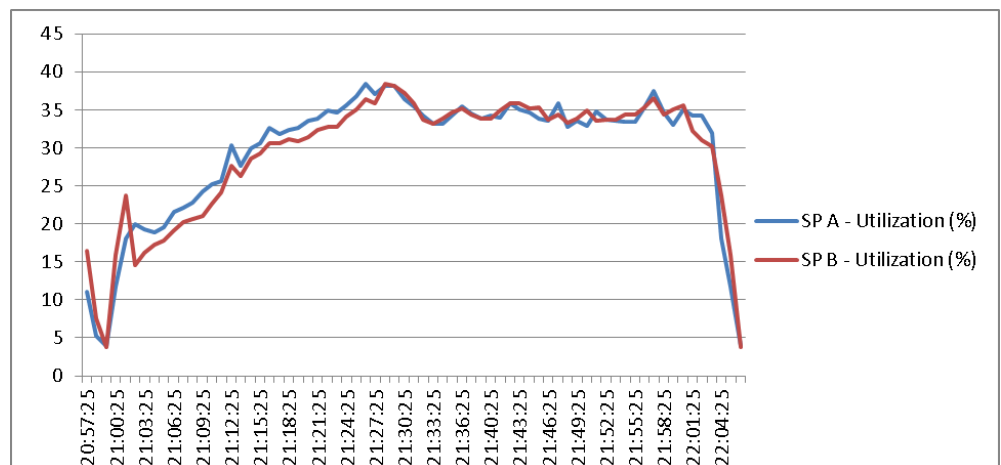
Figure 59 2000 Users EMC VNX5500 SP Utilization Test Phase
