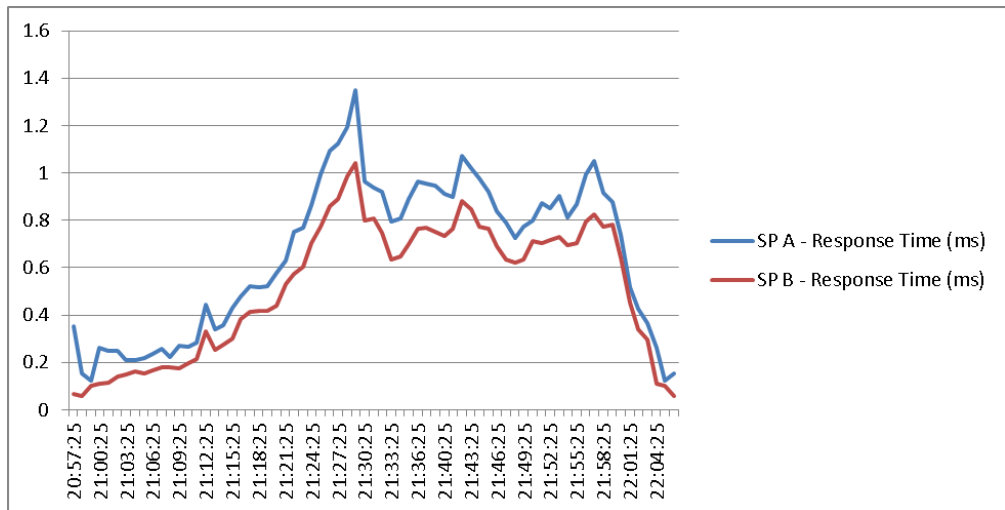
Figure 61 2000 Users EMC VNX5500 SP Response Time Test Phase
