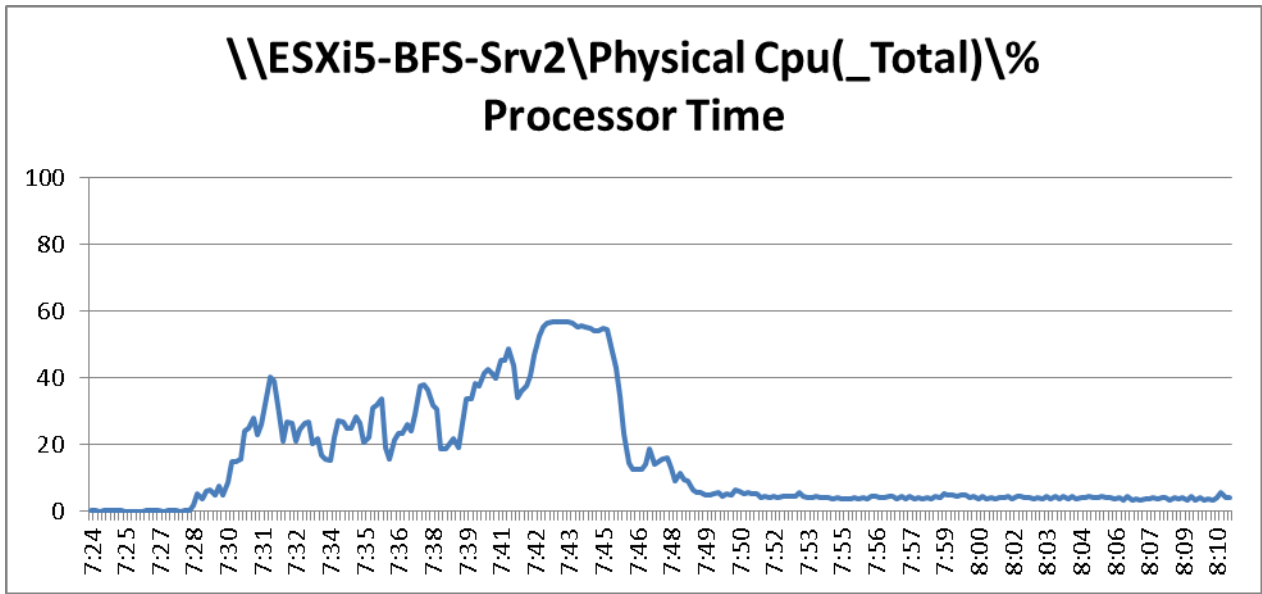
Figure 69 2000 User ESXi Host2 B200 M3 Processor Time Boot Phase
