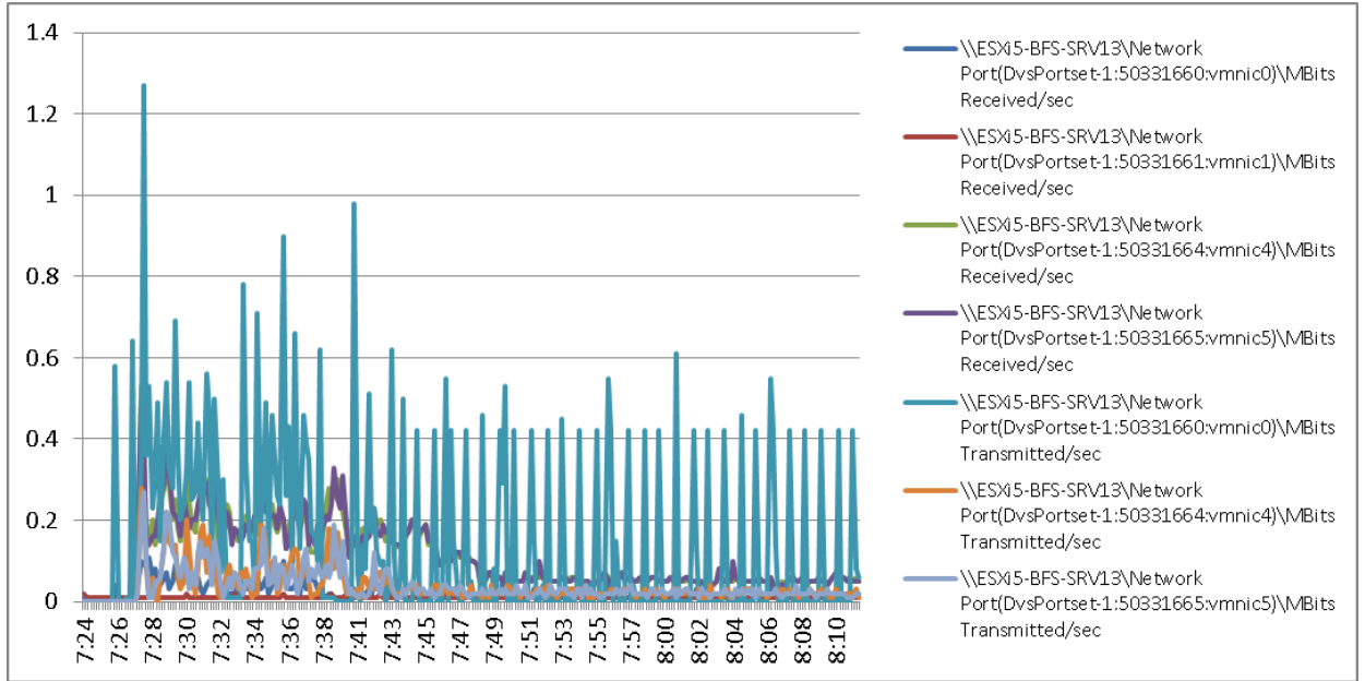
Figure 121 2000 User ESXi Host13 B200 M3 Cisco VIC1240 MLOM Network Adapter Mbps Receive/Transmit Boot Phase
