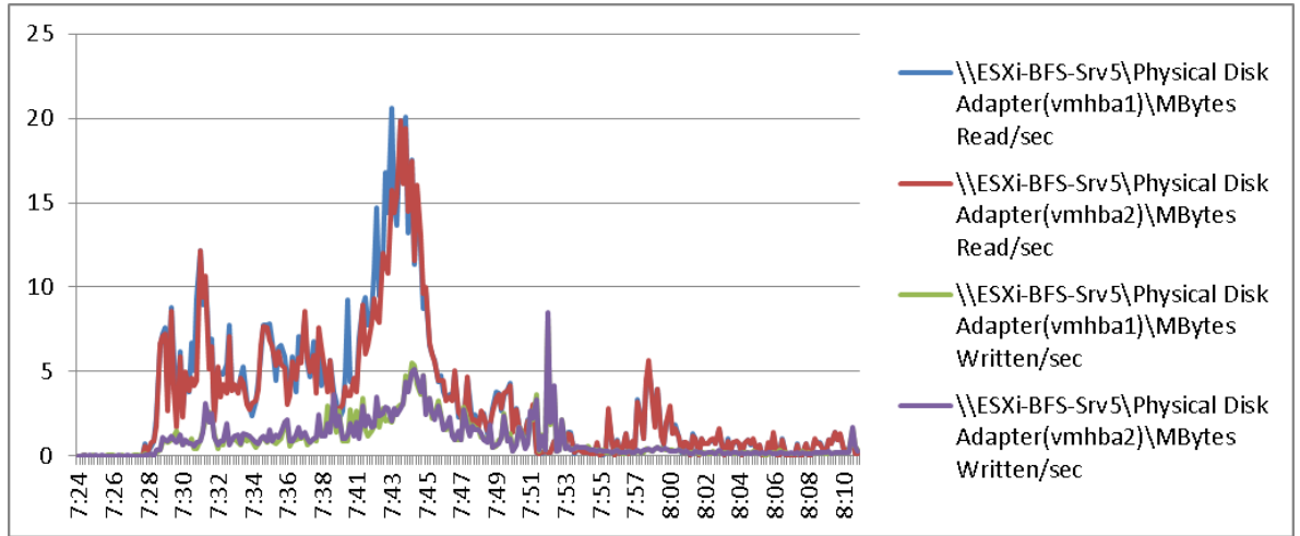
Figure 87 2000 User ESXi Host5 B200 M3 Cisco VIC1240 MLOM Physical Disk Adapter MBps Read/Write Boot Phase
