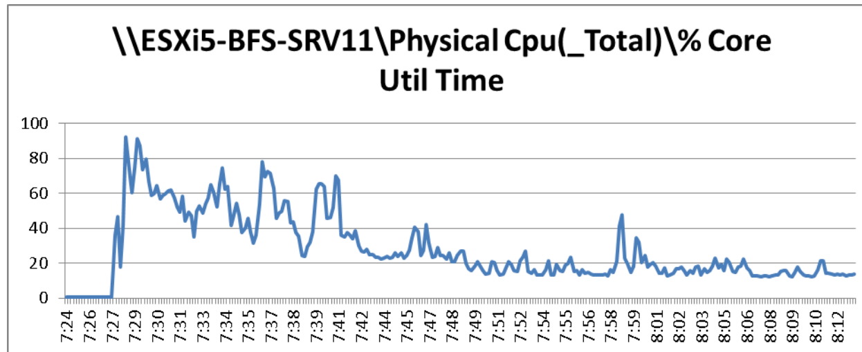
Figure 108 2000 User ESXi Host11 B200 M3 Processor Core Utilization Boot Phase
