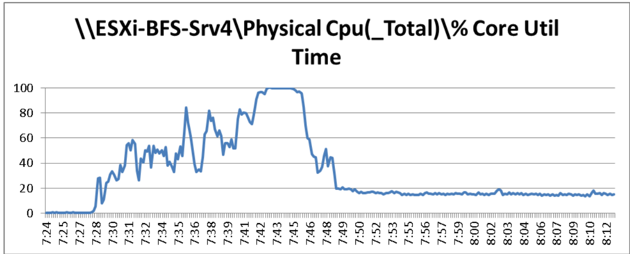
Figure 78 2000 User ESXi Host4 B200 M3 Processor Core Utilization Boot Phase
