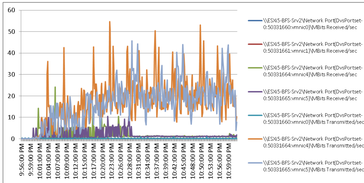
Figure 131 2000 User ESXi Host2 B200 M3 Cisco VIC1240 MLOM Network Adapter Mbps Receive/Transmit Test Phase
