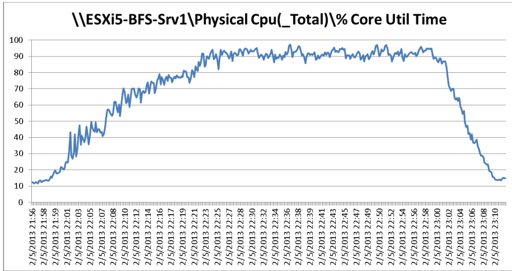
Figure 52 2000 User Single B200 M3 CPU Processor Time - Test Phase
