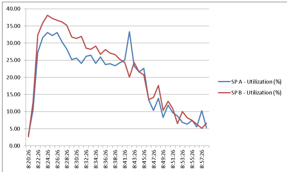
Figure 56 2000 Users EMC VNX5500 SP Utilization Boot Phase
