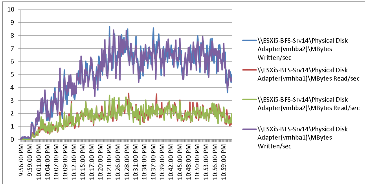
Figure 192 2000 User ESXi Host14 B200 M3 Cisco VIC1240 MLOM Physical Disk Adapter MBps Read/Write Test Phase
