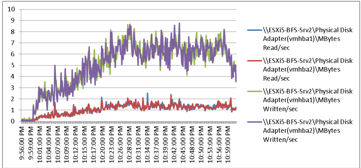
Figure 132 2000 User ESXi Host2 B200 M3 Cisco VIC1240 MLOM Physical Disk Adapter MBps Read/Write Test Phase
