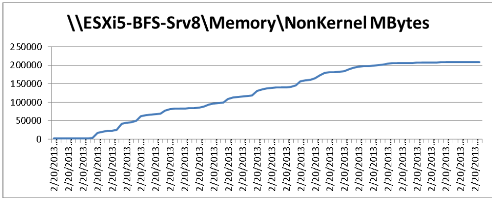
Figure 37 1000 User Single B200 M3 NonKernel Memory - Boot Phase
