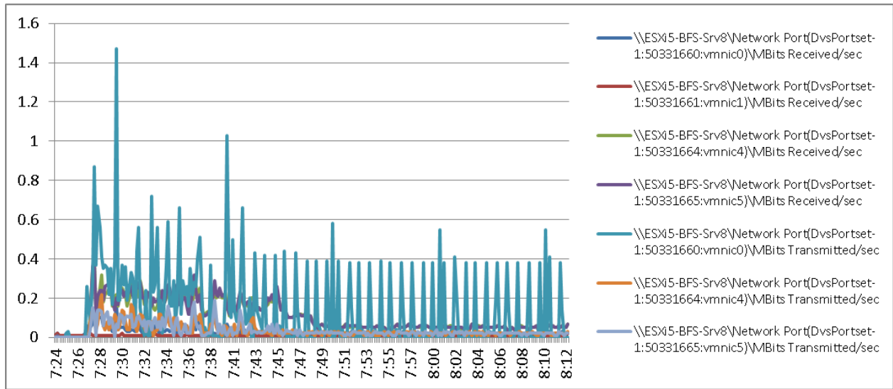
Figure 101 2000 User ESXi Host8 B200 M3 Cisco VIC1240 MLOM Network Adapter Mbps Receive/Transmit Boot Phase
