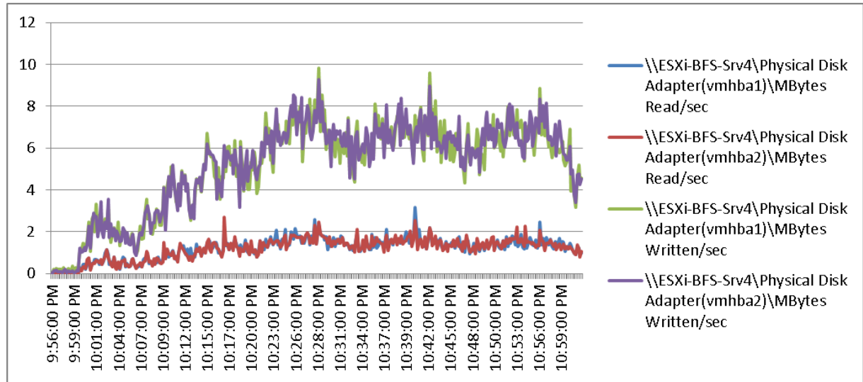
Figure 142 2000 User ESXi Host4 B200 M3 Cisco VIC1240 MLOM Physical Disk Adapter MBps Read/Write Test Phase
