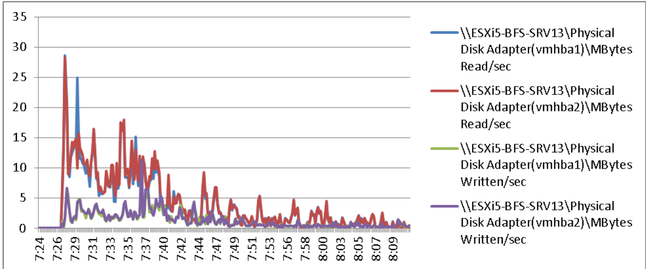
Figure 122 2000 User ESXi Host13 B200 M3 Cisco VIC1240 MLOM Physical Disk Adapter MBps Read/Write Boot Phase
