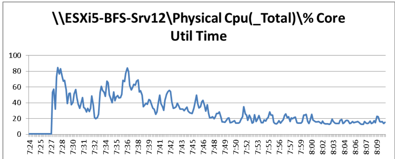
Figure 113 2000 User ESXi Host12 B200 M3 Processor Core Utilization Boot Phase
