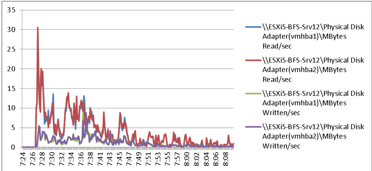
Figure 117 2000 User ESXi Host12 B200 M3 Cisco VIC1240 MLOM Physical Disk Adapter MBps Read/Write Boot Phase
