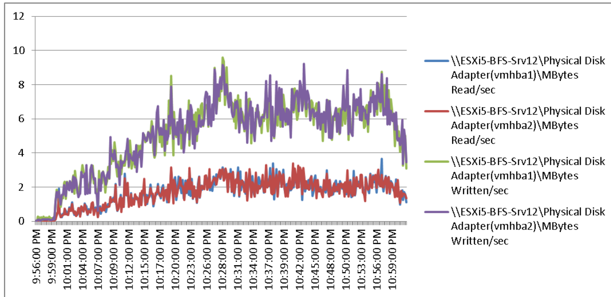
Figure 182 2000 User ESXi Host12 B200 M3 Cisco VIC1240 MLOM Physical Disk Adapter MBps Read/Write Test Phase
