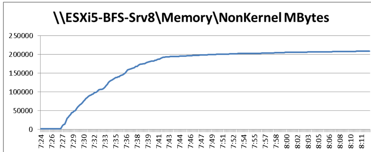
Figure 100 2000 User ESXi Host8 B200 M3 Memory NonKernel MBytes Boot Phase
