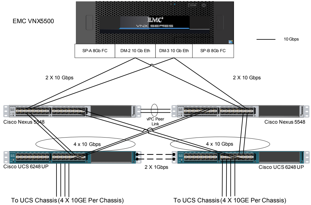
Figure 15 EMC VNX Ethernet Connectivity
