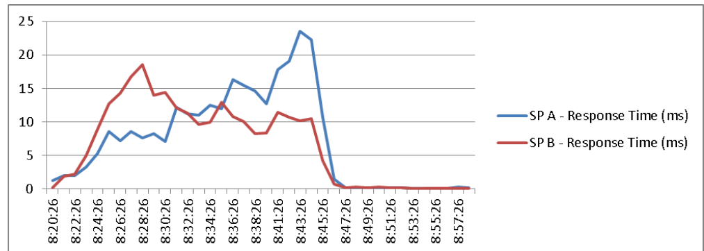
Figure 57 2000 Users EMC VNX5500 SP Response Time Boot Phase
