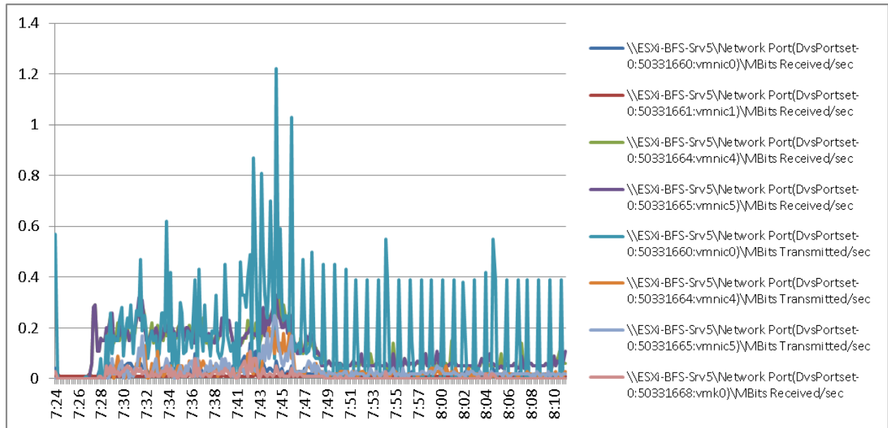
Figure 86 2000 User ESXi Host5 B200 M3 Cisco VIC1240 MLOM Network Adapter Mbps Receive/Transmit Boot Phase
