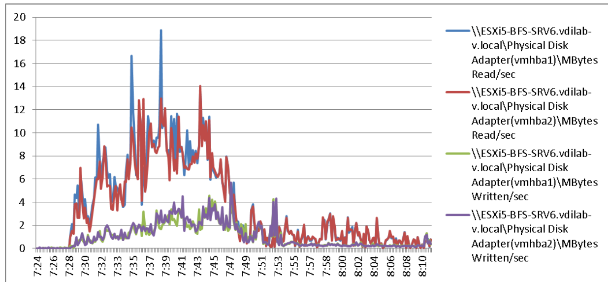
Figure 92 2000 User ESXi Host6 B200 M3 Cisco VIC1240 MLOM Physical Disk Adapter MBps Read/Write Boot Phase
