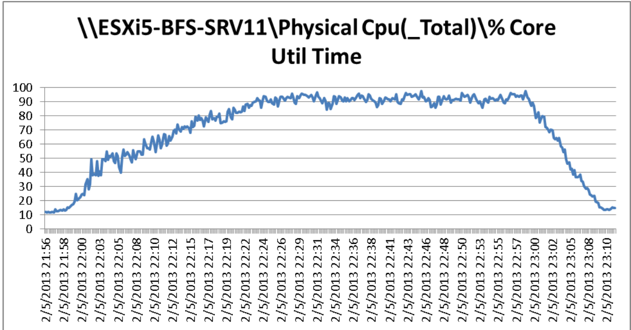
Figure 173 2000 User ESXi Host11 B200 M3 Processor Core Utilization Test Phase
