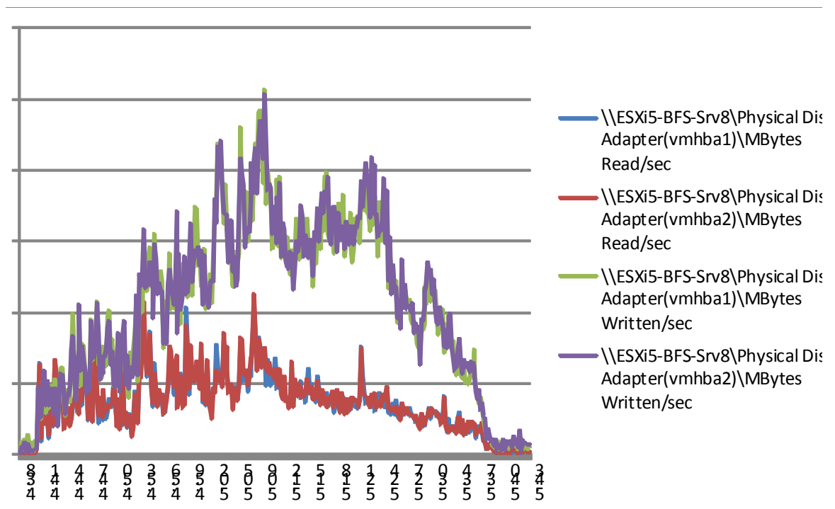
Figure 44 1000 User Single B200 M3 Cisco VIC1240 MLOM Physical Disk Adapter MBps Read/Write Test Phase
