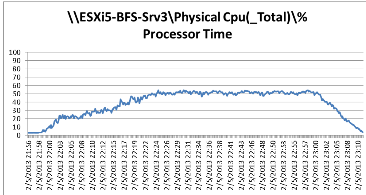
Figure 134 2000 User ESXi Host3 B200 M3 Processor Time Test Phase
