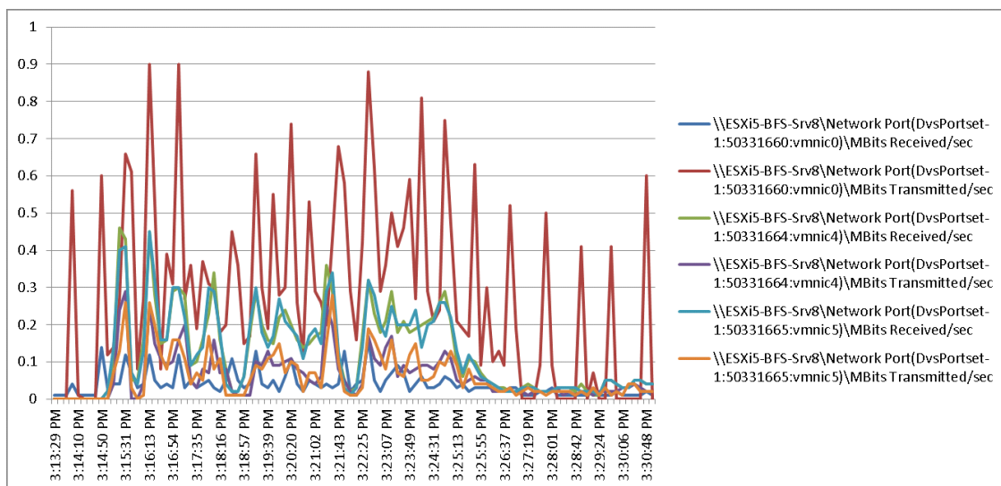
Figure 38 1000 User Single B200 M3 Cisco VIC1240 MLOM Network Adapter Mbps Receive/Transmit Boot Phase
