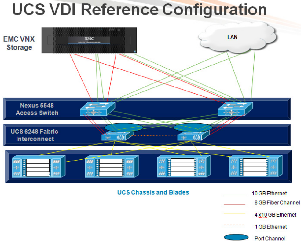
Figure 9 Architecture Block Diagram
