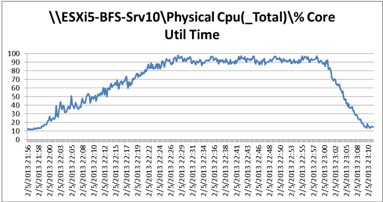
Figure 168 2000 User ESXi Host10 B200 M3 Processor Core Utilization Test Phase
