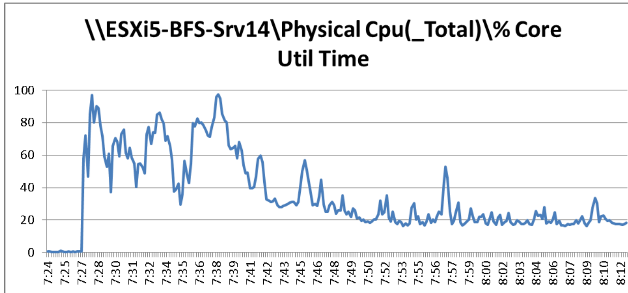
Figure 123 2000 User ESXi Host14 B200 M3 Processor Core Utilization Boot Phase
