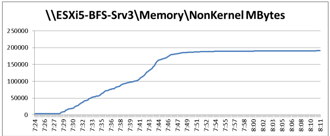
Figure 75 2000 User ESXi Host3 B200 M3 Memory NonKernel MBytes Boot Phase
