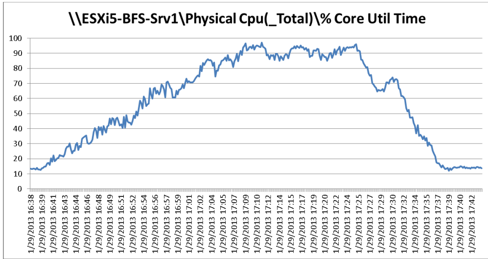
Figure 41 1000 User Single B200 M3 CPU Processor Time - Test Phase
