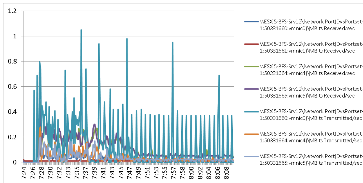
Figure 116 2000 User ESXi Host12 B200 M3 Cisco VIC1240 MLOM Network Adapter Mbps Receive/Transmit Boot Phase
