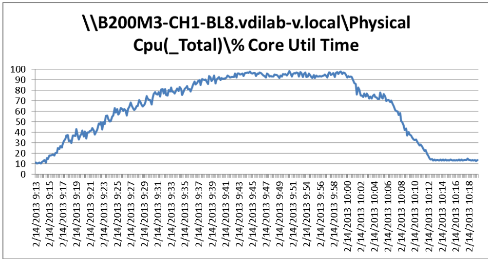
Figure 29 155 User Single B200 M3 CPU Core Utilization - Test Phase
