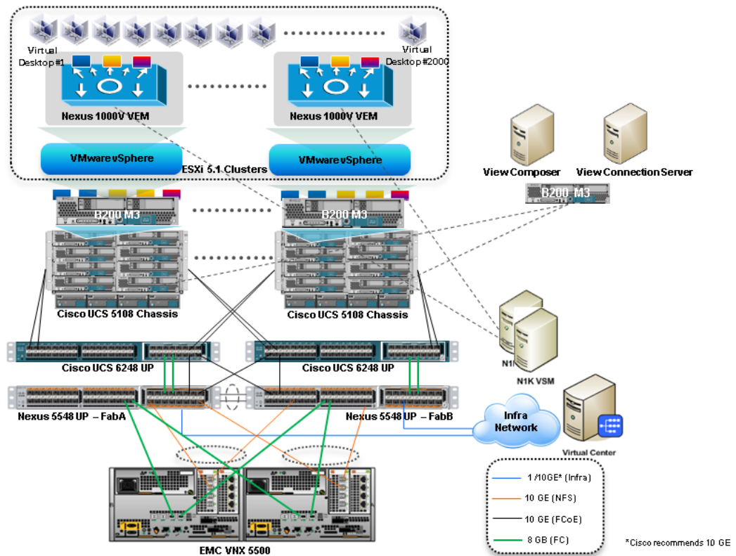
Figure 6 VMware View 5.1 on Cisco Unified Computing System
