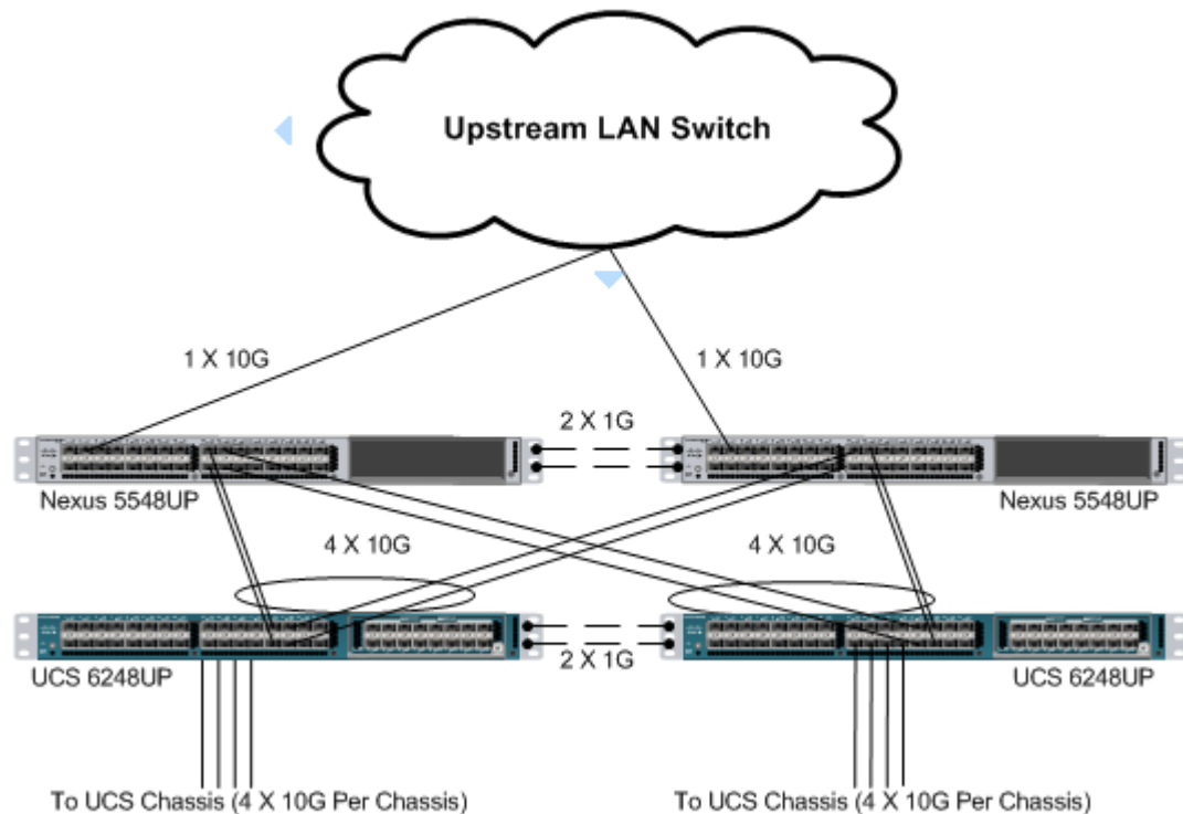
Figure 14 Ethernet Network Configuration with Upstream Cisco Nexus 5500 Series from the Cisco Unified Computing System 6200 Series Fabric Interconnects
