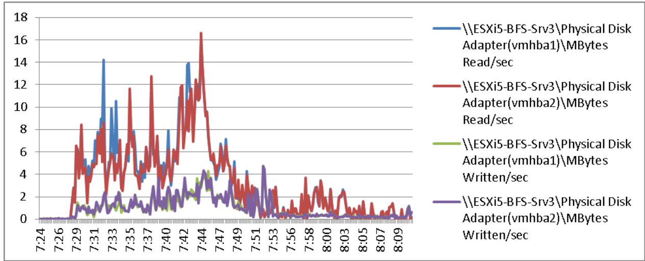
Figure 77 2000 User ESXi Host3 B200 M3 Cisco VIC1240 MLOM Physical Disk Adapter MBps Read/Write Boot Phase
