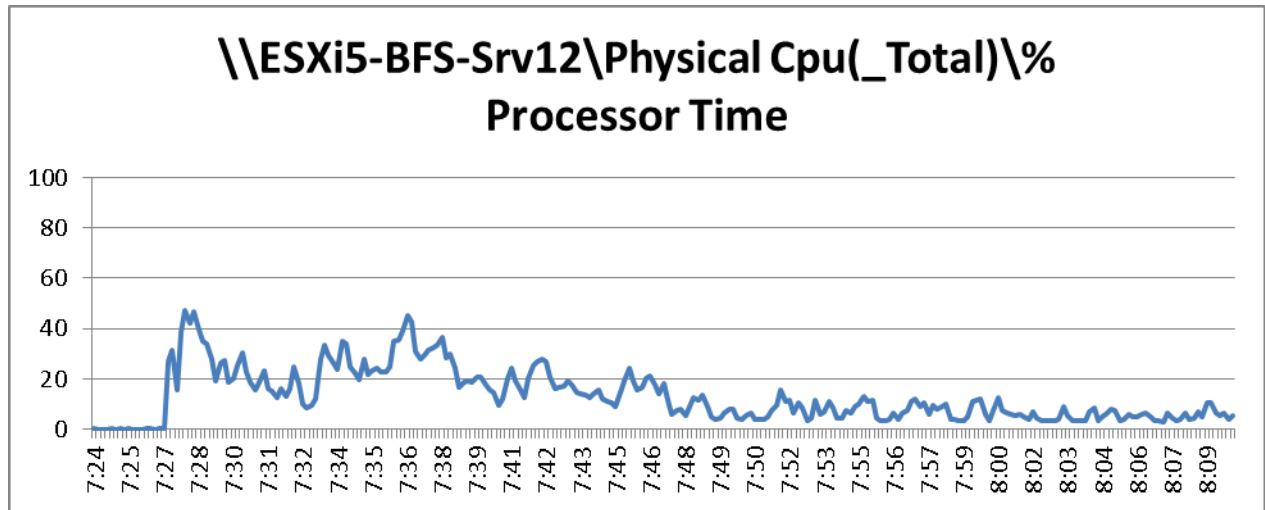
Figure 114 2000 User ESXi Host12 B200 M3 Processor Time Boot Phase
