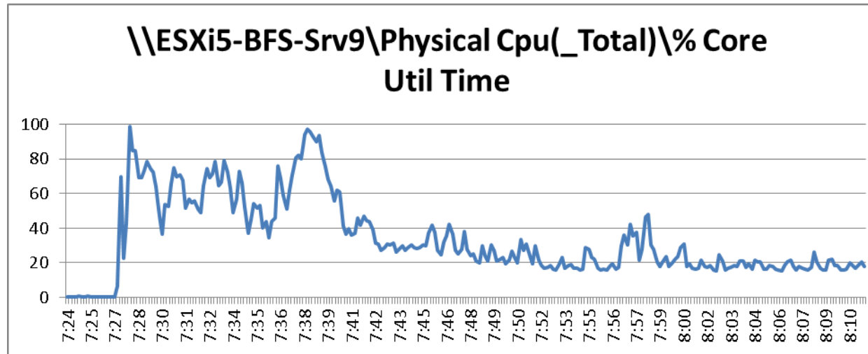
Figure 103 2000 User ESXi Host9 B200 M3 Processor Core Utilization Boot Phase
