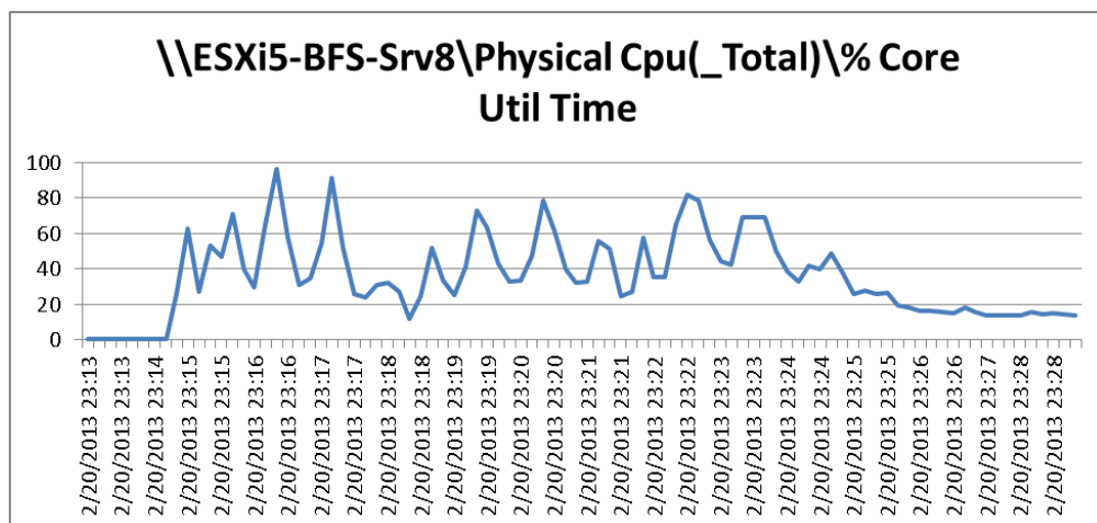
Figure 35 1000 User Single B200 M3 CPU Core Utilization - Boot Phase
