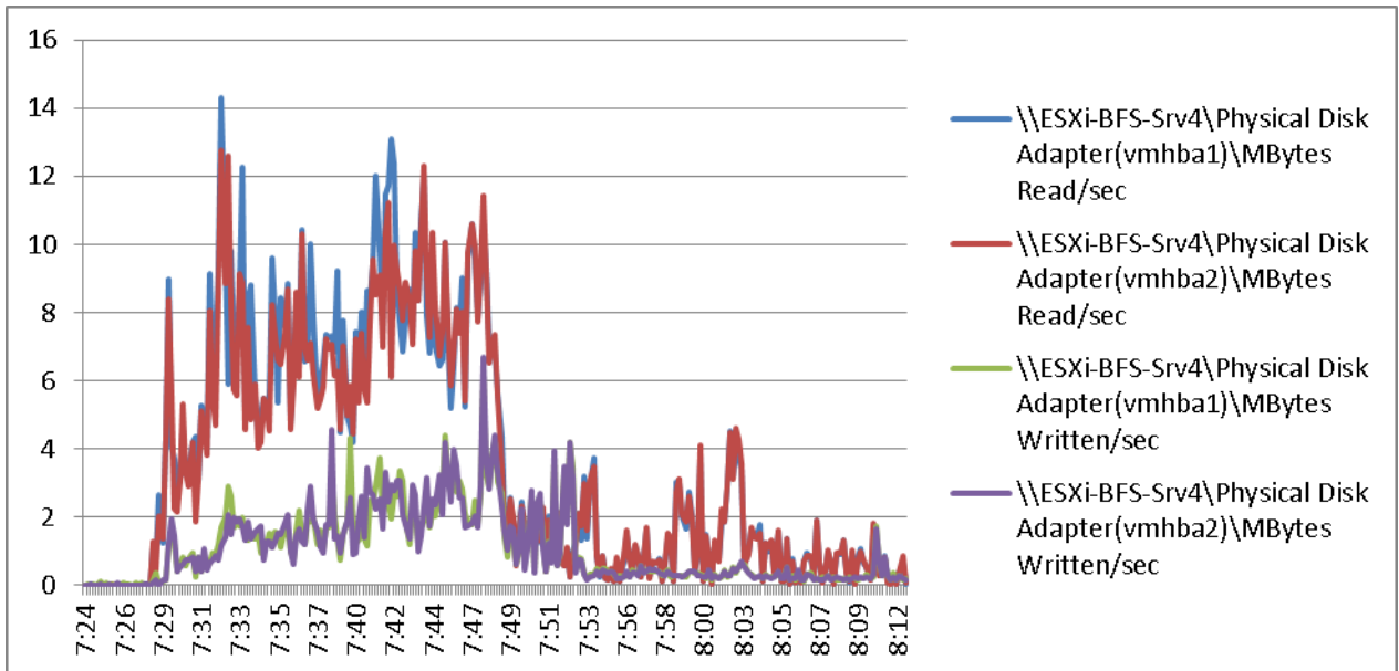
Figure 82 2000 User ESXi Host4 B200 M3 Cisco VIC1240 MLOM Physical Disk Adapter MBps Read/Write Boot Phase
