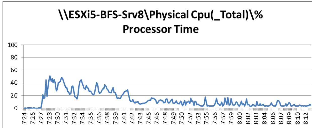
Figure 99 2000 User ESXi Host8 B200 M3 Processor Time Boot Phase
