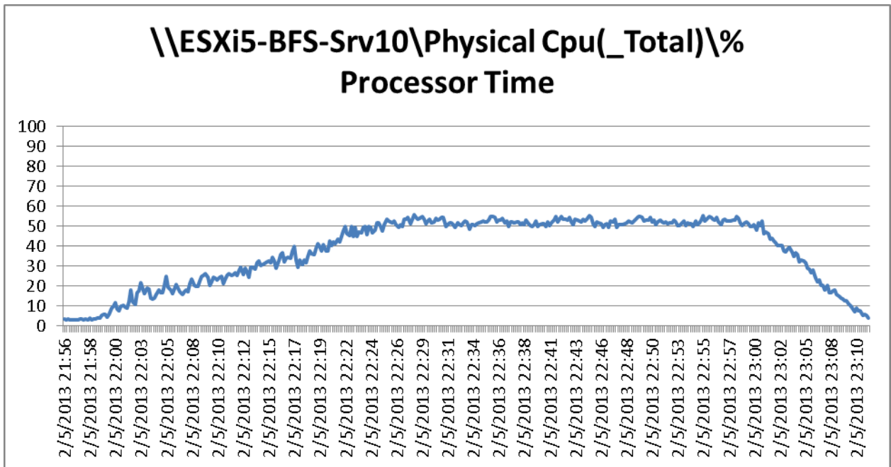
Figure 169 2000 User ESXi Host10 B200 M3 Processor Time Test Phase
