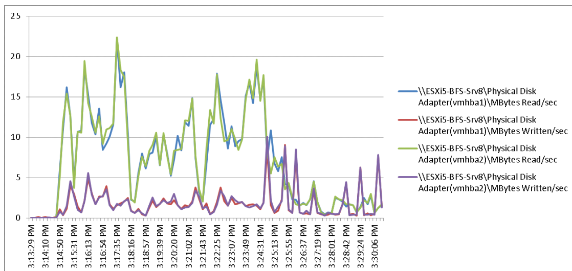
Figure 39 1000 User Single B200 M3 Cisco VIC1240 MLOM Physical Disk Adapter MBps Read/Write Boot Phase
