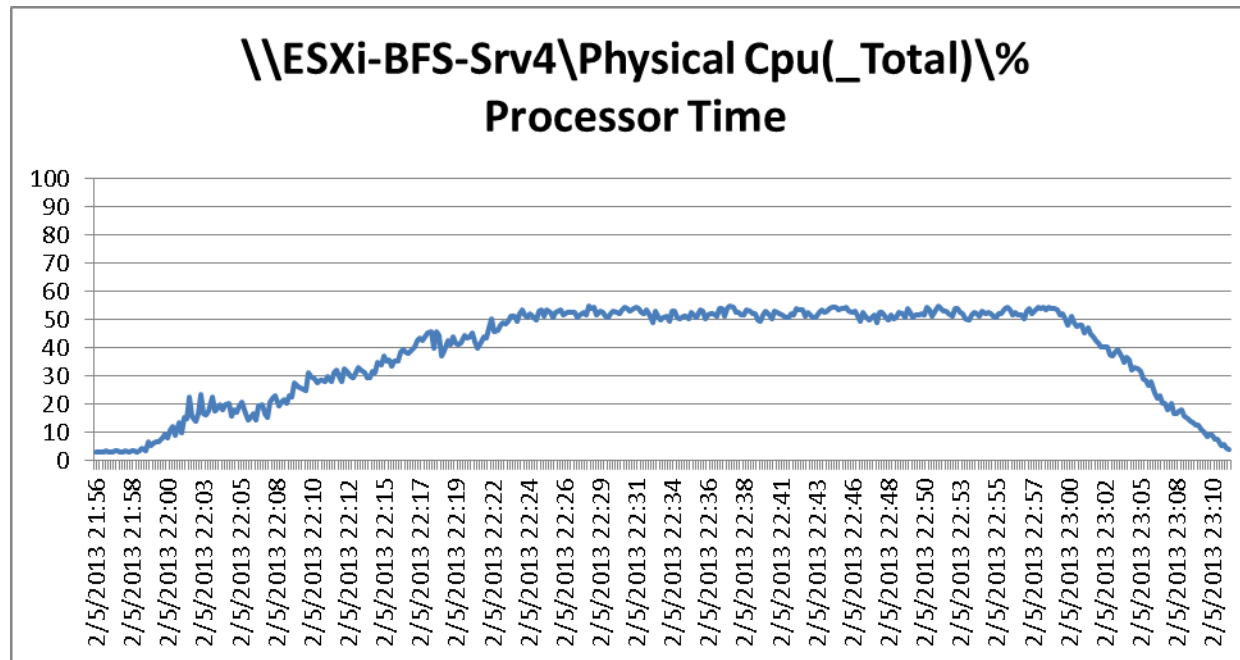
Figure 139 2000 User ESXi Host4 B200 M3 Processor Time Test Phase
