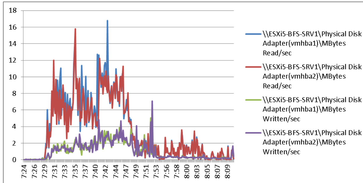
Figure 67 2000 User ESXi Host1 B200 M3 Cisco VIC1240 MLOM Physical Disk Adapter MBps Read/Write Boot Phase
