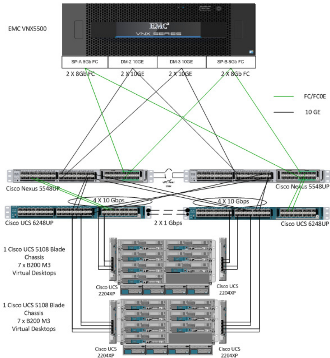
Figure 10 Detailed Architecture of the Configuration
