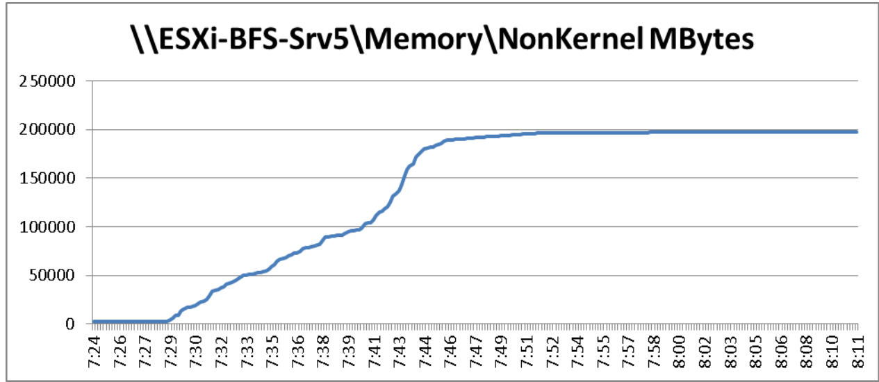
Figure 85 2000 User ESXi Host5 B200 M3 Memory NonKernel MBytes Boot Phase
