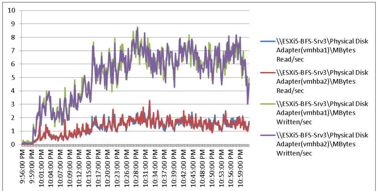
Figure 137 2000 User ESXi Host3 B200 M3 Cisco VIC1240 MLOM Physical Disk Adapter MBps Read/Write Test Phase
