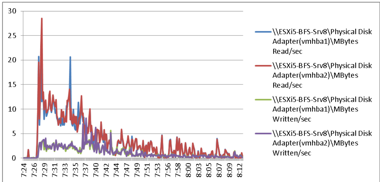
Figure 102 2000 User ESXi Host8 B200 M3 Cisco VIC1240 MLOM Physical Disk Adapter MBps Read/Write Boot Phase
