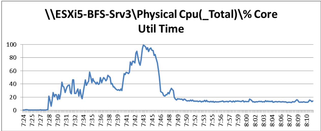
Figure 73 2000 User ESXi Host3 B200 M3 Processor Core Utilization Boot Phase
