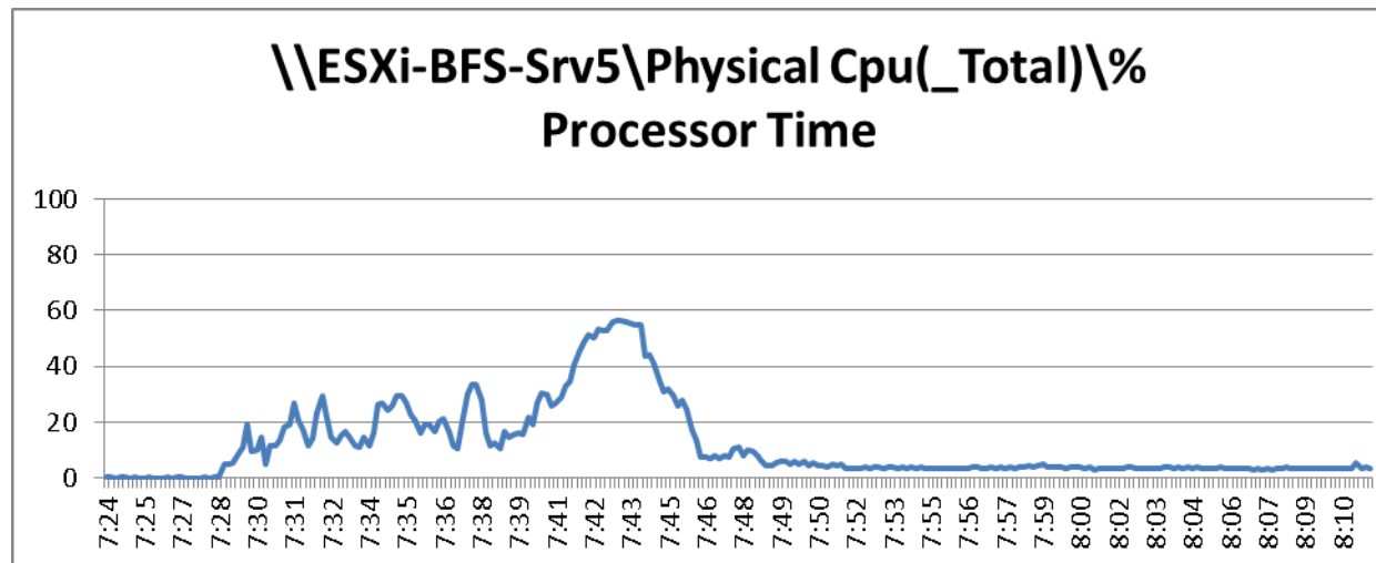
Figure 84 2000 User ESXi Host5 B200 M3 Processor Time Boot Phase
