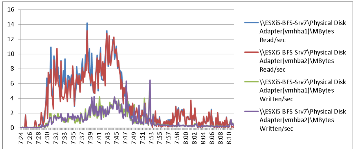
Figure 97 2000 User ESXi Host7 B200 M3 Cisco VIC1240 MLOM Physical Disk Adapter MBps Read/Write Boot Phase
