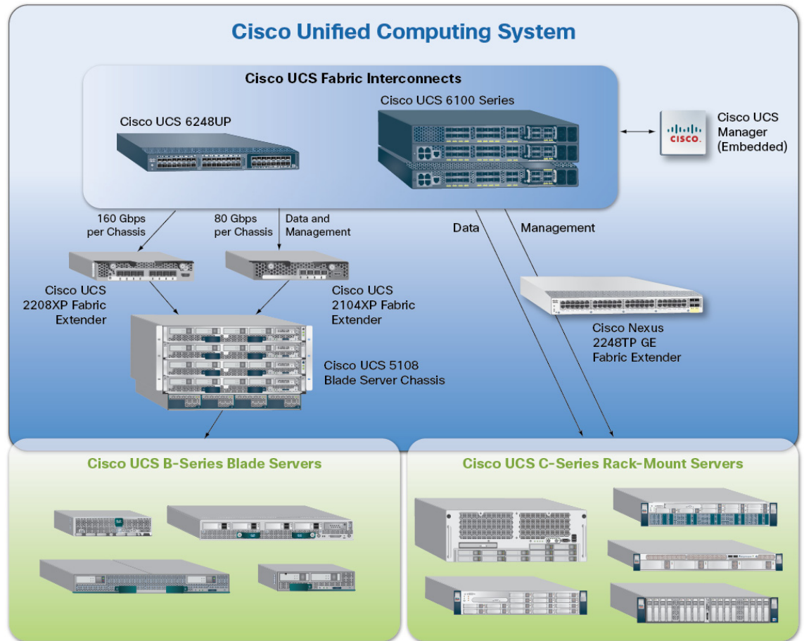
Figure 2 Cisco Unified Computing System Components
