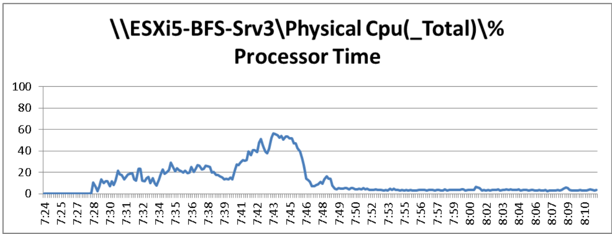
Figure 74 2000 User ESXi Host3 B200 M3 Processor Time Boot Phase
