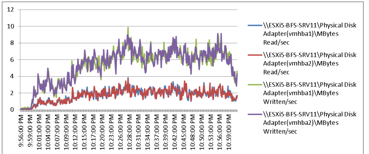
Figure 177 2000 User ESXi Host11 B200 M3 Cisco VIC1240 MLOM Physical Disk Adapter MBps Read/Write Test Phase
