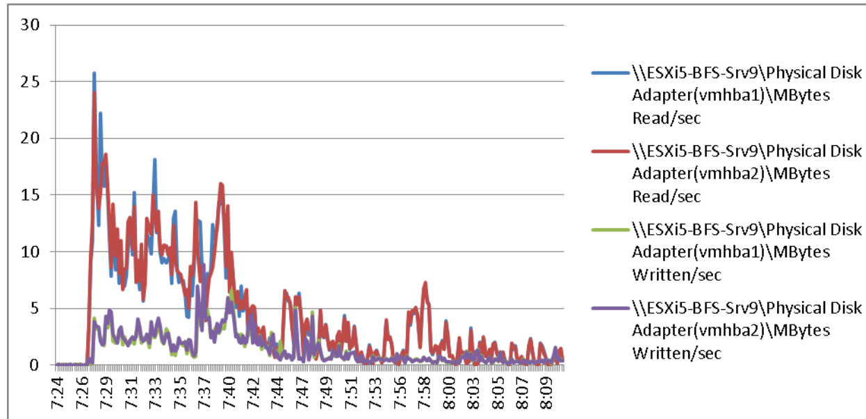
Figure 107 2000 User ESXi Host9 B200 M3 Cisco VIC1240 MLOM Physical Disk Adapter MBps Read/Write Boot Phase
