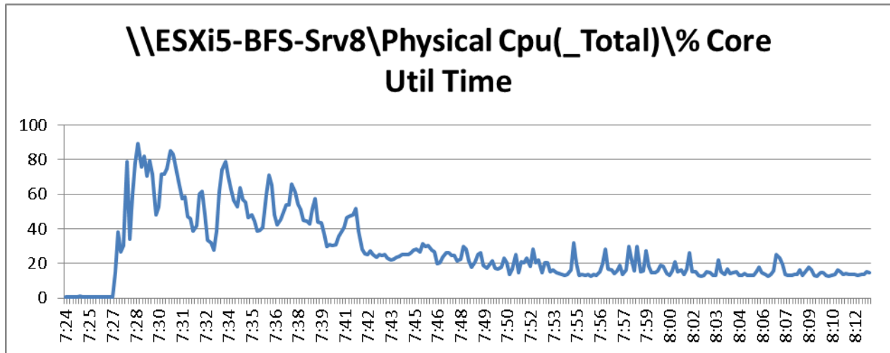
Figure 98 2000 User ESXi Host8 B200 M3 Processor Core Utilization Boot Phase
