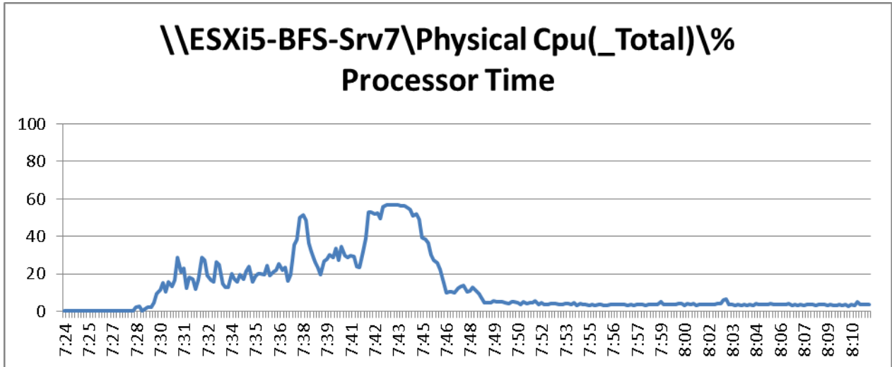
Figure 94 2000 User ESXi Host7 B200 M3 Processor Time Boot Phase
