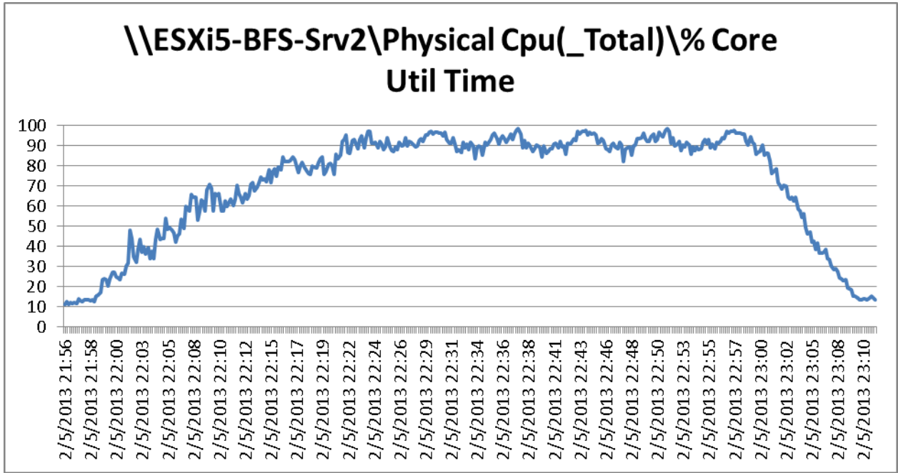
Figure 128 2000 User ESXi Host2 B200 M3 Processor Core Utilization Test Phase
