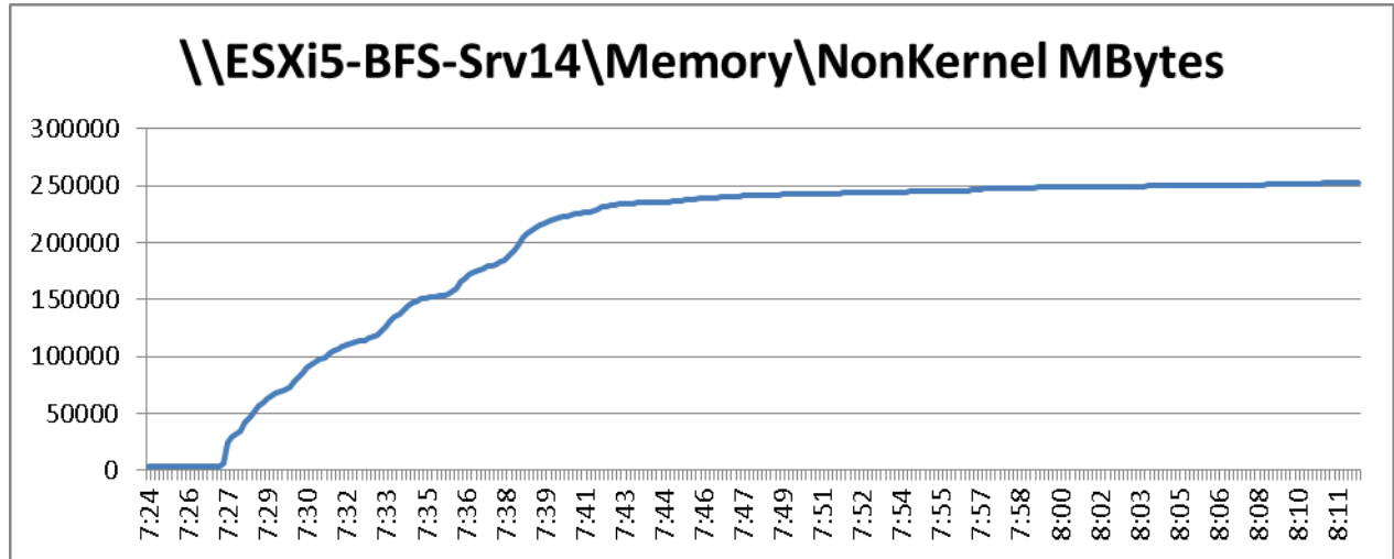
Figure 125 2000 User ESXi Host14 B200 M3 Memory NonKernel MBytes Boot Phase
