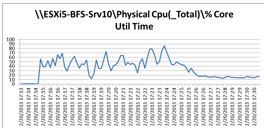
Figure 46 2000 User Single B200 M3 CPU Core Utilization - Boot Phase
