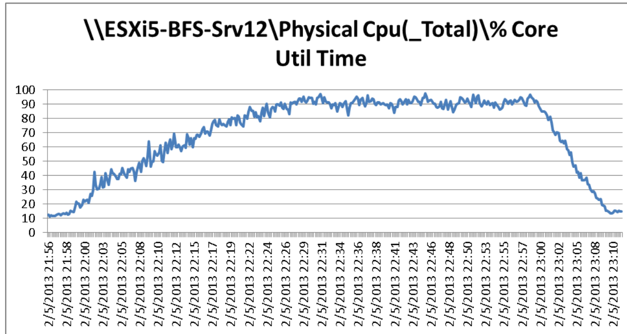
Figure 178 2000 User ESXi Host12 B200 M3 Processor Core Utilization Test Phase
