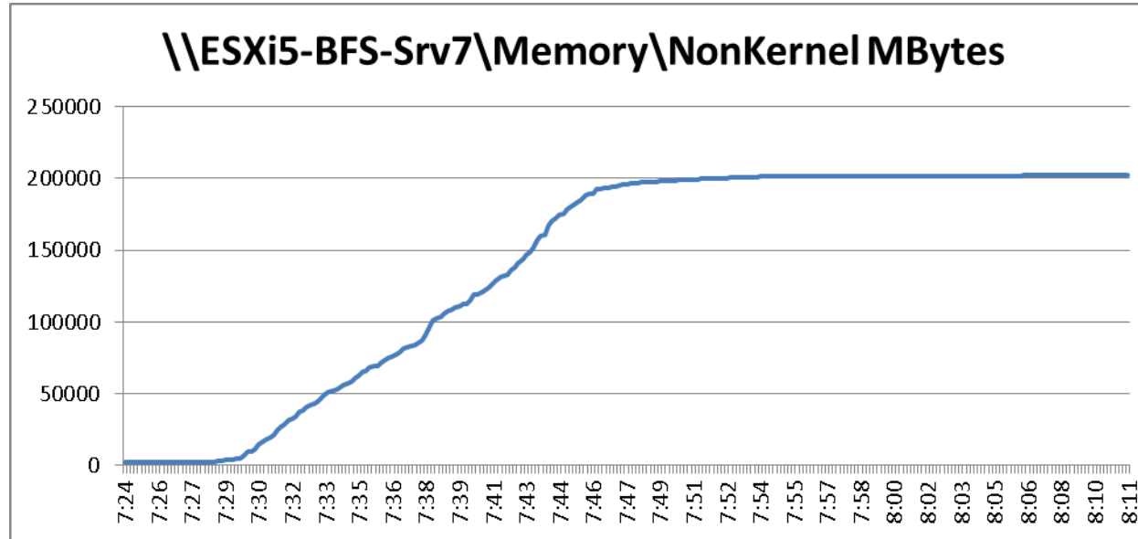
Figure 95 2000 User ESXi Host7 B200 M3 Memory NonKernel MBytes Boot Phase
