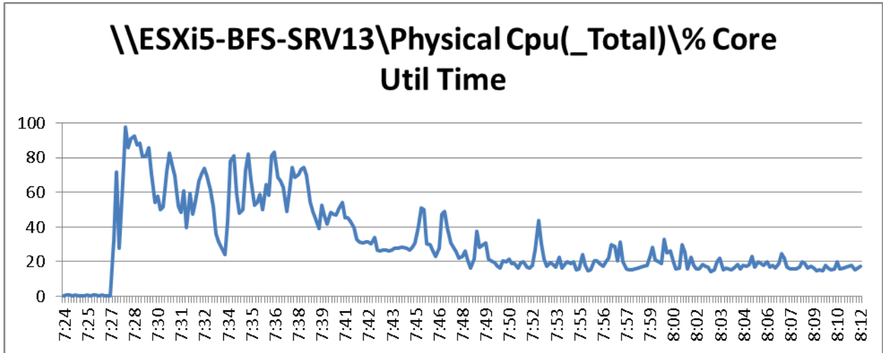
Figure 118 2000 User ESXi Host13 B200 M3 Processor Core Utilization Boot Phase
