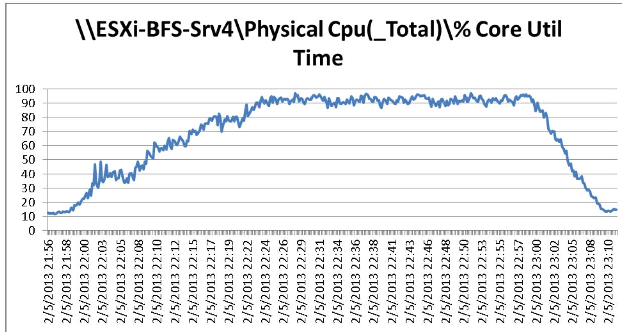
Figure 138 2000 User ESXi Host4 B200 M3 Processor Core Utilization Test Phase
