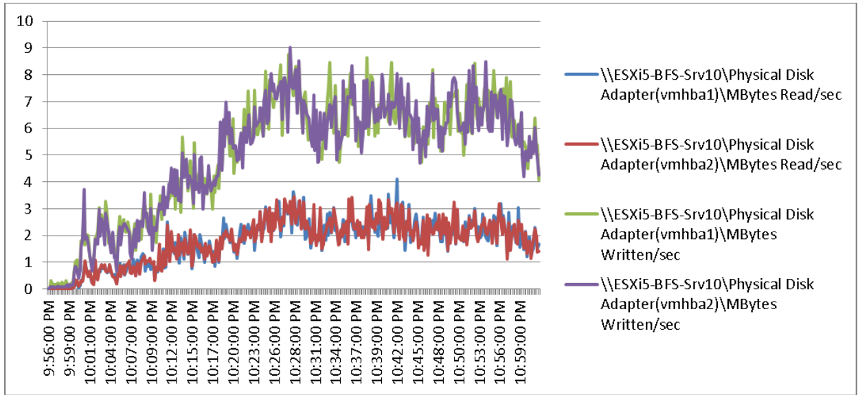
Figure 172 2000 User ESXi Host10 B200 M3 Cisco VIC1240 MLOM Physical Disk Adapter MBps Read/Write Test Phase
