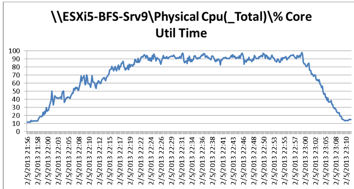
Figure 163 2000 User ESXi Host9 B200 M3 Processor Core Utilization Test Phase
