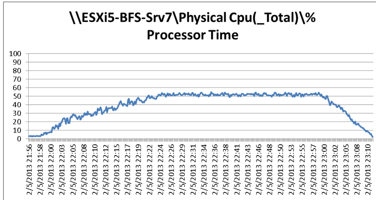
Figure 154 2000 User ESXi Host7 B200 M3 Processor Time Test Phase
