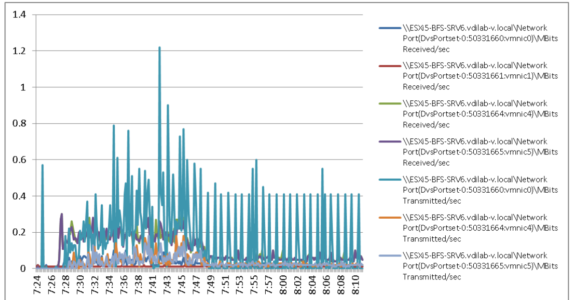
Figure 91 2000 User ESXi Host6 B200 M3 Cisco VIC1240 MLOM Network Adapter Mbps Receive/Transmit Boot Phase
