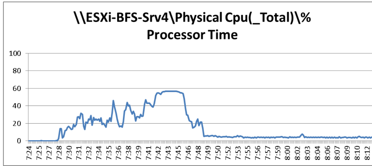
Figure 79 2000 User ESXi Host4 B200 M3 Processor Time Boot Phase
