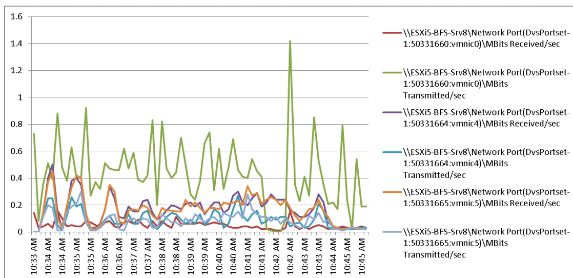
Figure 27 155 User Single B200 M3 Cisco VIC1240 MLOM Network Adapter Mbps Receive/Transmit Boot Phase
