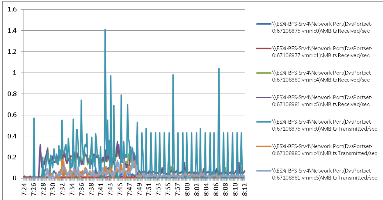
Figure 81 2000 User ESXi Host4 B200 M3 Cisco VIC1240 MLOM Network Adapter Mbps Receive/Transmit Boot Phase
