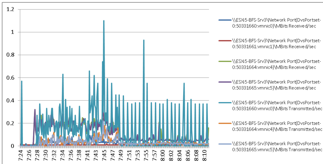
Figure 76 2000 User ESXi Host3 B200 M3 Cisco VIC1240 MLOM Network Adapter Mbps Receive/Transmit Boot Phase
