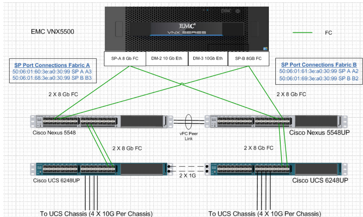
Figure 17 VNX5500 FC Target Ports
