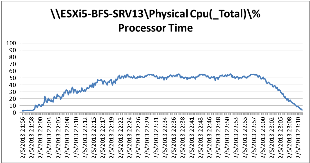
Figure 184 2000 User ESXi Host13 B200 M3 Processor Time Test Phase
