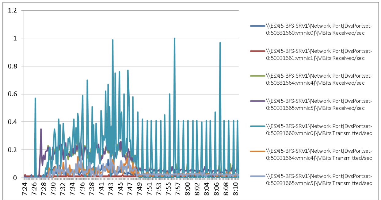
Figure 66 2000 User ESXi Host1 B200 M3 Cisco VIC1240 MLOM Network Adapter Mbps Receive/Transmit Boot Phase
