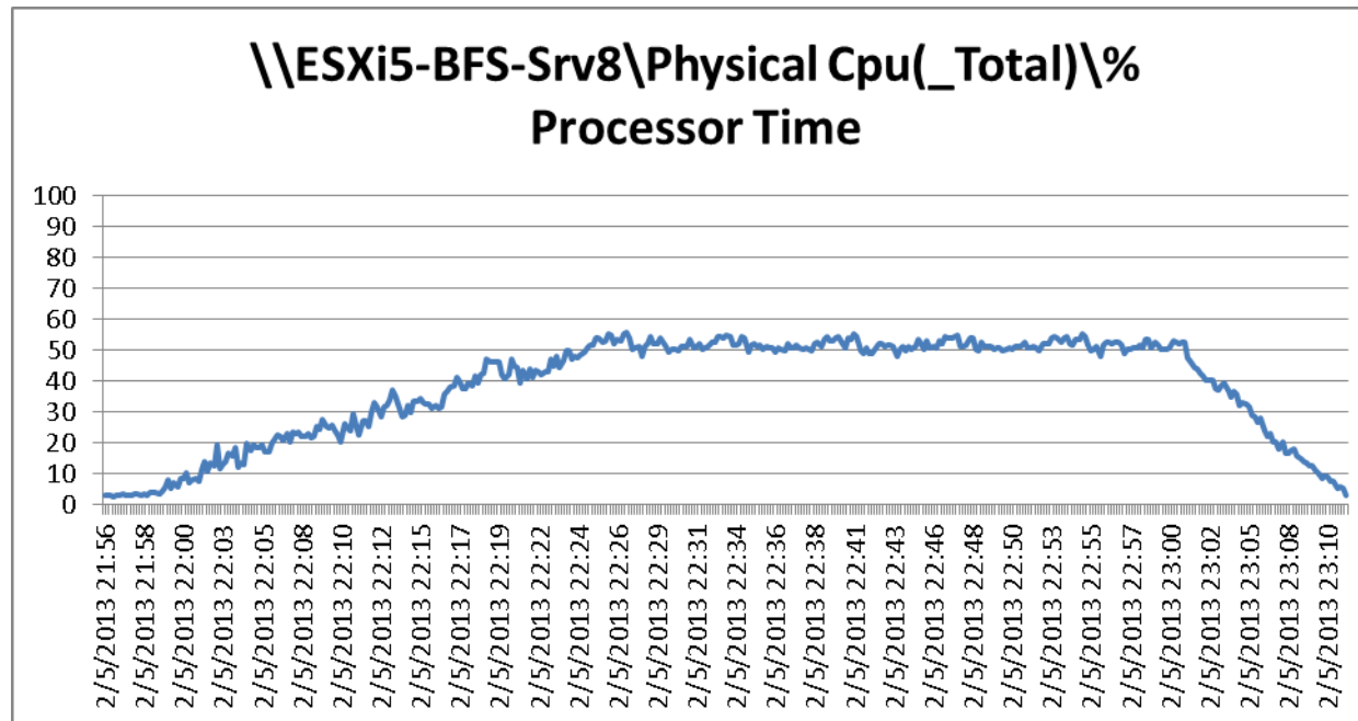
Figure 159 2000 User ESXi Host8 B200 M3 Processor Time Test Phase
