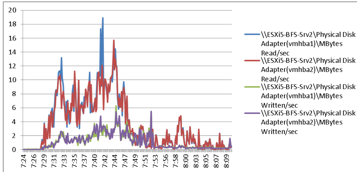
Figure 72 2000 User ESXi Host2 B200 M3 Cisco VIC1240 MLOM Physical Disk Adapter MBps Read/Write Boot Phase
