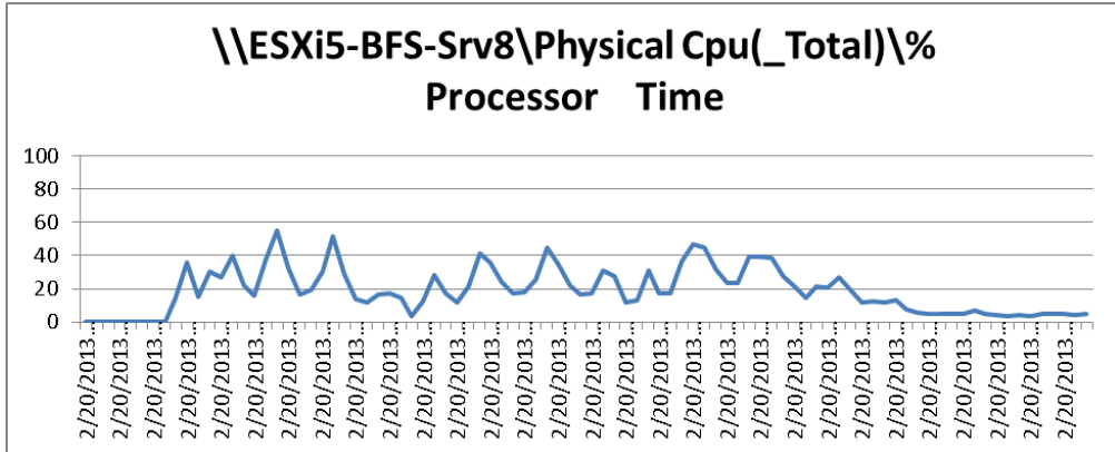
Figure 36 1000 User Single B200 M3 CPU Processor Time - Boot Phase
