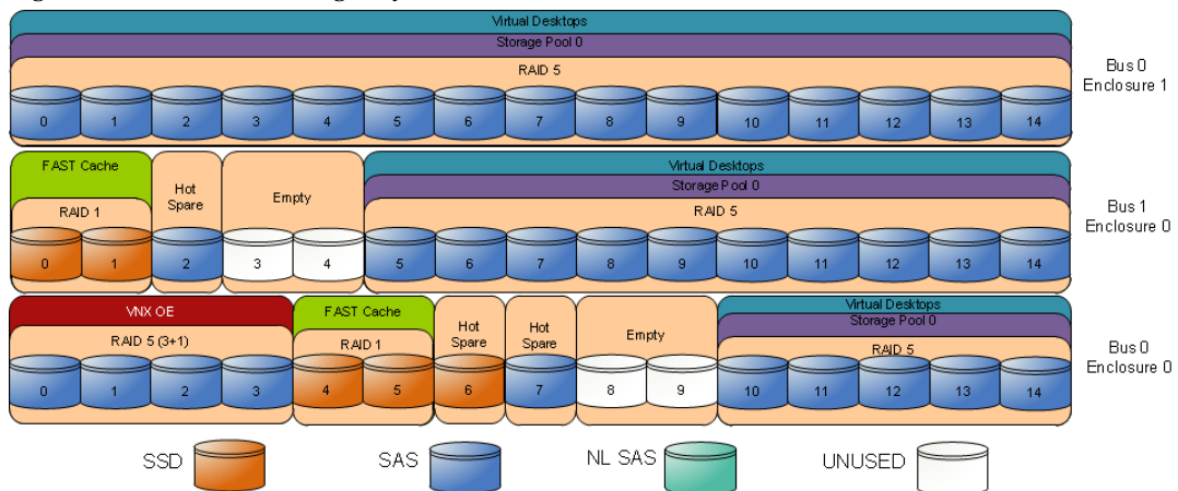
Figure 18 Core Storage Layout on VNX5500
