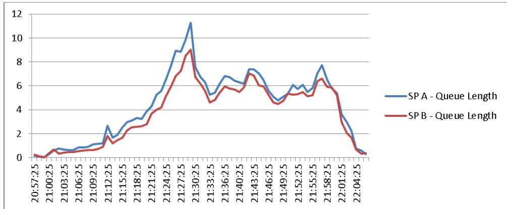
Figure 60 2000 Users EMC VNX5500 SP Queue Lengths Test Phase
