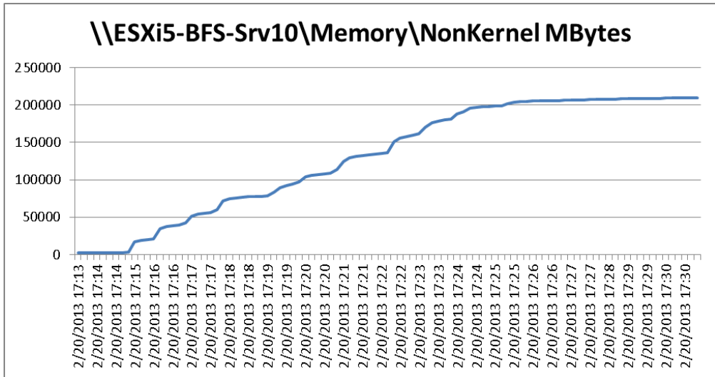
Figure 48 2000 User Single B200 M3 Memory NonKernel - Boot Phase
