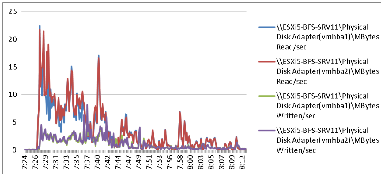
Figure 112 2000 User ESXi Host11 B200 M3 Cisco VIC1240 MLOM Physical Disk Adapter MBps Read/Write Boot Phase
