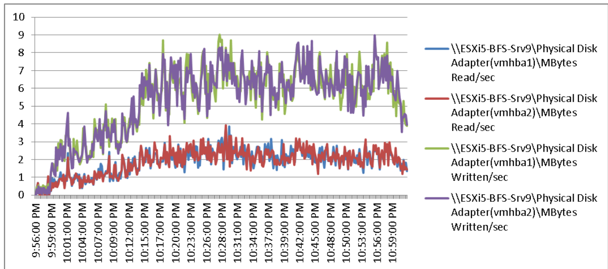
Figure 167 2000 User ESXi Host9 B200 M3 Cisco VIC1240 MLOM Physical Disk Adapter MBps Read/Write Test Phase
