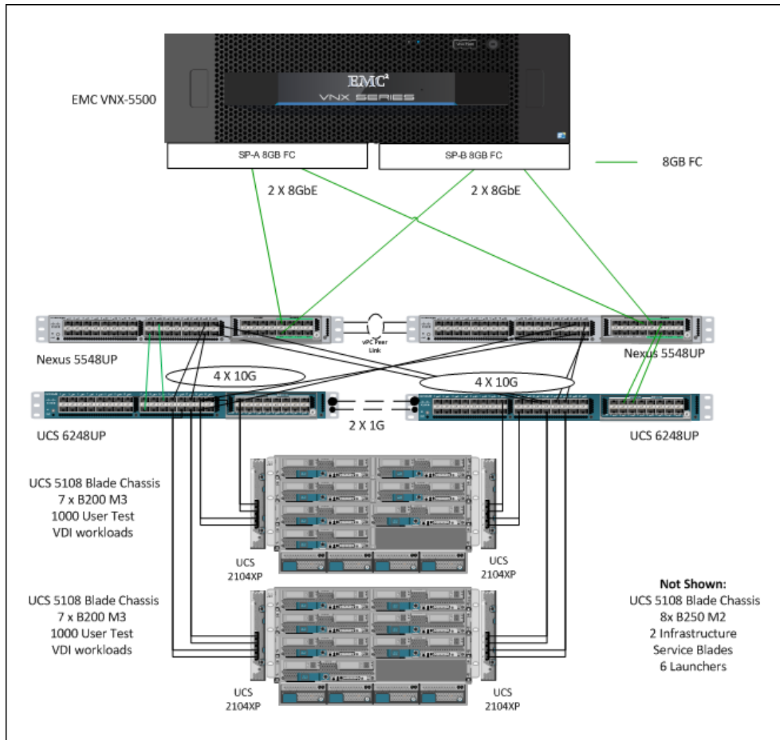
Figure 16 Figure 15a. EMC VNX Fibre Channel Connectivity
