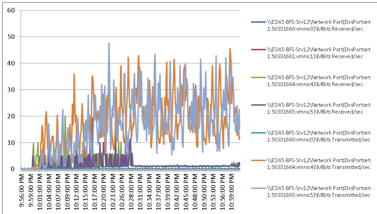
Figure 181 2000 User ESXi Host12 B200 M3 Cisco VIC1240 MLOM Network Adapter Mbps Receive/Transmit Test Phase
