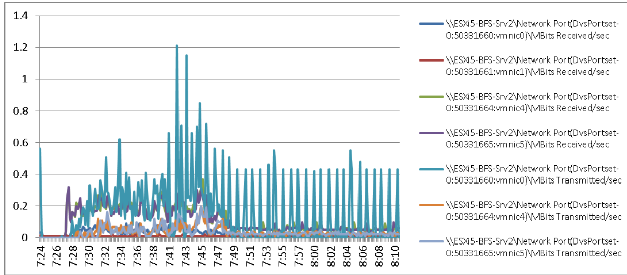
Figure 71 2000 User ESXi Host2 B200 M3 Cisco VIC1240 MLOM Network Adapter Mbps Receive/Transmit Boot Phase
