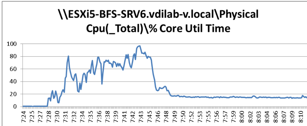
Figure 88 2000 User ESXi Host6 B200 M3 Processor Core Utilization Boot Phase
