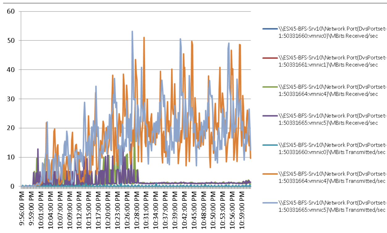
Figure 171 2000 User ESXi Host10 B200 M3 Cisco VIC1240 MLOM Network Adapter Mbps Receive/Transmit Test Phase
