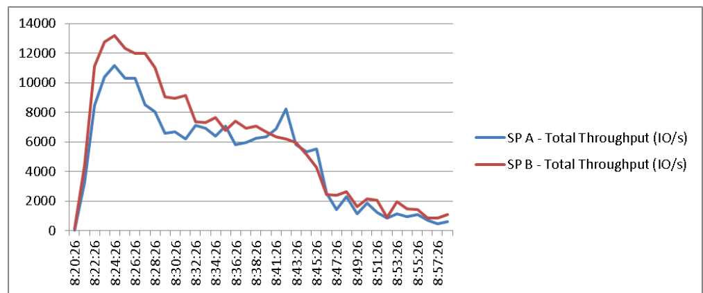
Figure 58 2000 Users EMC VNX5500 SP Total Throughput Boot Phase
