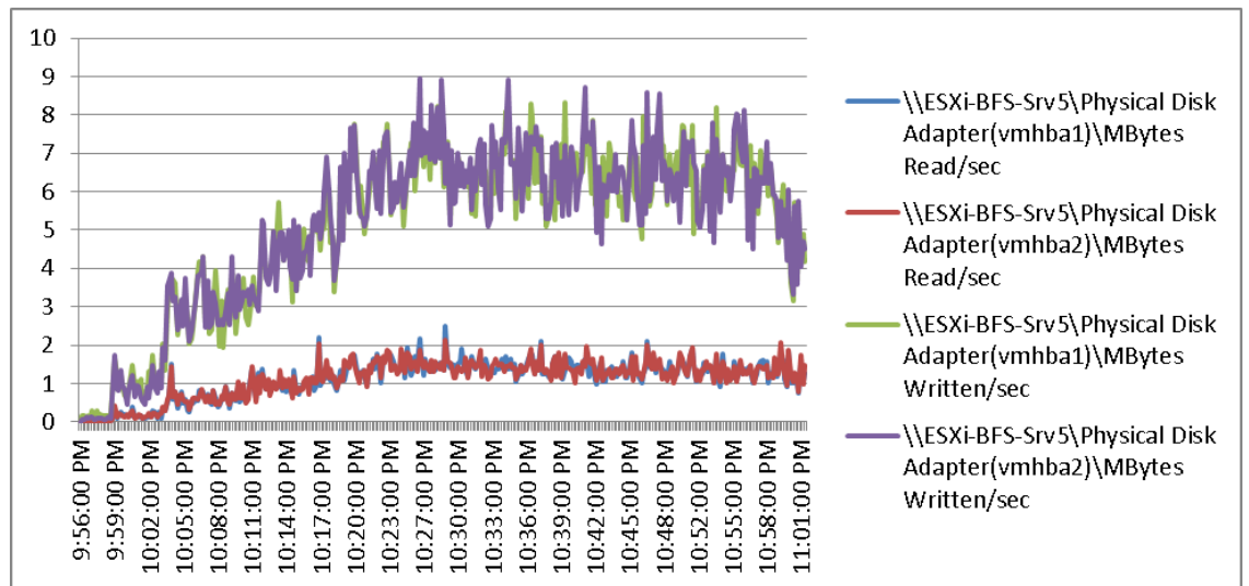
Figure 147 2000 User ESXi Host5 B200 M3 Cisco VIC1240 MLOM Physical Disk Adapter MBps Read/Write Test Phase
