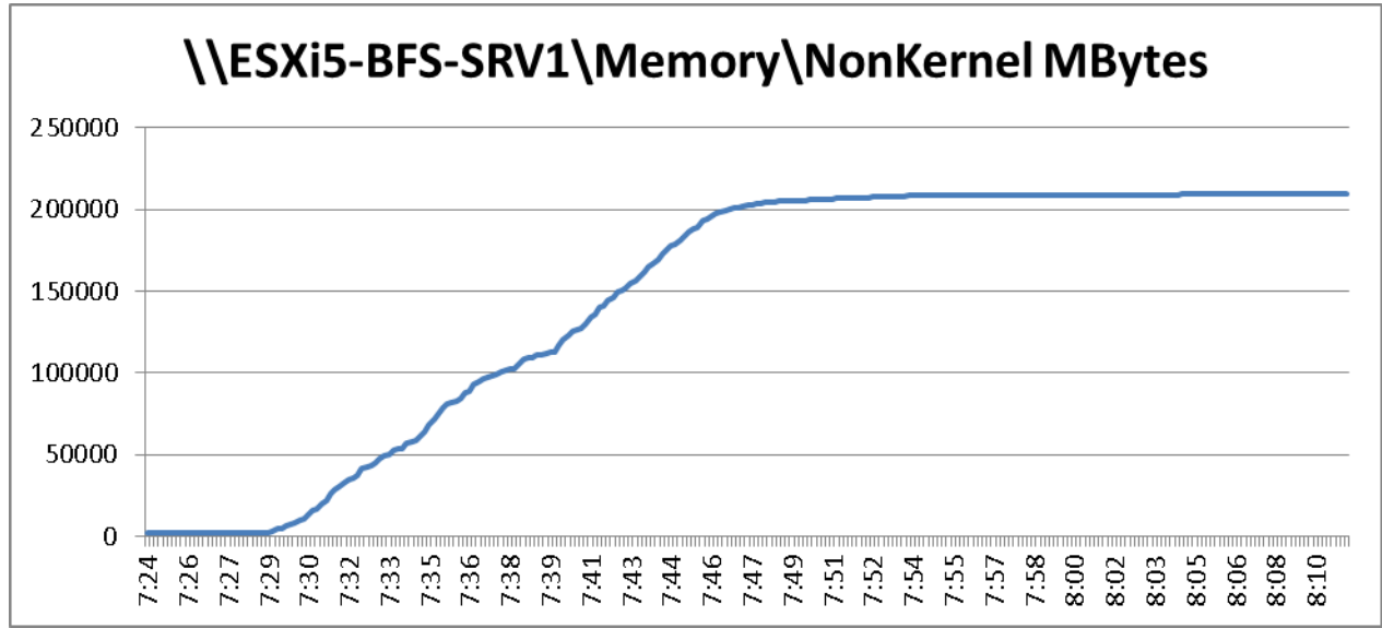
Figure 65 2000 User ESXi Host1 B200 M3 Memory NonKernel MBytes Boot Phase
