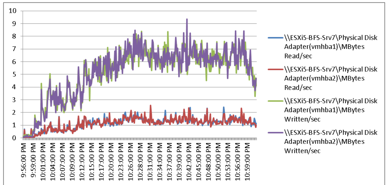
Figure 157 2000 User ESXi Host7 B200 M3 Cisco VIC1240 MLOM Physical Disk Adapter MBps Read/Write Test Phase
