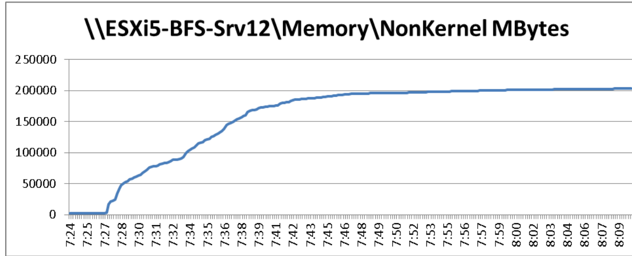
Figure 115 2000 User ESXi Host12 B200 M3 Memory NonKernel MBytes Boot Phase
