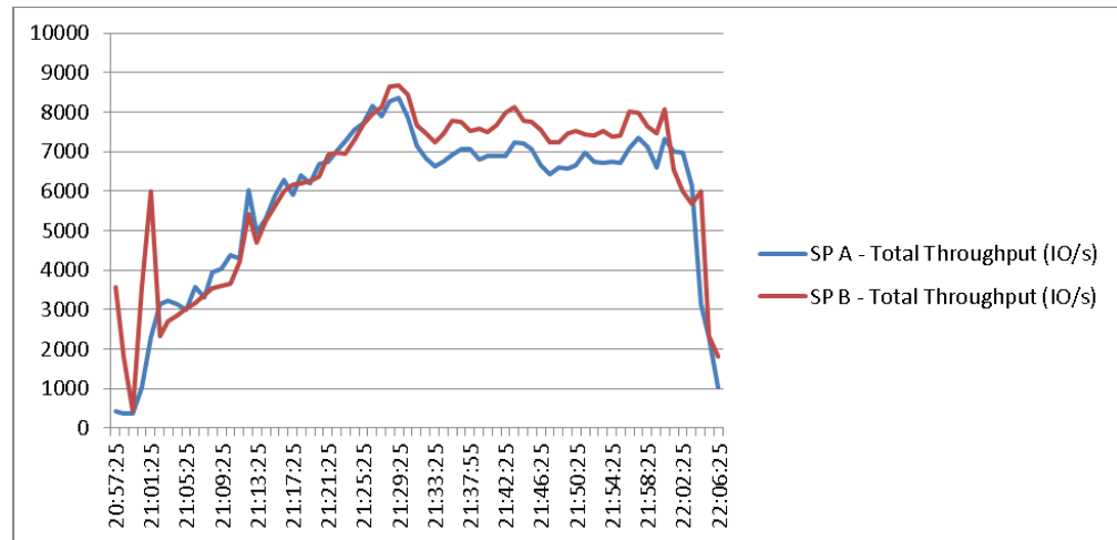
Figure 62 2000 Users EMC VNX5500 SP Total Throughput Test Phase
