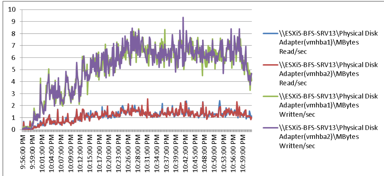
Figure 187 2000 User ESXi Host13 B200 M3 Cisco VIC1240 MLOM Physical Disk Adapter MBps Read/Write Test Phase
