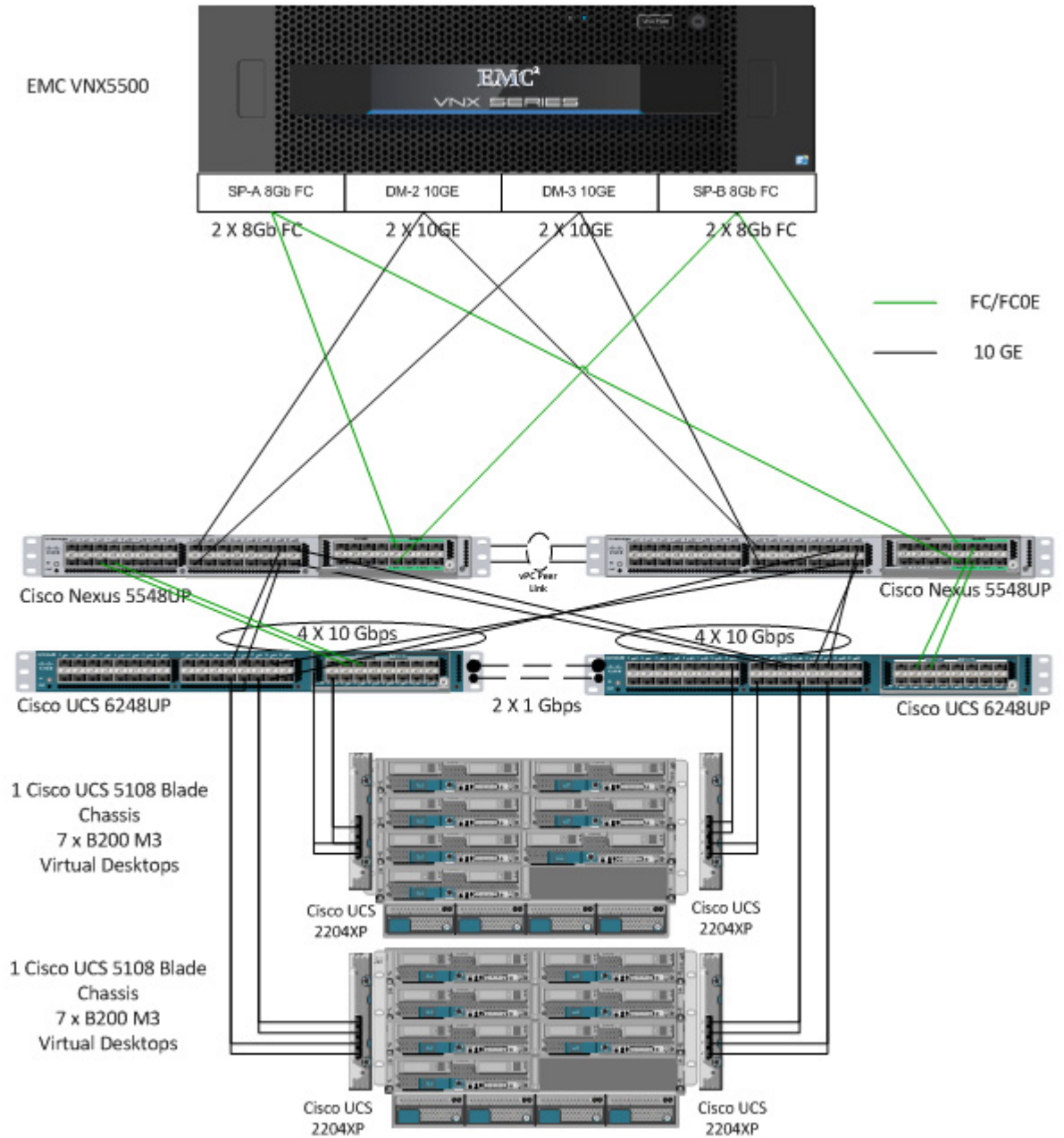
Figure 1 VMware View 5.1 2000 User Hardware Components
