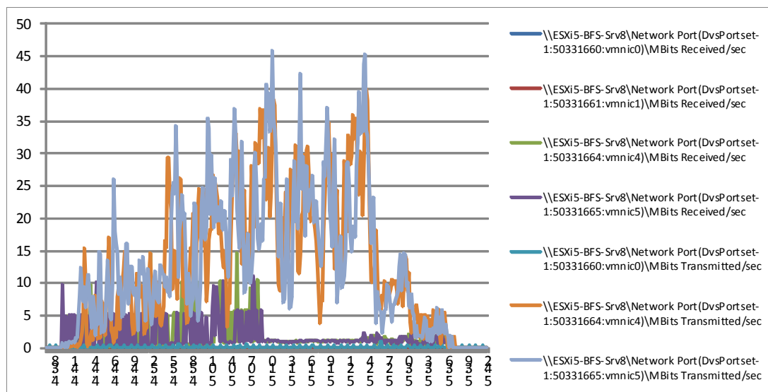
Figure 43 1000 User Single B200 M3 Cisco VIC1240 MLOM Network Adapter Mbps Receive/Transmit Test Phase
