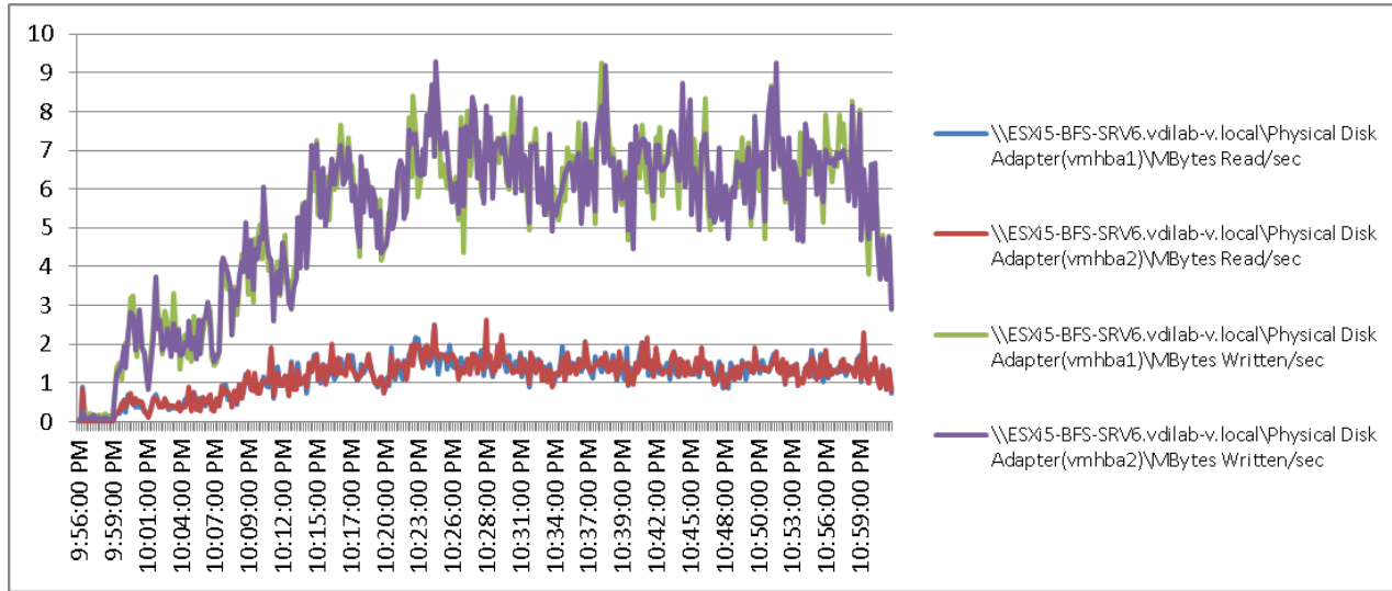
Figure 152 2000 User ESXi Host6 B200 M3 Cisco VIC1240 MLOM Physical Disk Adapter MBps Read/Write Test Phase
