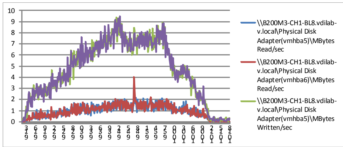
Figure 33 155 User Single B200 M3 Cisco VIC1240 MLOM Physical Disk Adapter MBps Read/Write Test Phase
