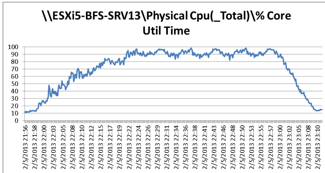
Figure 183 2000 User ESXi Host13 B200 M3 Processor Core Utilization Test Phase
