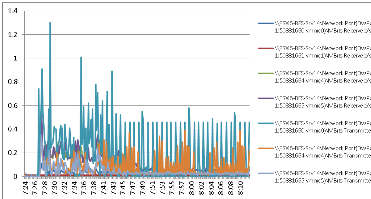
Figure 126 2000 User ESXi Host14 B200 M3 Cisco VIC1240 MLOM Network Adapter Mbps Receive/Transmit Boot Phase
