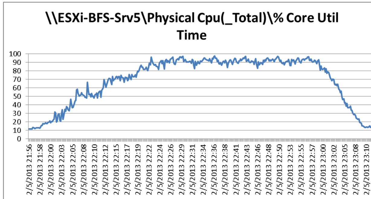
Figure 143 2000 User ESXi Host5 B200 M3 Processor Core Utilization Test Phase
