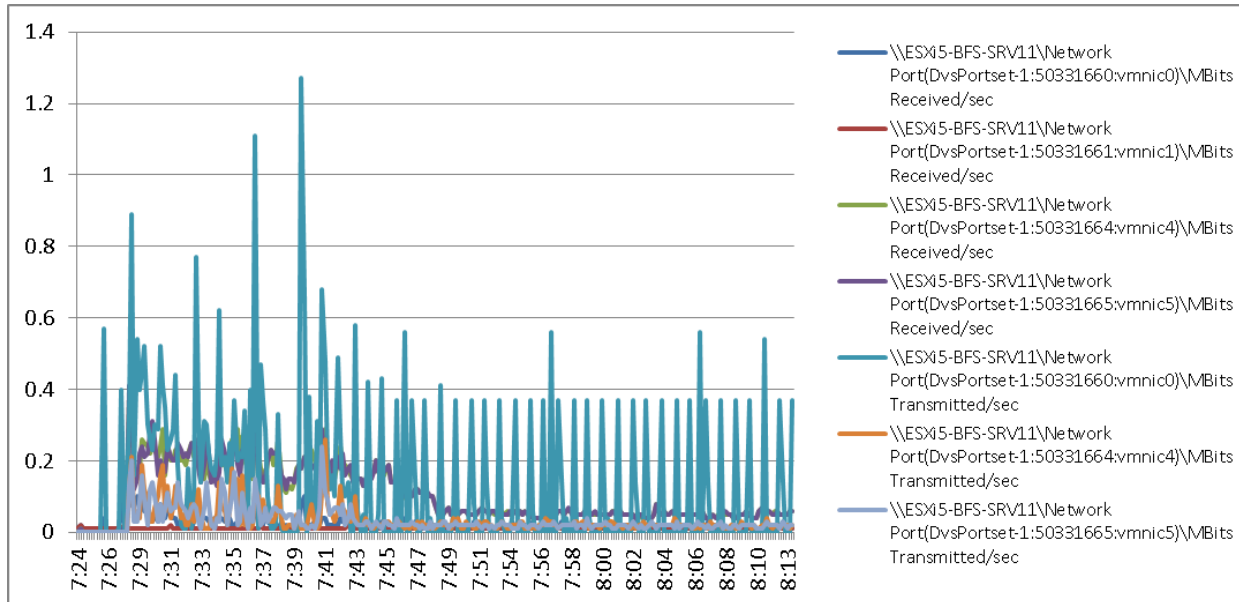
Figure 111 2000 User ESXi Host11 B200 M3 Cisco VIC1240 MLOM Network Adapter Mbps Receive/Transmit Boot Phase
