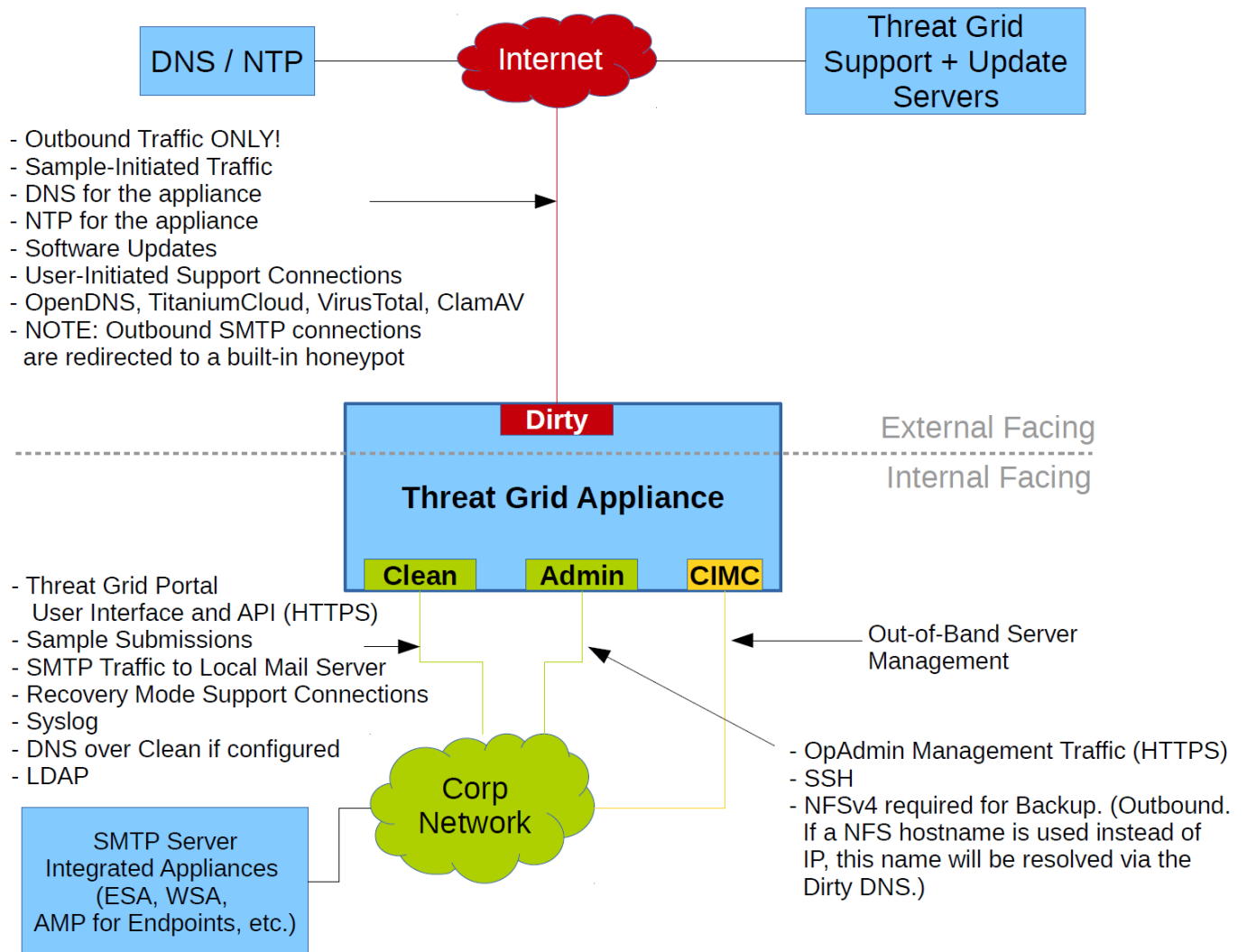
Figure 7 - Network Interfaces Setup Diagram
