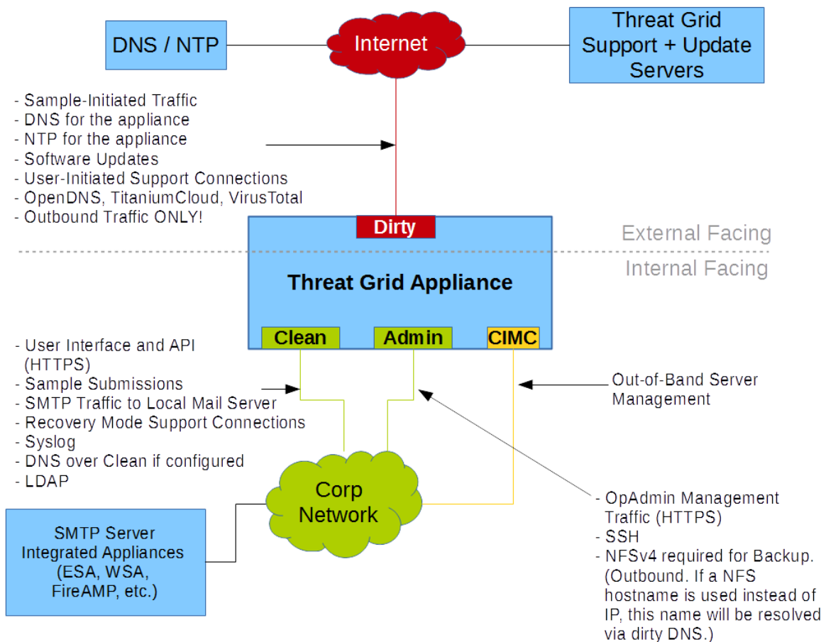
Figure 7 - Network Interfaces Setup Diagram
