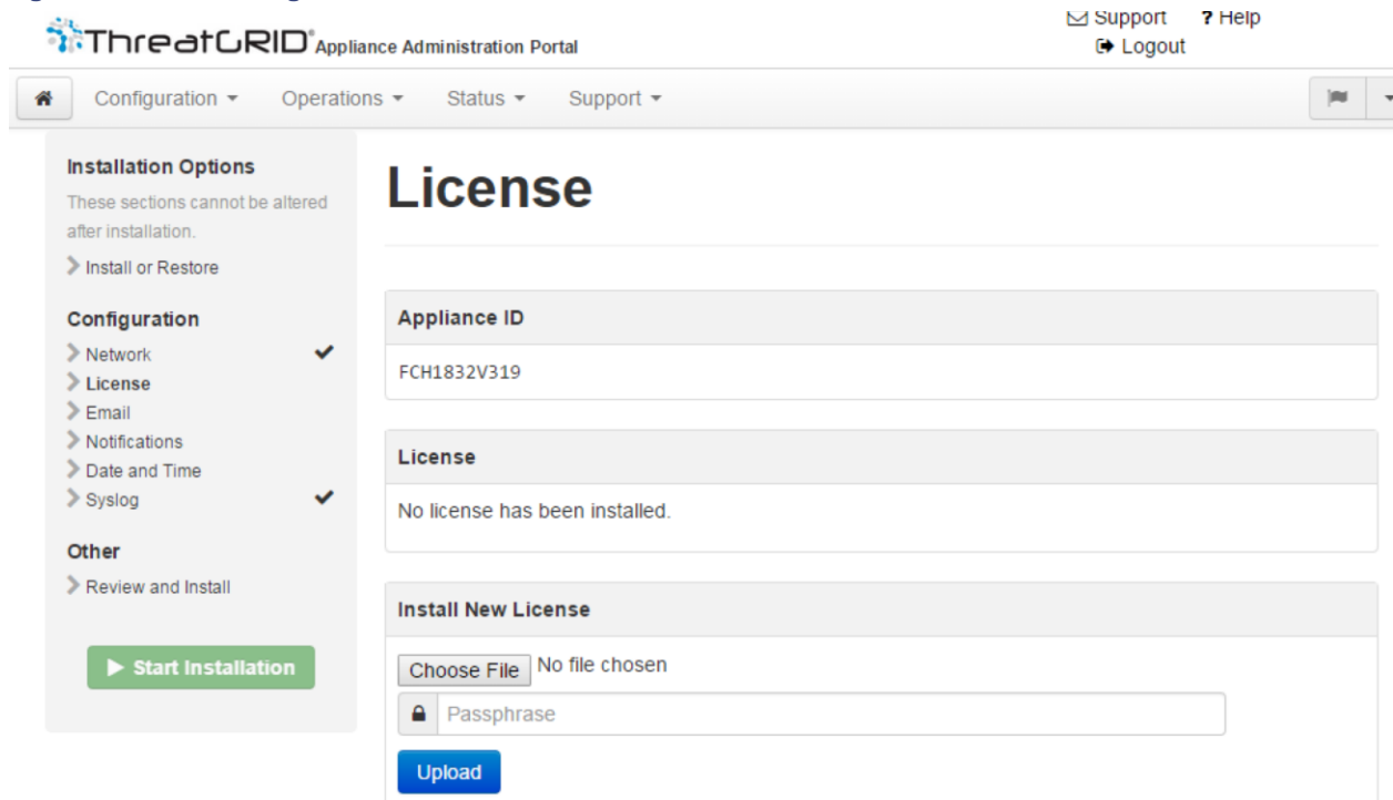
Figure 18 - License Page
