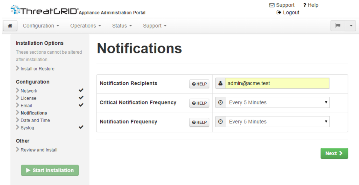
Figure 20 - Notifications Configuration
