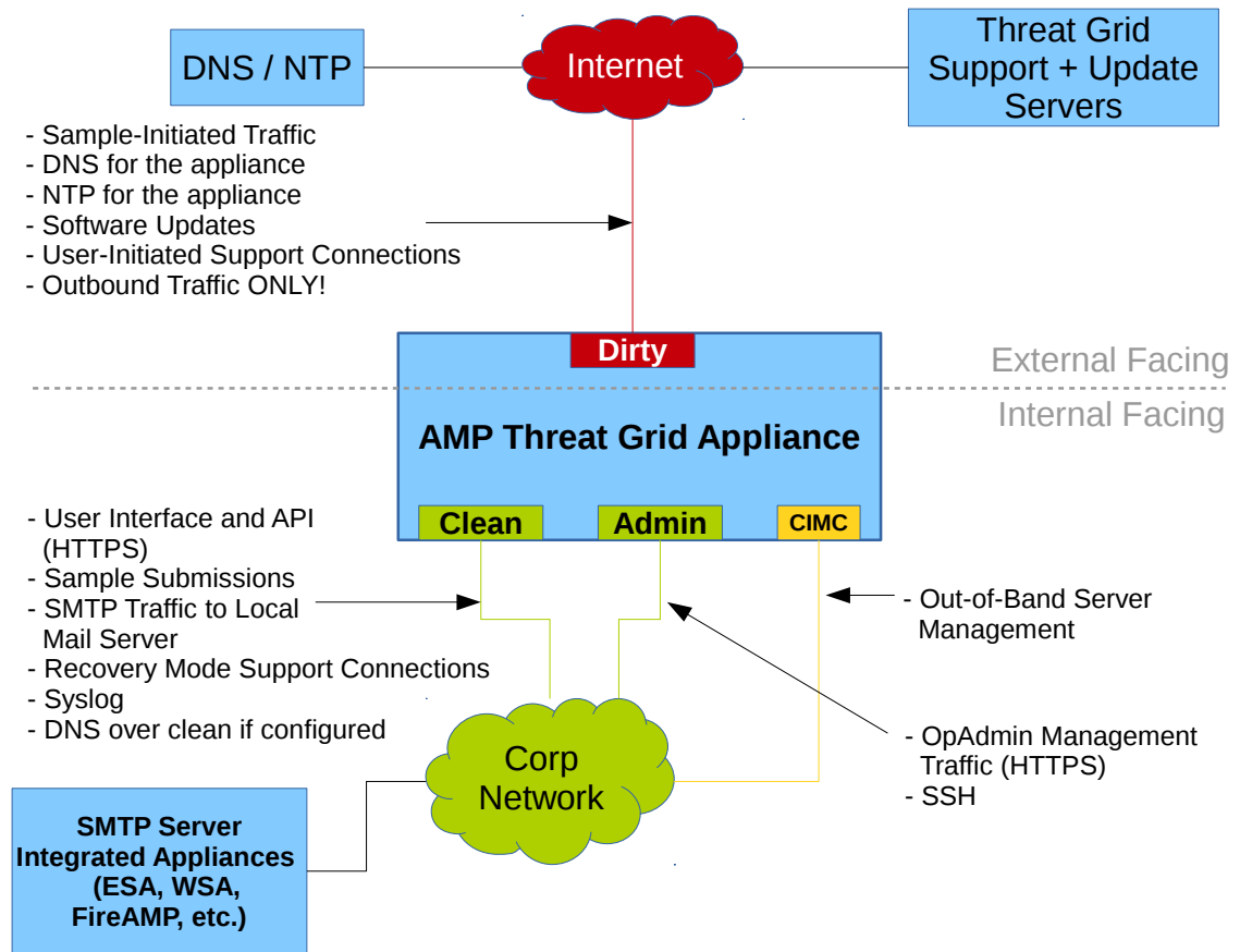
Figure 5 - Network Interfaces Setup Diagram
