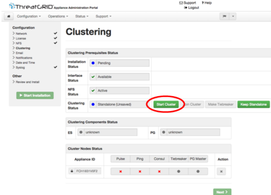
Figure 31 - Start Cluster
