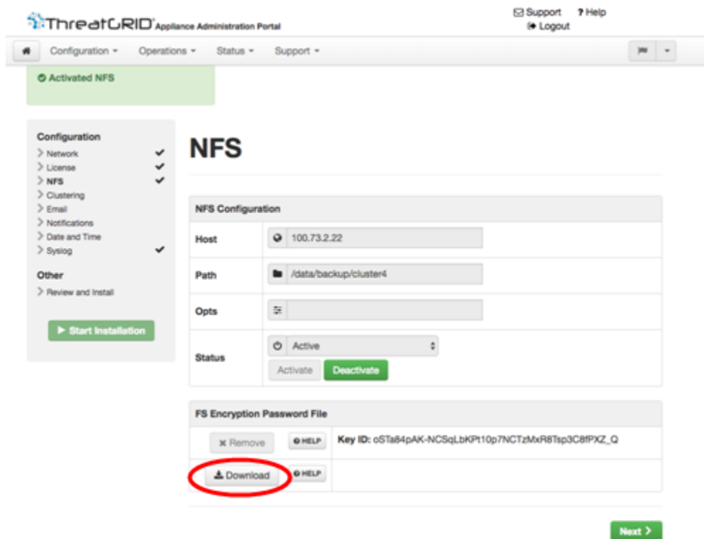
Figure 29 - NFS Active
