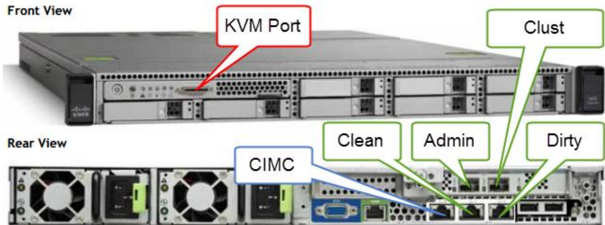
Figure 23 - Clust Interface Setup for Cisco UCS M3 C220
