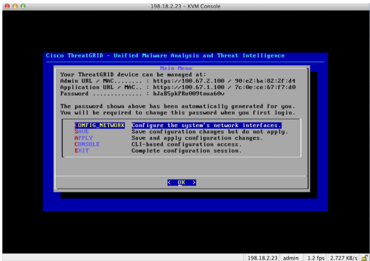
Figure 2 - TGSH Dialog
