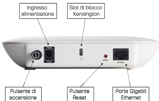
Figura 3. Pannello posteriore di Cisco WAP321 Wireless-N Selectable-Band Access Point with Single Point Setup
