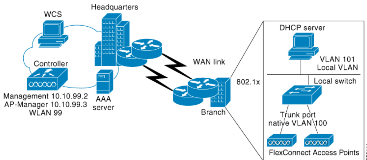
Figure 16: FlexConnect Deployment
