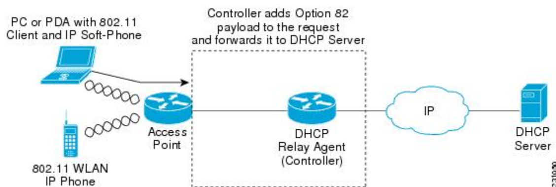
Figure 52: DHCP Option 82
