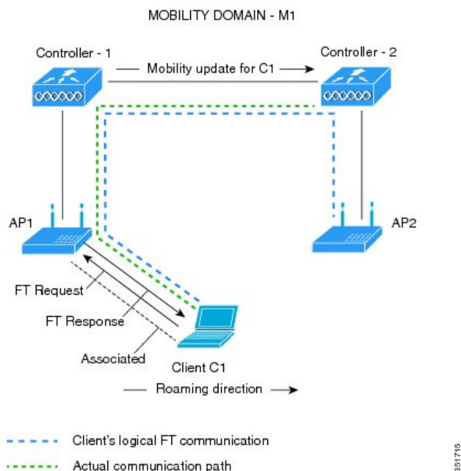
Figure 58: Message Exchanges when Over-the-DS Client Roaming is Configured
