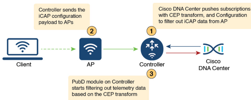
Figure 24: High-Level End-to-End System Flow for Cisco Catalyst Center Client Event and SSID Telemetry Filter
