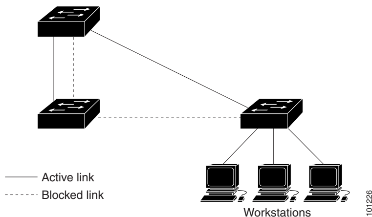
Figure 17-3 Spanning Tree and Redundant Connectivity
