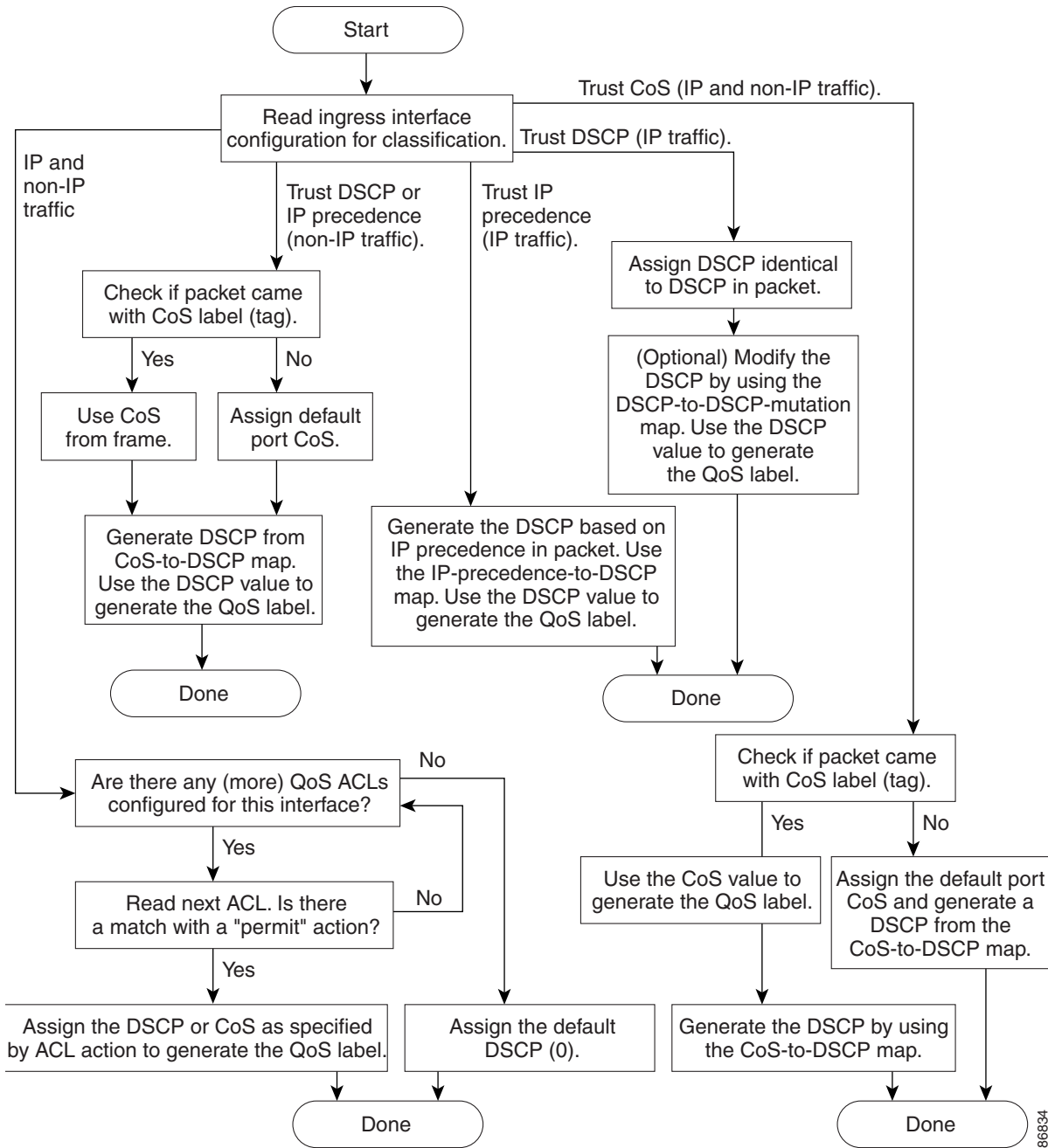
Figure 35-3 Classification Flowchart
