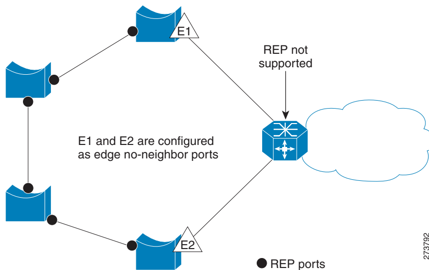
Figure 20-3 Edge No-Neighbor Ports
