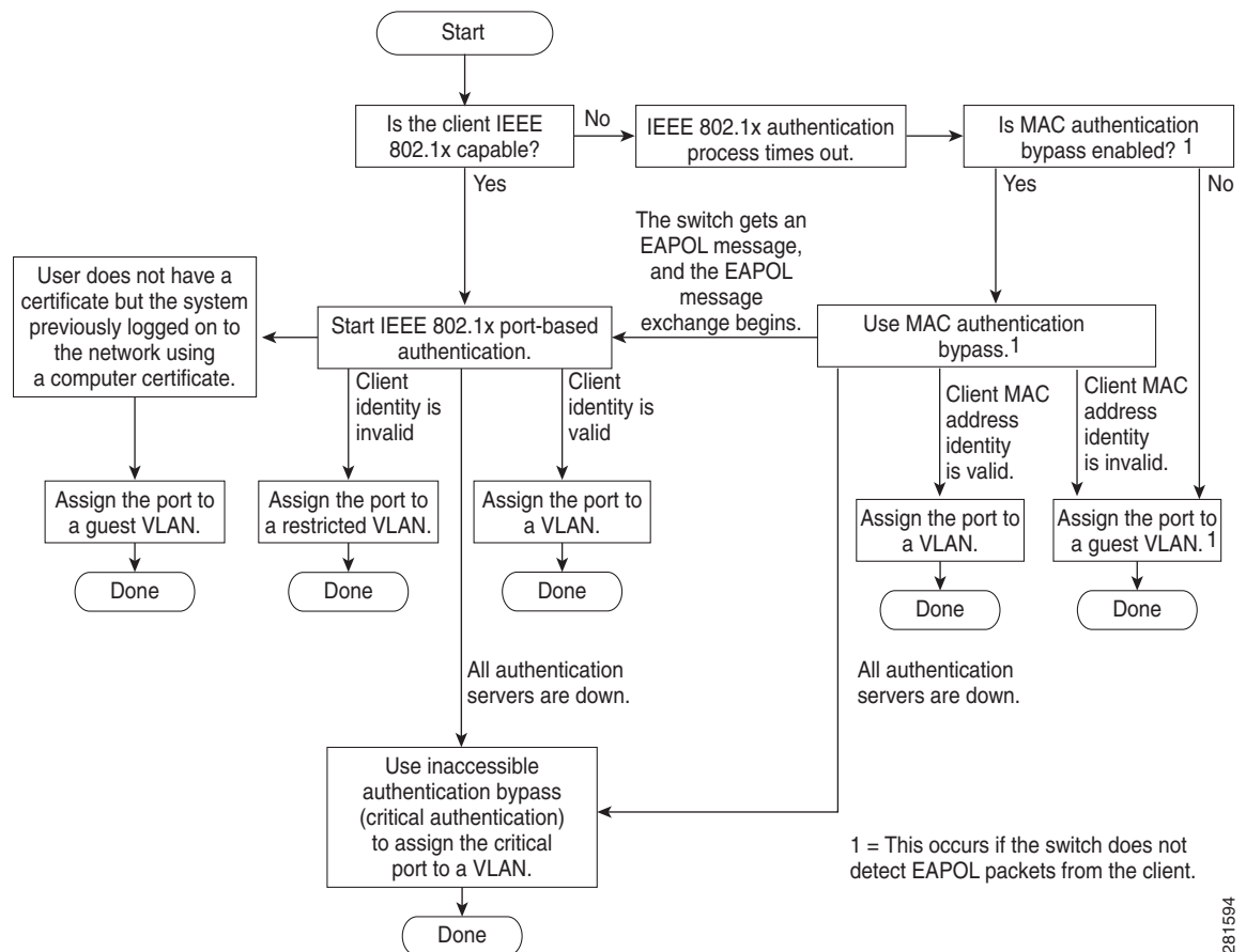
Figure 10-2 Authentication Flowchart
