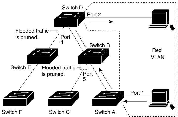
Figure 15-2 Optimized Flooded Traffic with VTP Pruning
