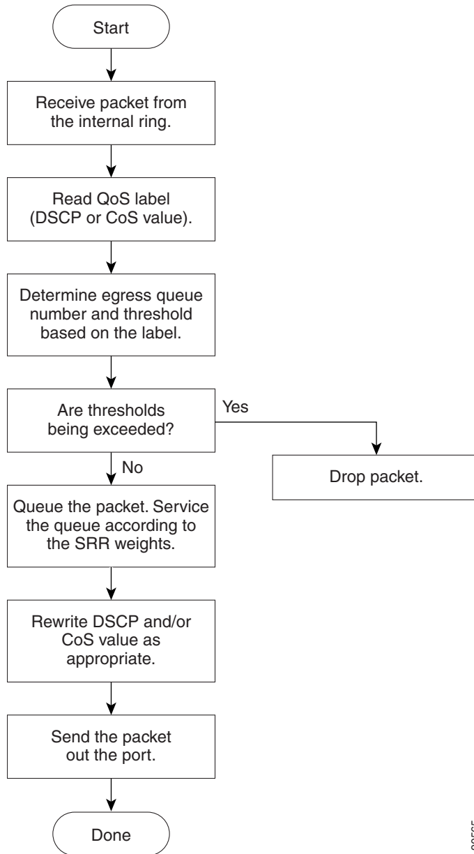
Figure 38-8 Queueing and Scheduling Flowchart for Egress Ports
