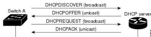
Figure 111: DHCP Client and Server Message Exchange
