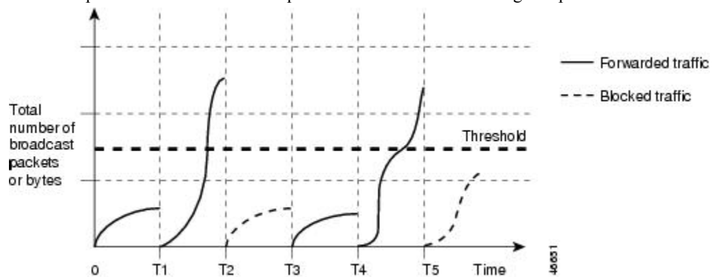
Figure 103: Broadcast Storm Control Example
