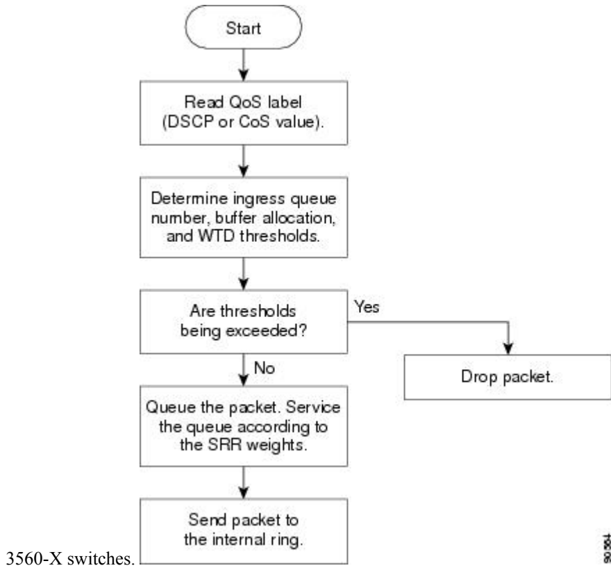
Figure 60: Queueing and Scheduling Flowchart for Ingress Ports on Catalyst 3560-E and 3560-X Switches
