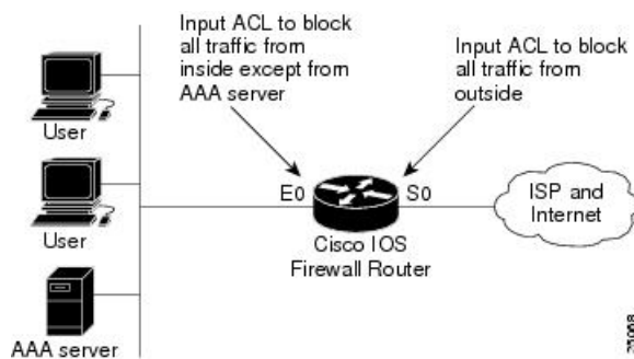
Figure 96: Applying the Authentication Proxy at the Local Interface
