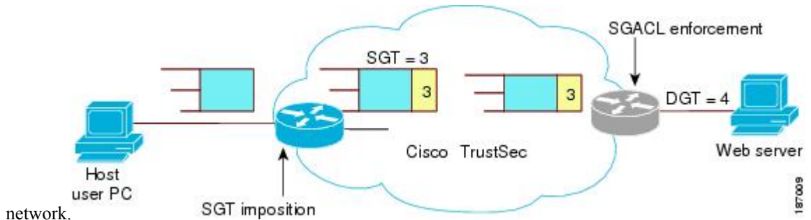
Figure 9: SGT and SGACL in Cisco TrustSec Network
