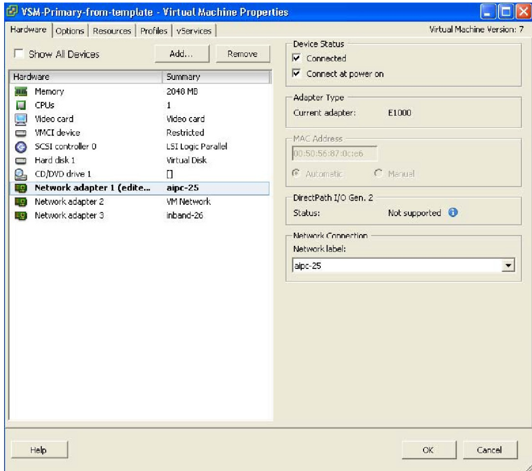
Figure 20: Virtual Machine Properties Window
