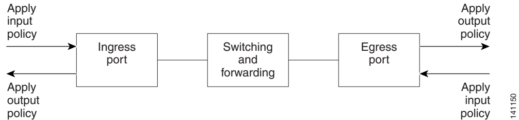
Figure 2-2 Input and Output Policy Relationship
