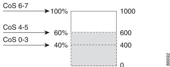
Figure 2-7 WTD and Queue Operation
