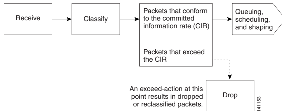
Figure 2-5 Policing of Classified Packets
