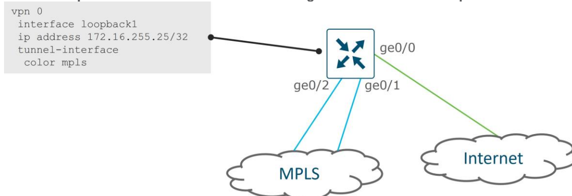
Figure 67. Loopback interface tunnel use case: scaling traffic to the same transport
