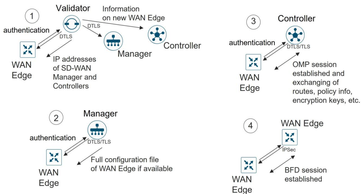
Figure 19. Bringing a WAN Edge into the overlay
