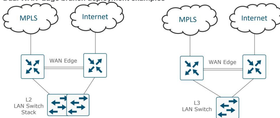
Figure 77. Dual WAN-Edge branch deployment examples
