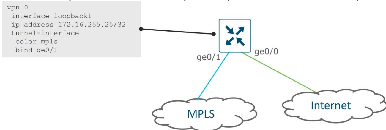
Figure 66. Loopback interface tunnel use case: provider IP space cannot be used for a tunnel endpoint
