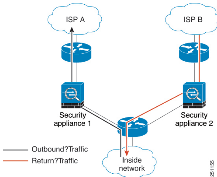
Figure 39: Asymmetric Routing
