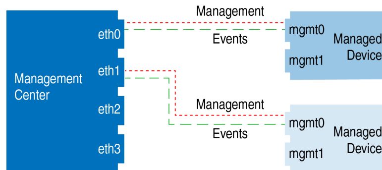
Figure 43: Multiple Management Interfaces on the Firepower Management Center
