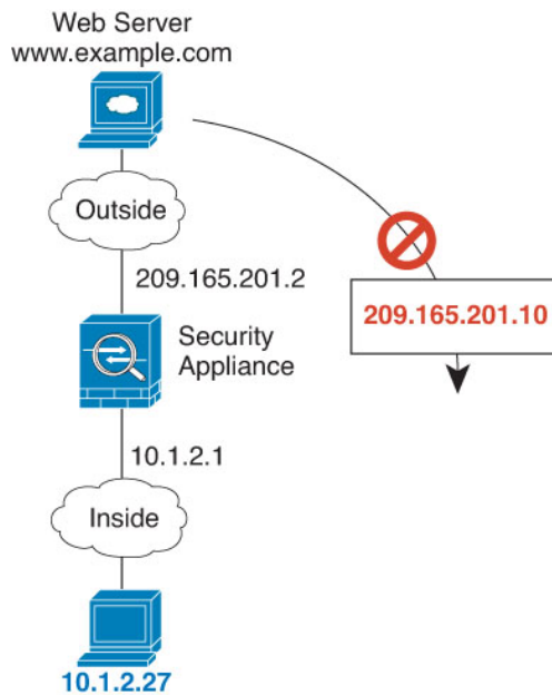
Figure 50: Remote Host Attempts to Initiate a Connection to a Mapped Address
