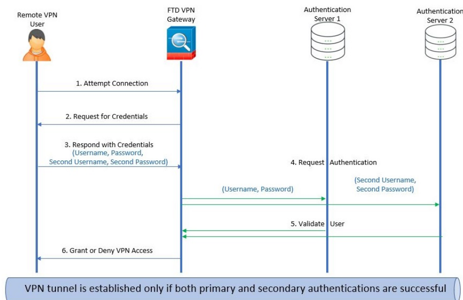
Figure 38: Remote Access VPN Secondary or Double Authentication
