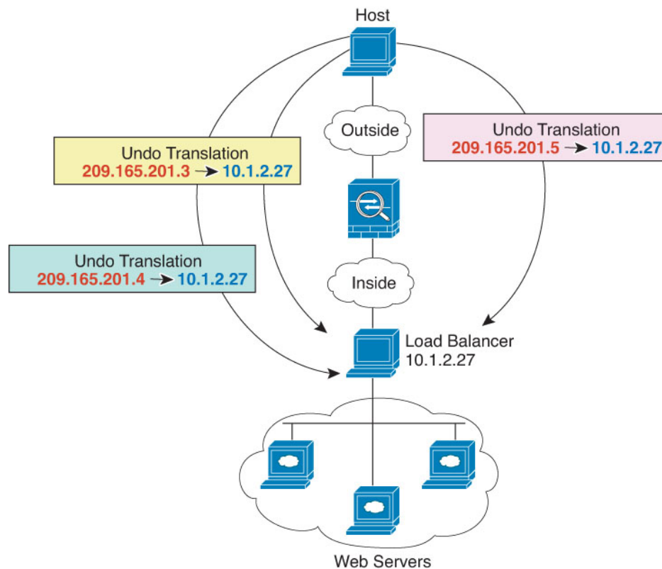
Figure 55: One-to-Many Static NAT Example
