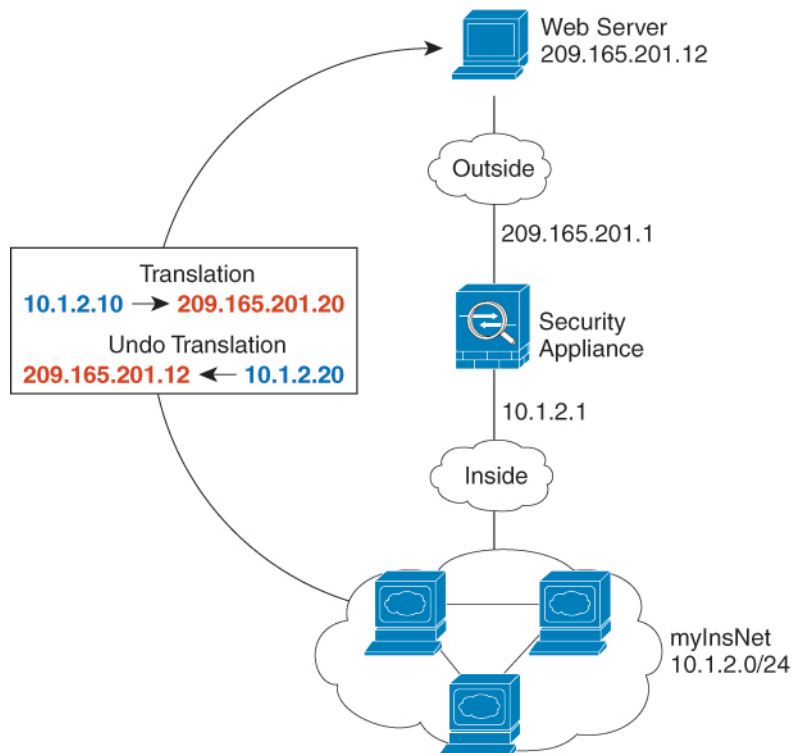
Figure 60: Dynamic NAT for Inside, Static NAT for Outside Web Server
