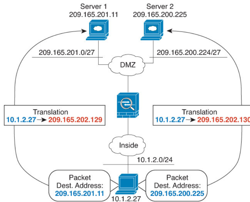
Figure 63: Manual NAT with Different Destination Addresses
