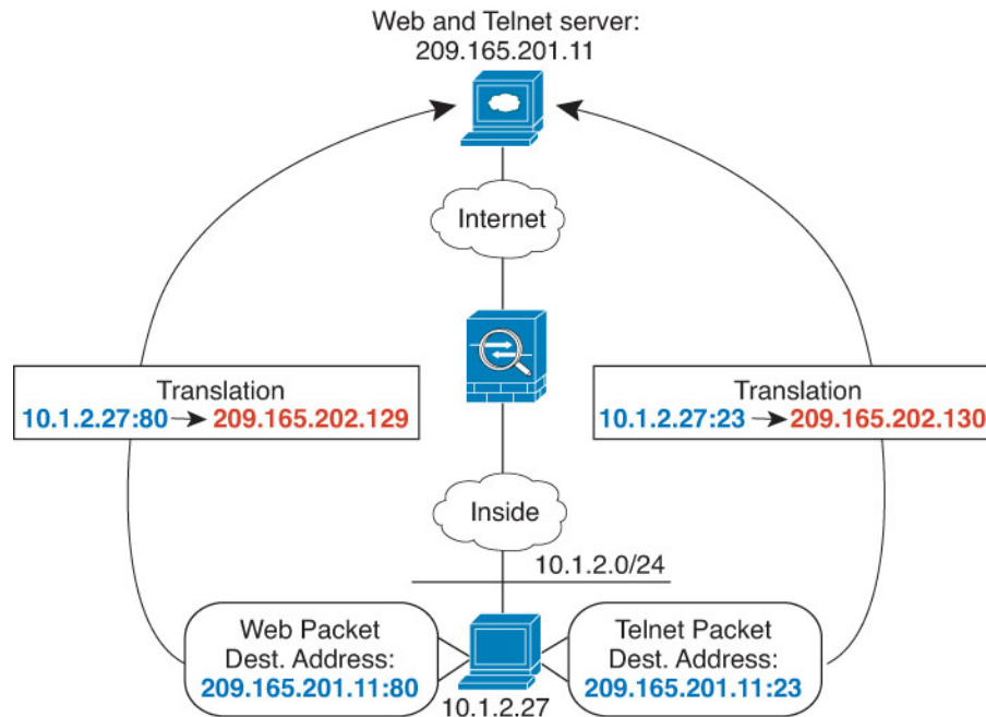
Figure 64: Manual NAT with Different Destination Ports
