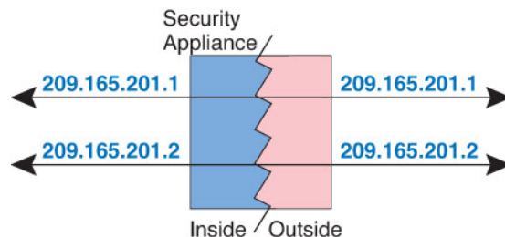
Figure 58: Identity NAT
