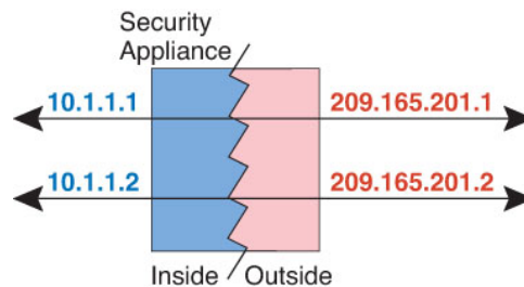
Figure 52: Static NAT
