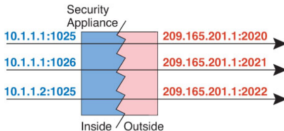
Figure 51: Dynamic PAT
