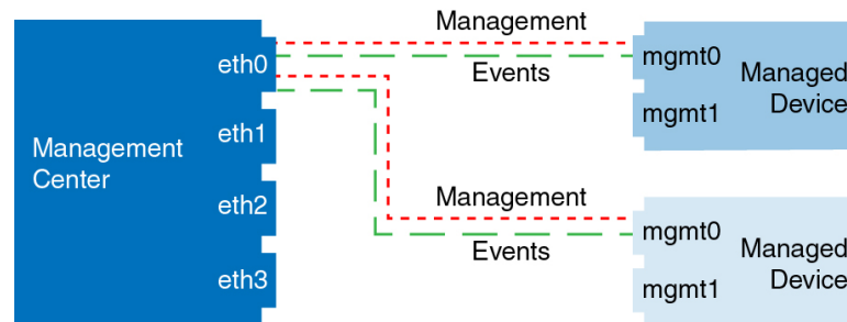
Figure 42: Single Management Interface on the Firepower Management Center
