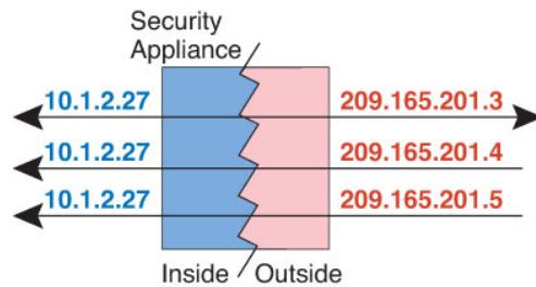
Figure 54: One-to-Many Static NAT
