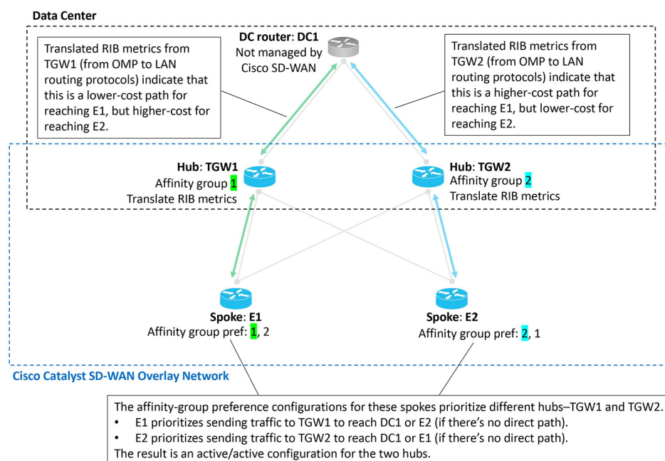
Figure 46: Data Center, Two Hubs, Active/Active
