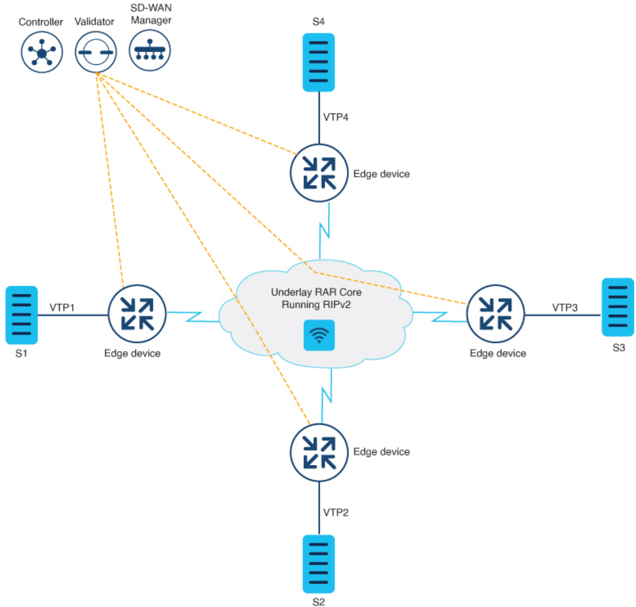
Figure 8: RAR Architecture
