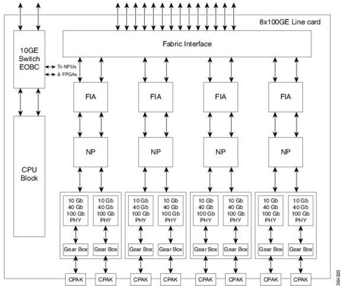
Figure 49: Major Components in the Cisco ASR 9000 Series Routers Line Cards
