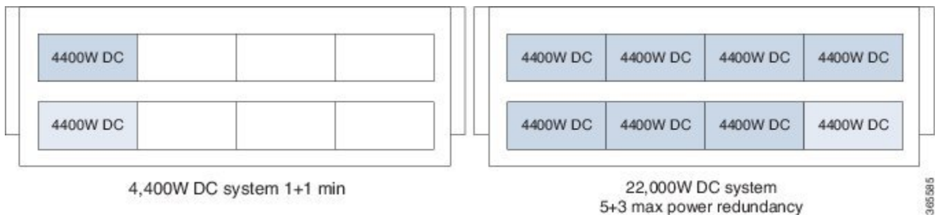
Figure 109: DC System Power Redundancy for the Cisco ASR 9910 Router—Version 3
