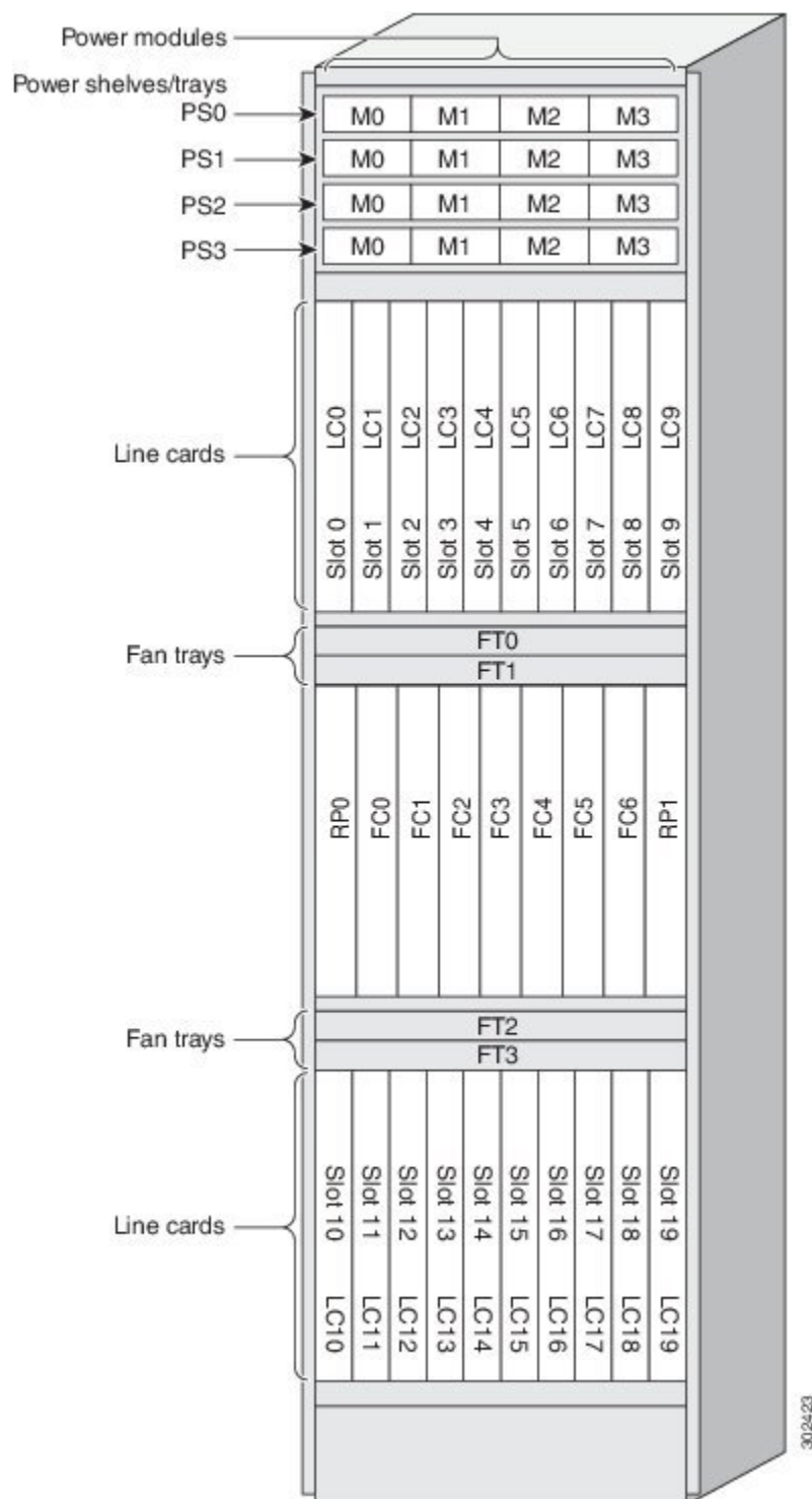
Figure 24: Cisco ASR 9922 Router Slot Numbering
