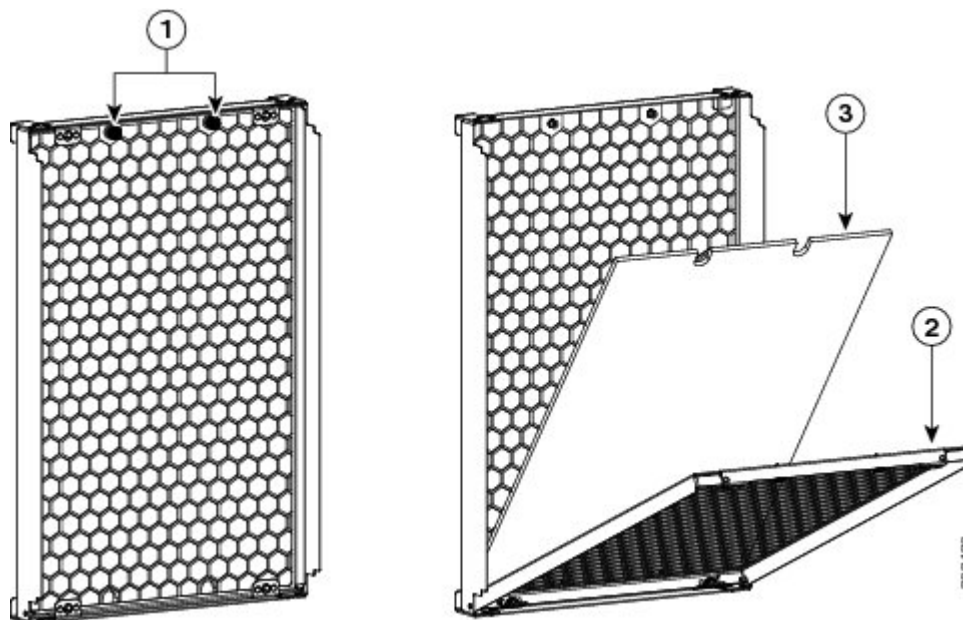
Figure 89: Cisco ASR 9922 Router Chassis Center Air Filter —Version 1
