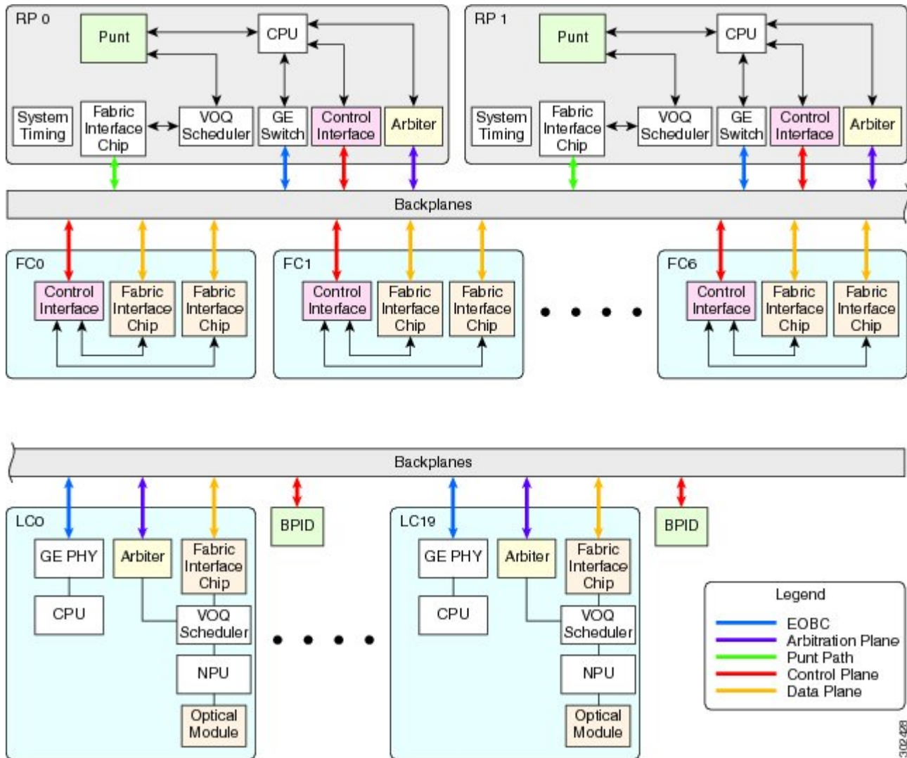
Figure 51: Major System Components and Interconnections in the Cisco ASR 9922 Router
