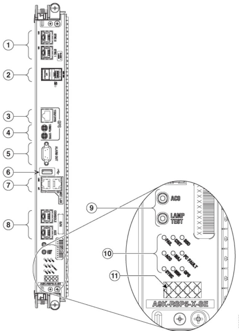
Figure 32: RSP5-X Card Front Panel
