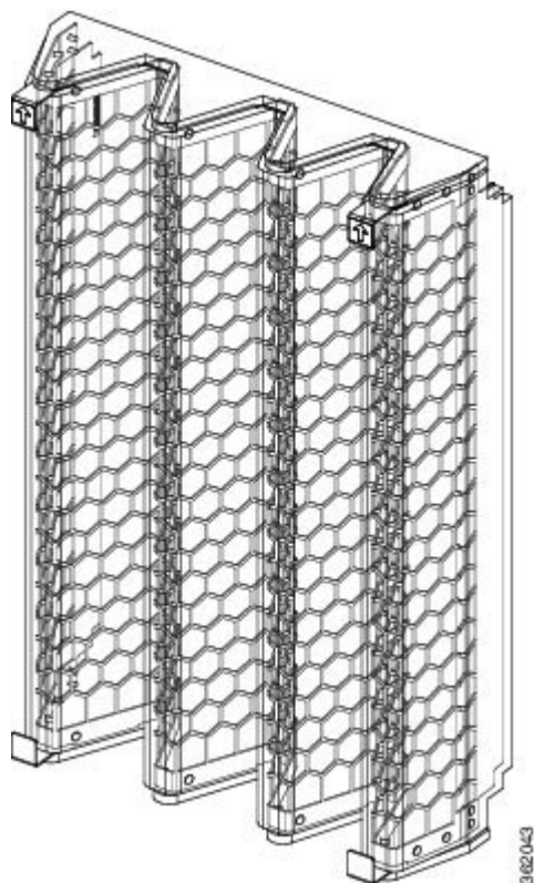
Figure 89: Cisco ASR 9922 Router Chassis Center Air Filter —Version 1
