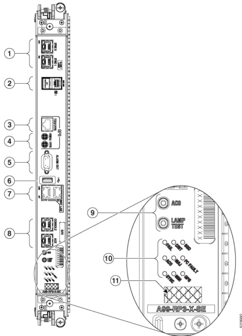
Figure 35: RP3-X Card Front Panel
