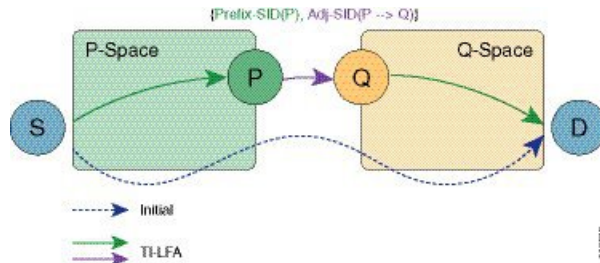
Figure 8: TI-LFA: { Prefix-SID(P) , Adj-SID (P -> Q) }
