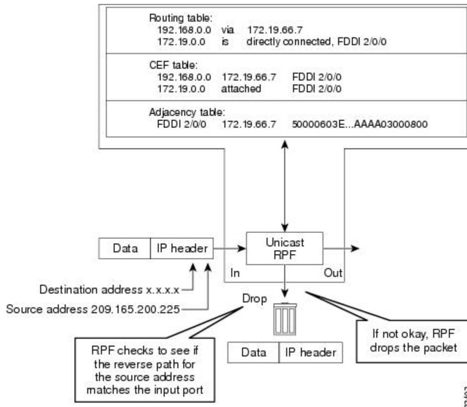
Figure 7: Unicast RPF Dropping Packets That Fail Verification
