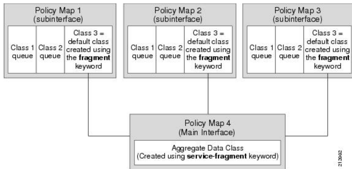
Figure 62: Physical Interface with Policy-Maps—Using Fragments
