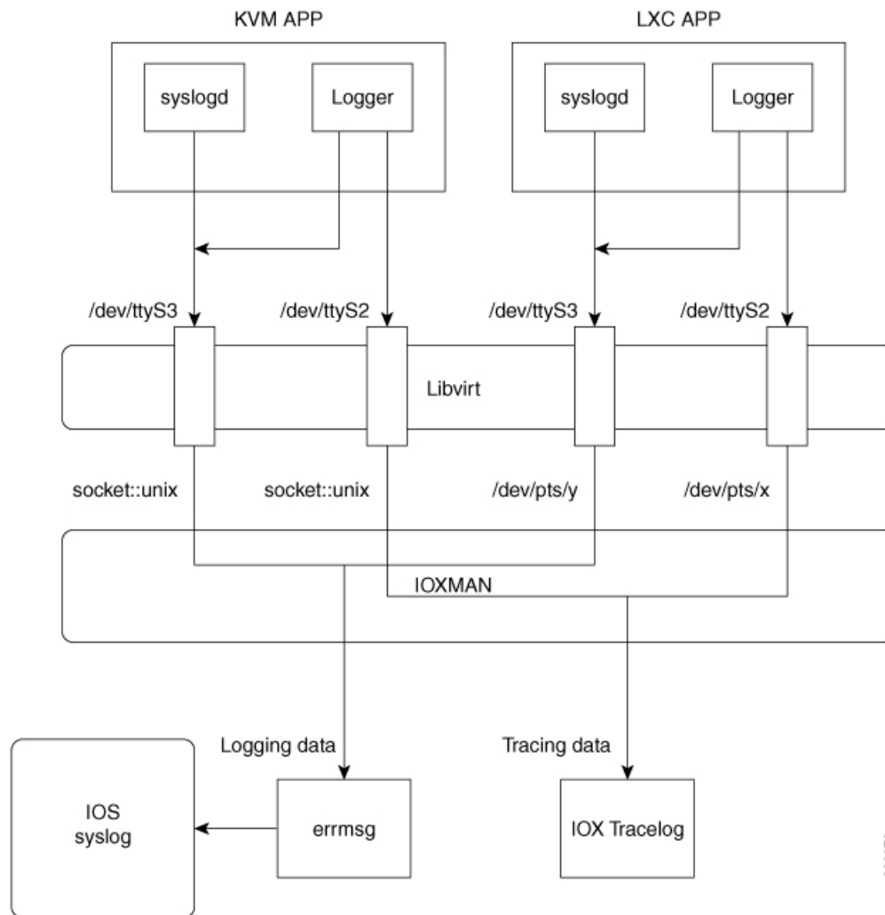
Figure 1: IOXMAN Structure
