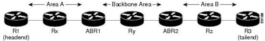
Figure 6: Multiarea Network
