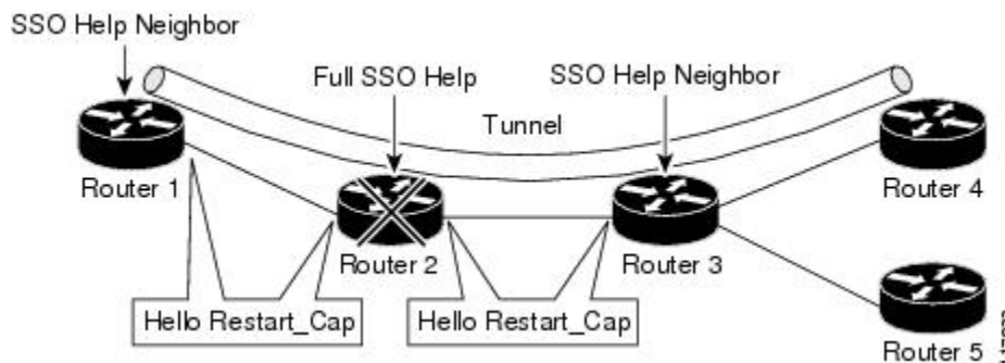
Figure 36: How Graceful Restart Works
