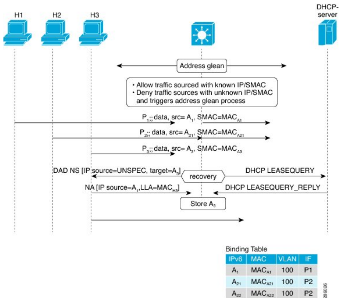
Figure 3: IPv6 Source Guard and Address Glean Overview
