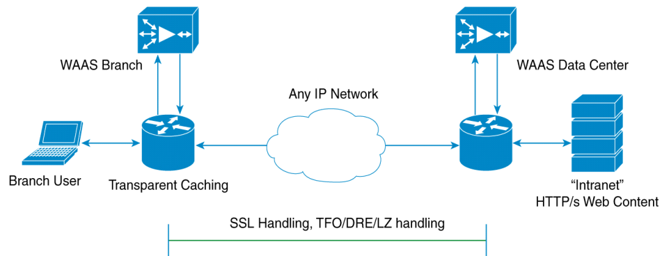
Figure 13-1 Dual-sided Deployment
