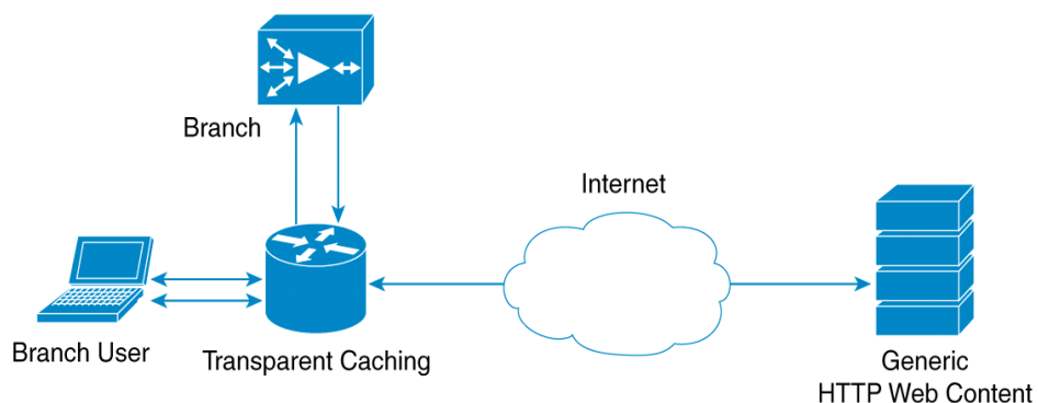
Figure 13-2 Single-sided Deployment
