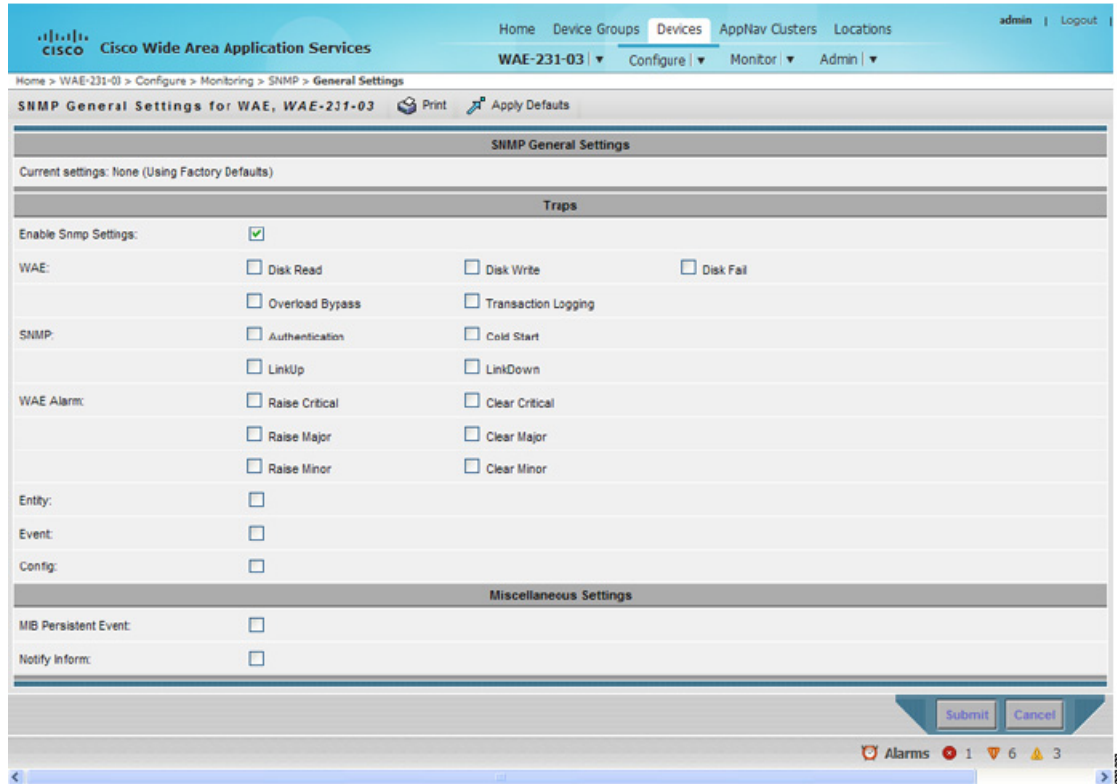
Figure 17-4 SNMP General Settings Window
