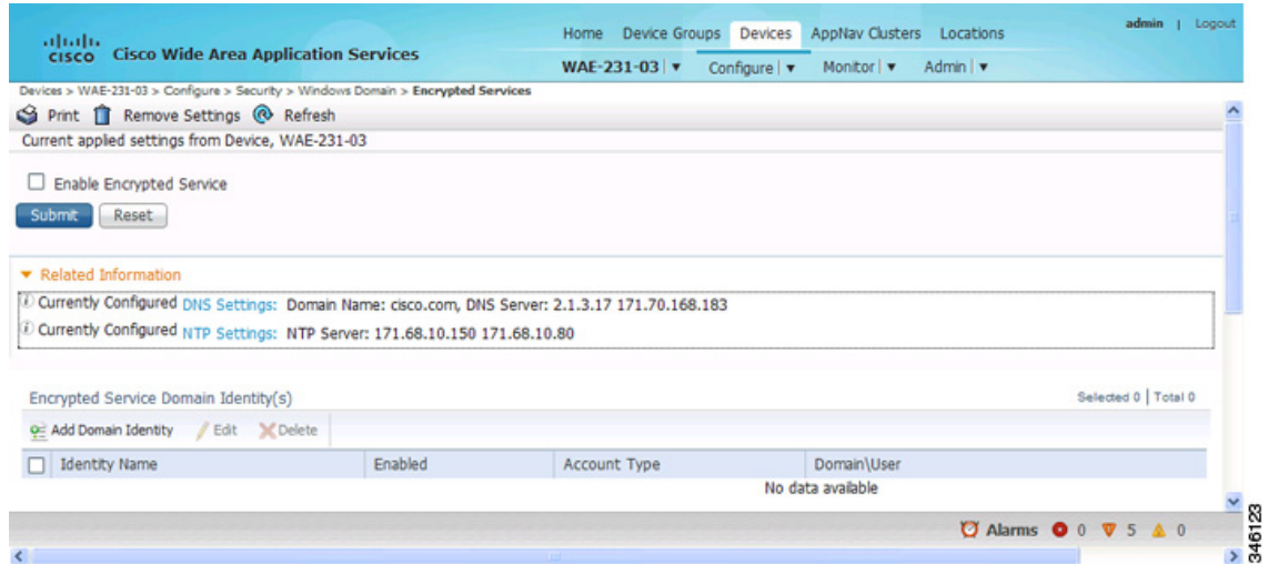
Figure 13-7 Encrypted Services
