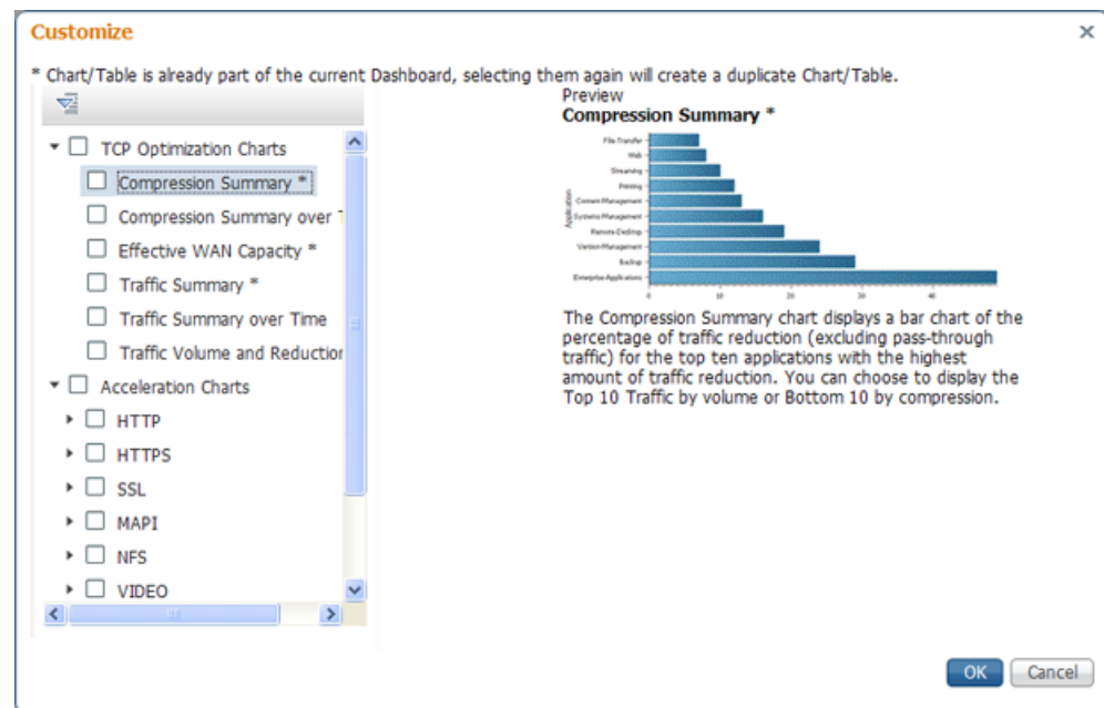
Figure 17-7 Customize Window
