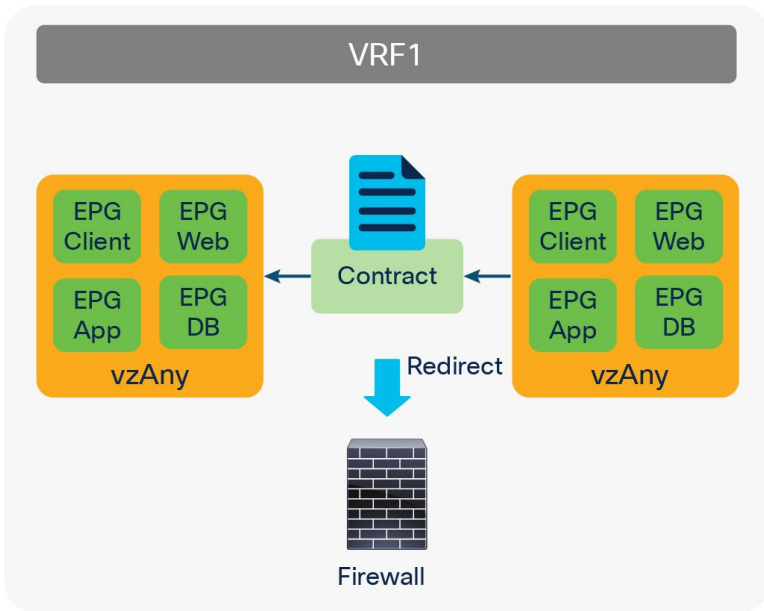
Figure 56. vzAny as consumer and provider (all EPGs to all EPGs use case)
