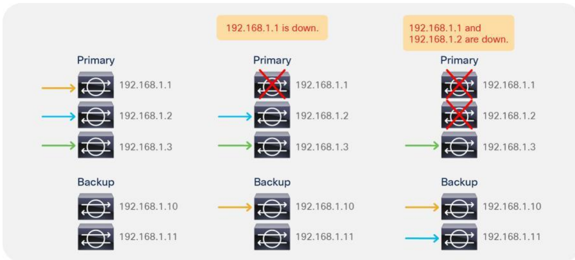
Figure 75. Multiple backup PBR nodes scenario
