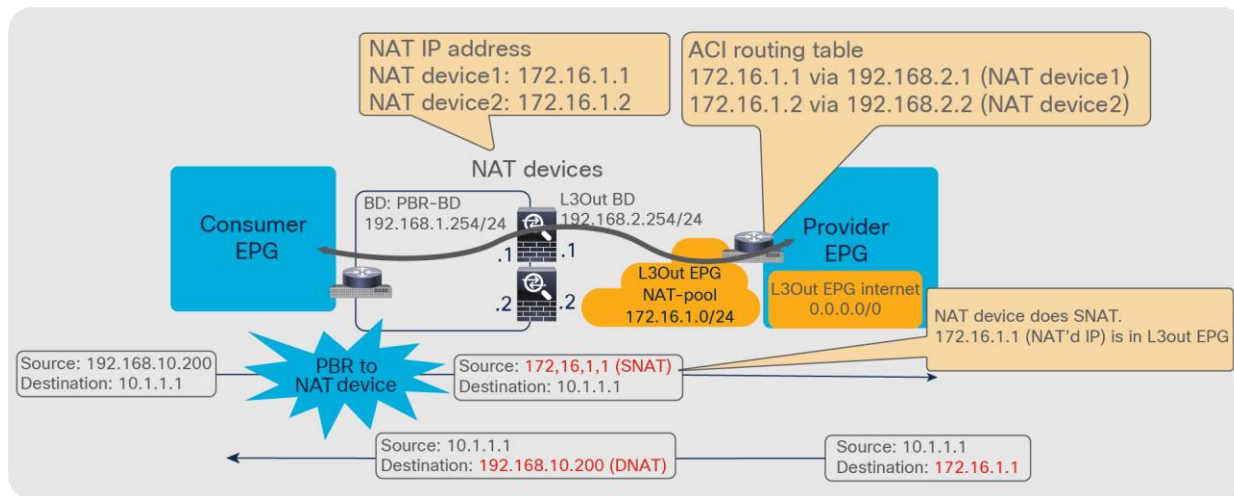
Figure 36. Design example of unidirectional PBR with the provider connector in a L3Out
