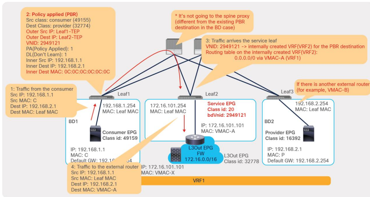
Figure 197. Traffic flow example: Consumer-to-provider traffic is redirected to the external router
