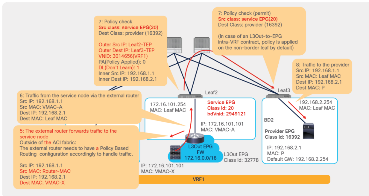
Figure 198. Traffic flow example: PBR node to the provider
