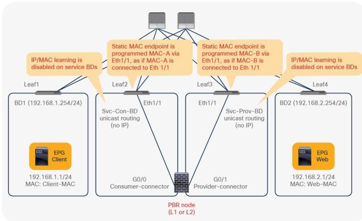
Figure 143. L1/L2 PBR topology example
