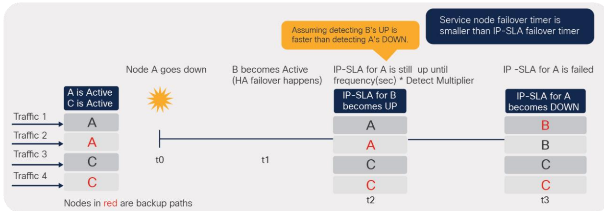
Figure 178. Example1: service node failover timer is smaller than IP-SLA failover timer (recommended)
