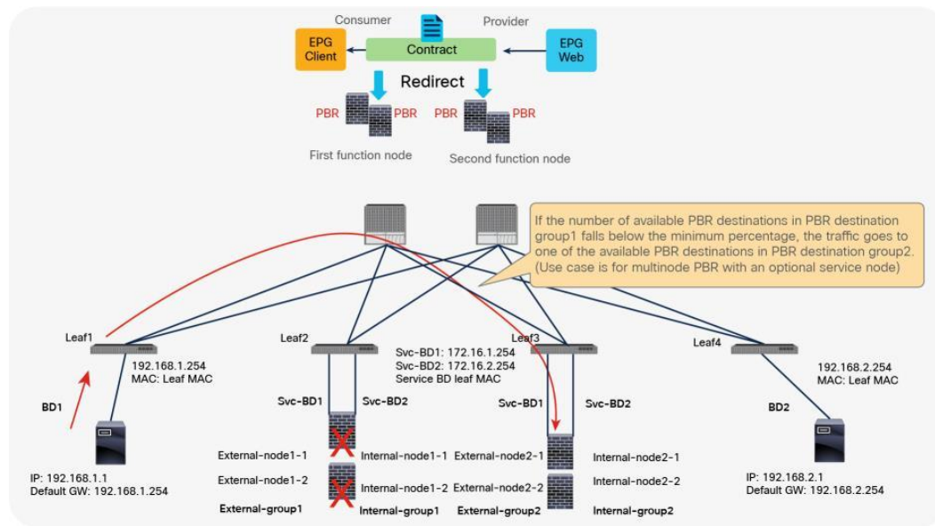
Figure 66. Down action Bypass
