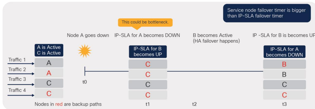
Figure 179. Example2: service node failover timer is bigger than IP-SLA failover timer (NOT recommended)
