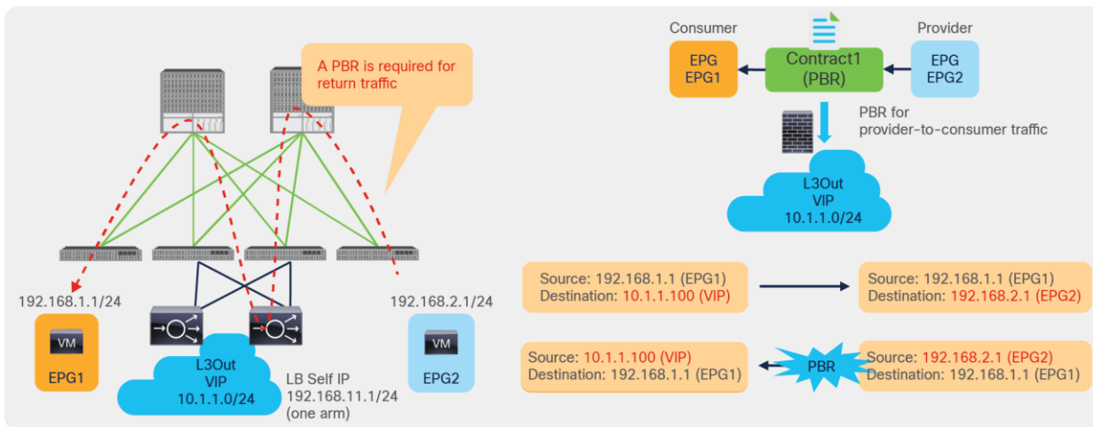
Figure 181. Use case example 2: Load balancer insertion
