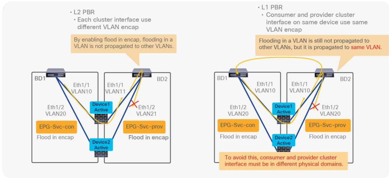
Figure 152. How to prevent loop for active/active L1/L2 PBR
