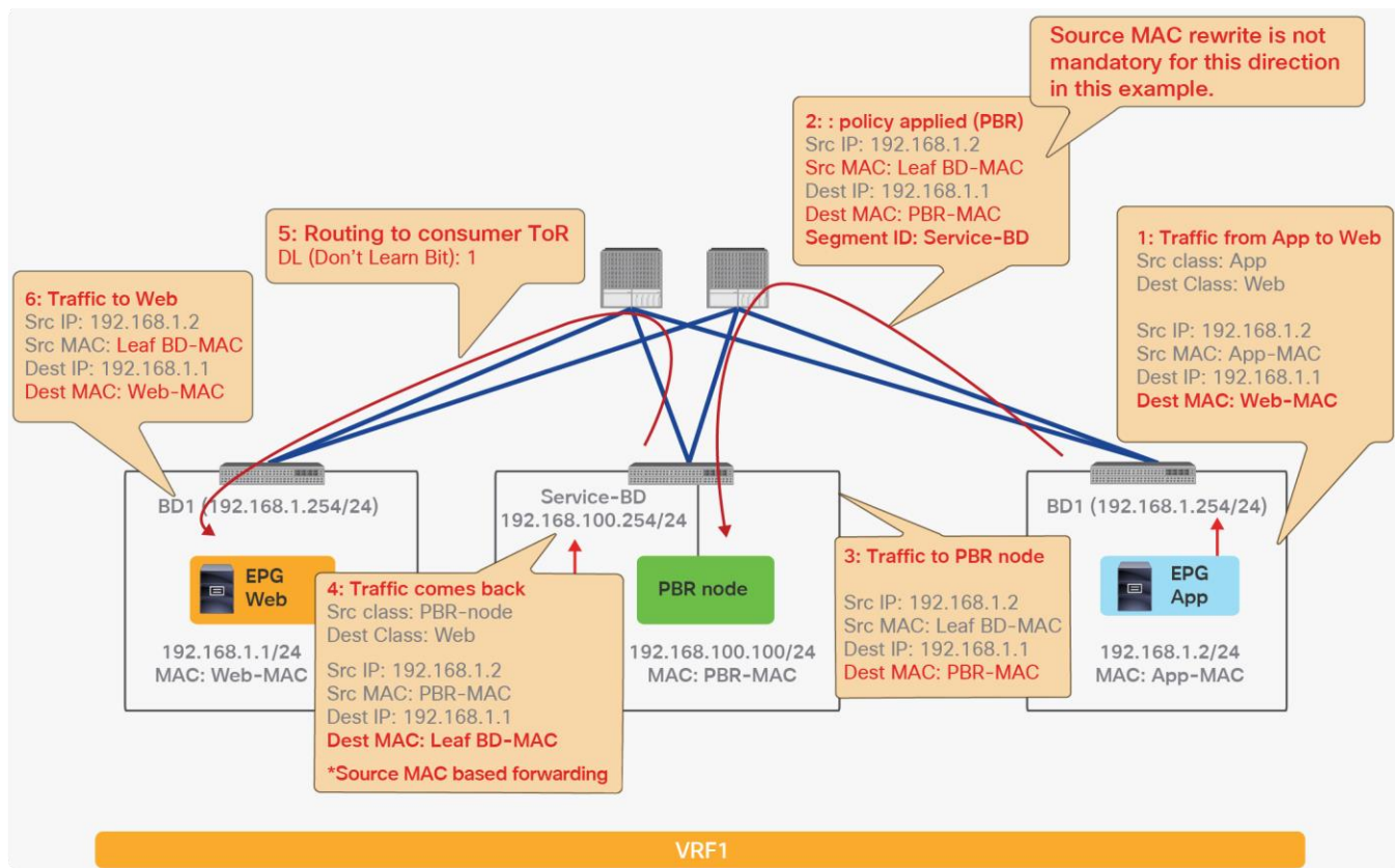
Figure 85. Rewrite source MAC packet walk (return traffic from provider to consumer traffic)
