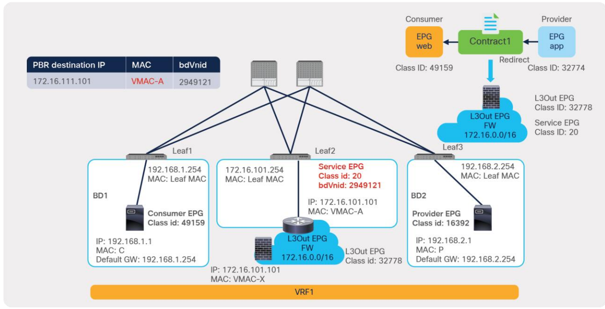
Figure 196. Traffic flow example: PBR destination IP is behind external routers
