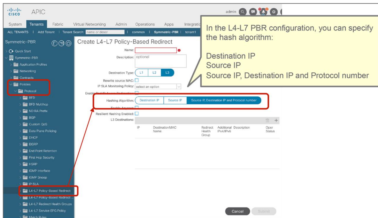
Figure 128. Hashing algorithm
