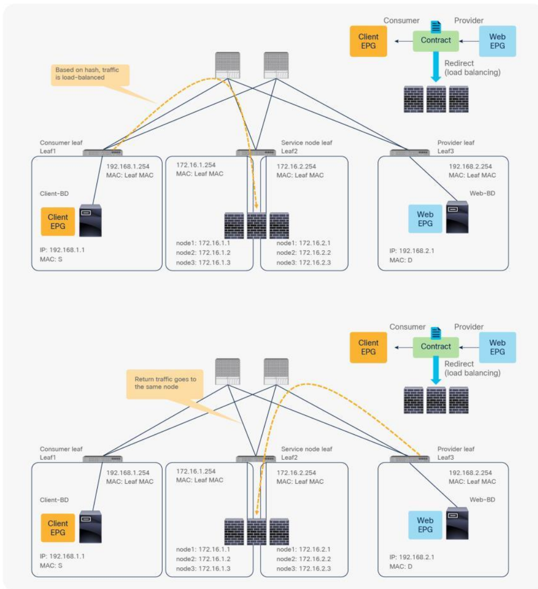
Figure 30. Symmetric PBR
