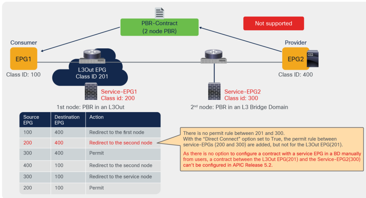
Figure 205. Multi-node service graph consideration: communication between nodes
