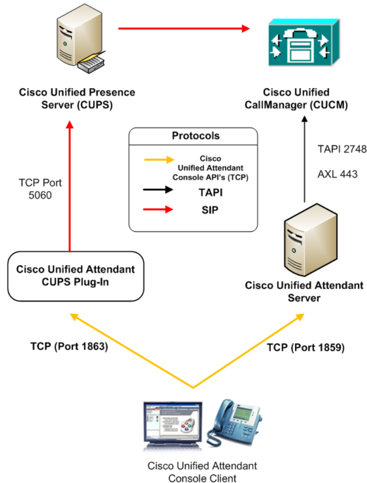
Figure 7-1 Cisco Unified Attendant Console Advanced Integration with CUPS
