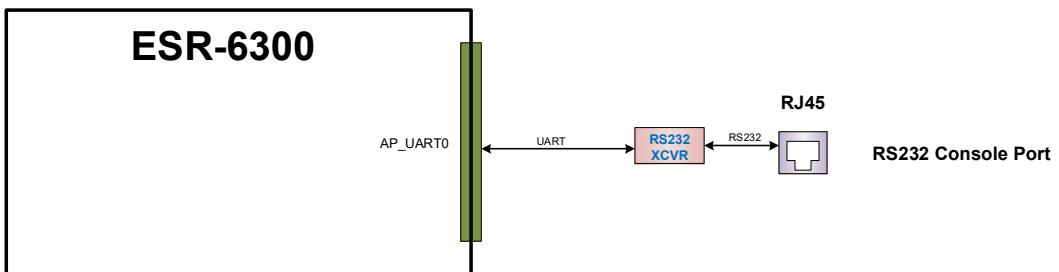
Option 2: RS232 Console Port
