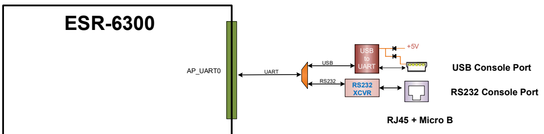
Option 3: RS232/USB Combo Console Port
