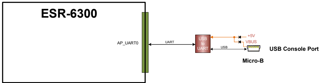
Option 1: USB Console Port
